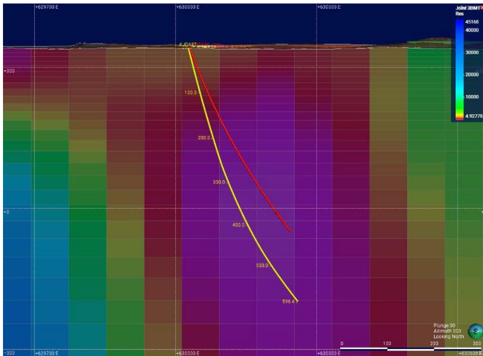
Figure 2. Kylie Prospect KJCD687 hole completed and the final hole planned in red and the integrated joint inversion model represents resistivity.
