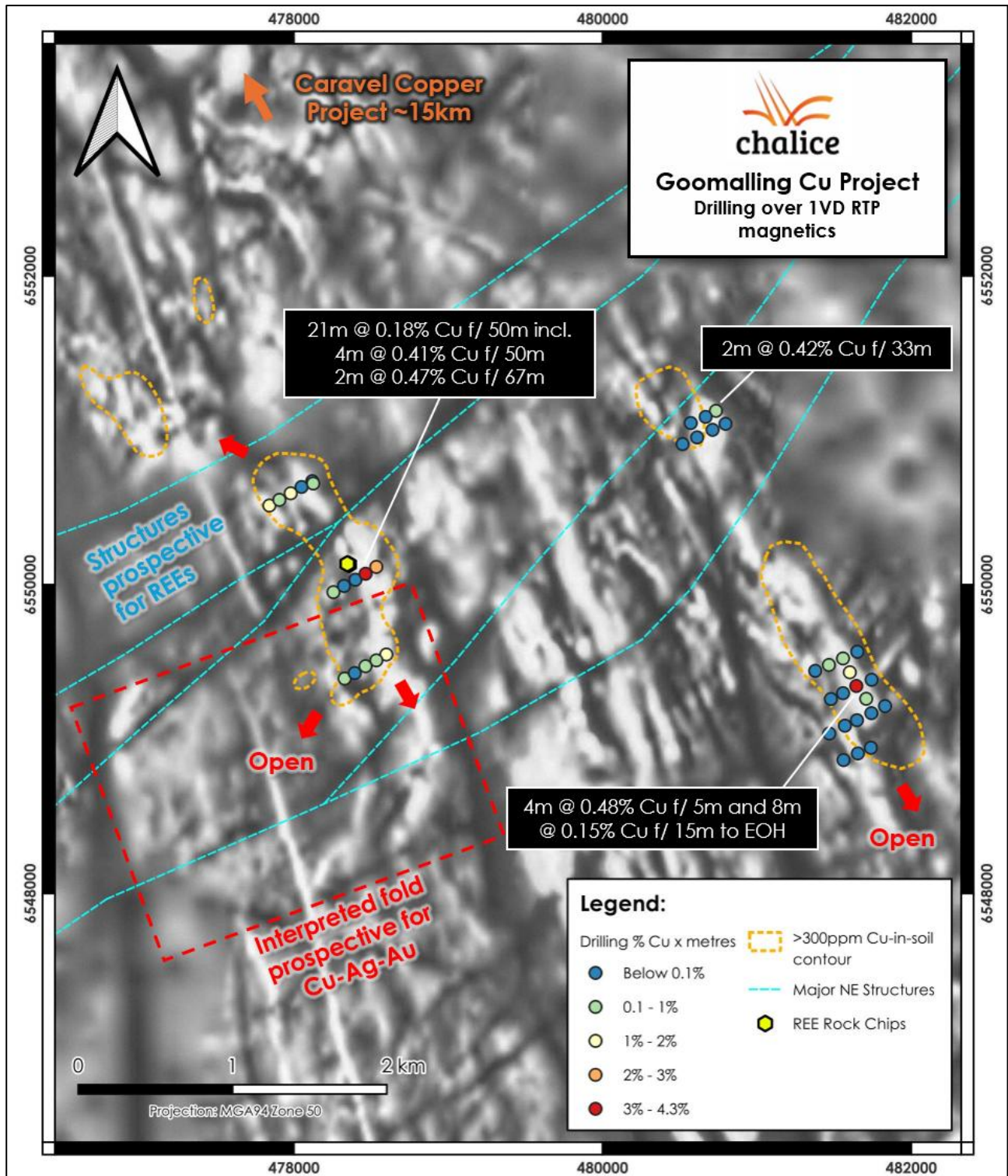
Figure 7. Goomalling Project drilling to date over 1VD magnetics.
