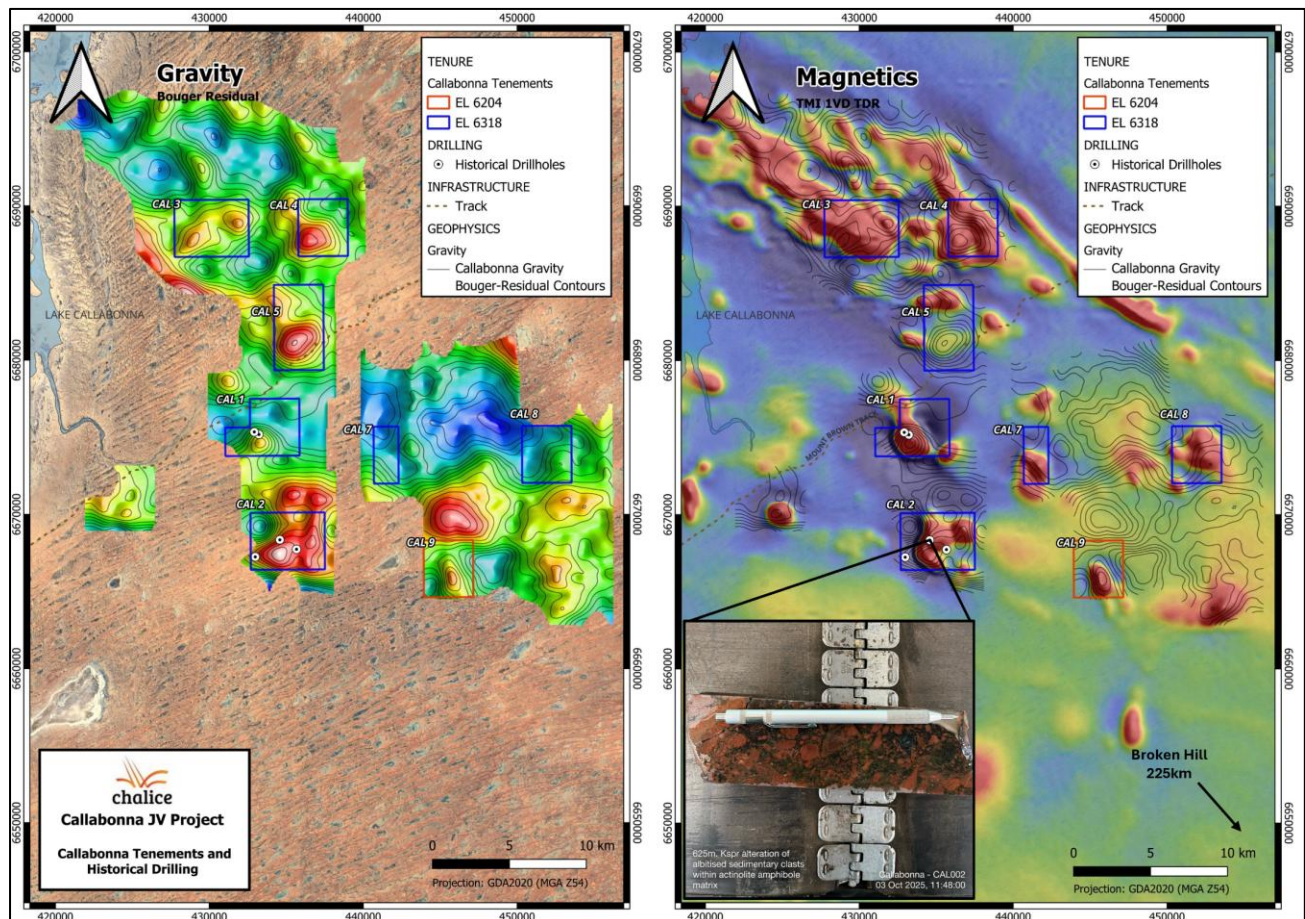
Figure 8. Callabonna residual gravity (LHS) and regional magnetics (TMI, RHS).
