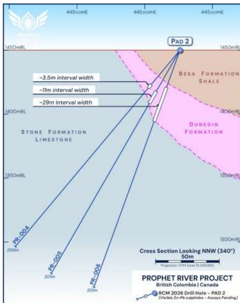
Figure 1: Cross-section through Pad 2 (looking 340°) showing the mineralised interval at the Dunedin/Stone Formation contact thickening with depth. Interval lengths from visual logging; true widths not yet known; assays pending.
