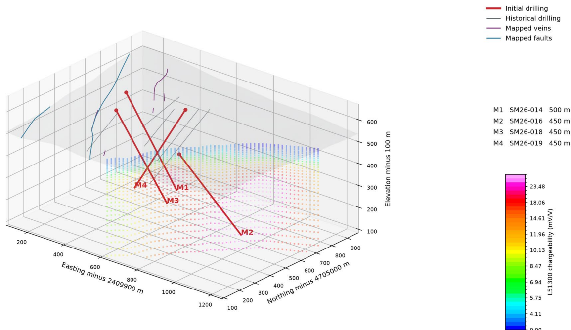
Figure 7 – Marcelina initial drill holes in 3D, showing mapped veins and faults, historical drilling and chargeability from 2026 IP line 51300.
