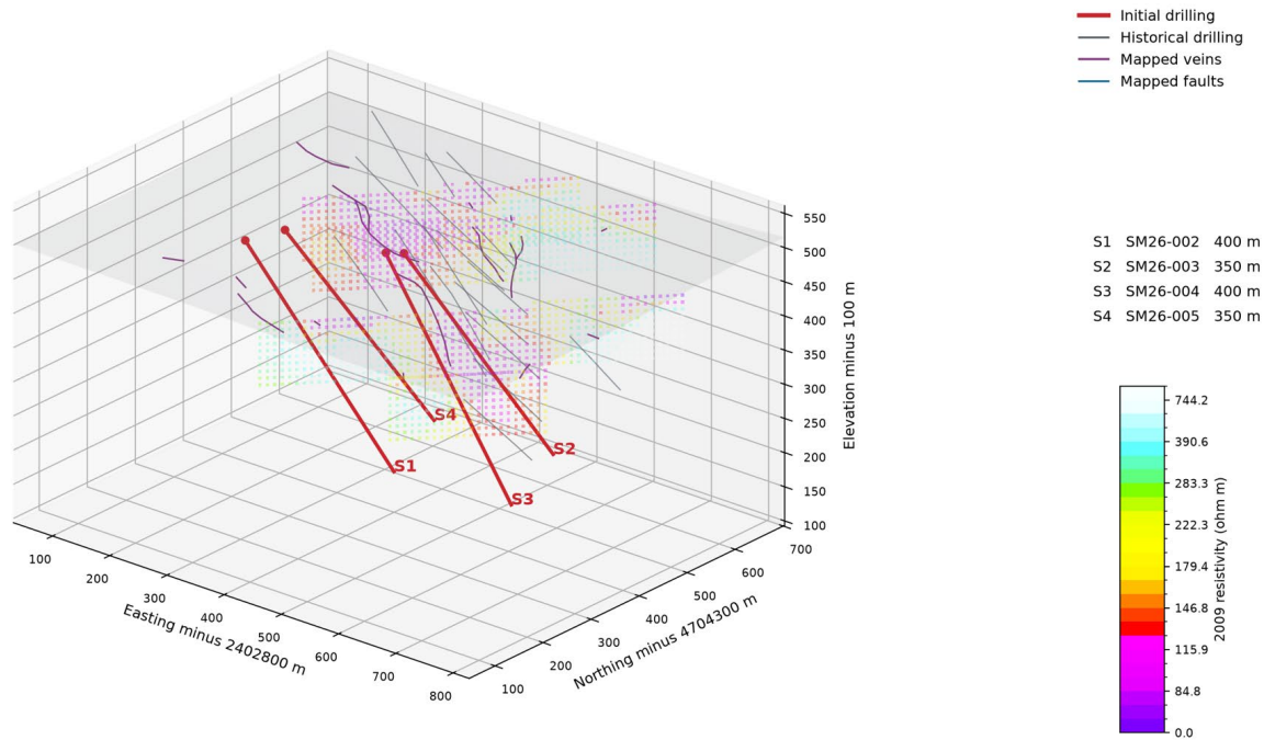
Figure 2 – Sascha initial drill holes in 3D, showing mapped veins, historical drilling and 2009 resistivity grid slices.
