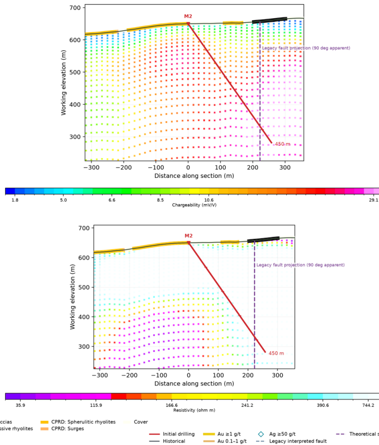
Figure 8 – Section SEC-11 showing SM26-016 (M2) drilled northeast across the interpreted Fault 2 and into the 2026 line 51300 chargeability (upper) and resistivity (lower) response.
