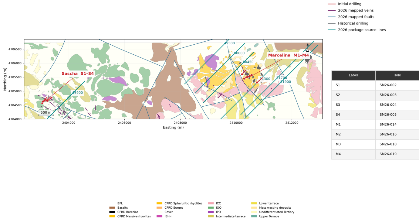
Figure 1 – Sascha Marcelina Project geology showing 2026 IP survey lines, 2026 mapped veins and faults, historical drilling and the initial drill holes at Sascha (S1 to S4) and Marcelina (M1 to M4).
