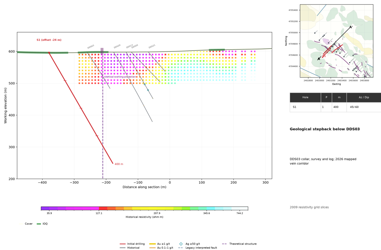
Figure 3 – Section SEC-01 showing SM26-002 (S1) as a geological step-back below historical hole DDS03, with 2009 resistivity and historical gold and silver intercepts.
