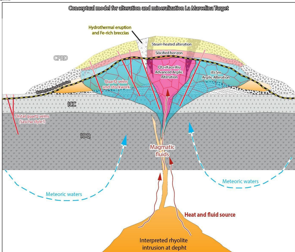
Figure 4 – Conceptual geological model of the Marcelina hydrothermal system showing the preserved silica cap, advanced argillic alteration, hydrothermal breccias and interpreted mineralised zones beneath the palaeo-water table.
