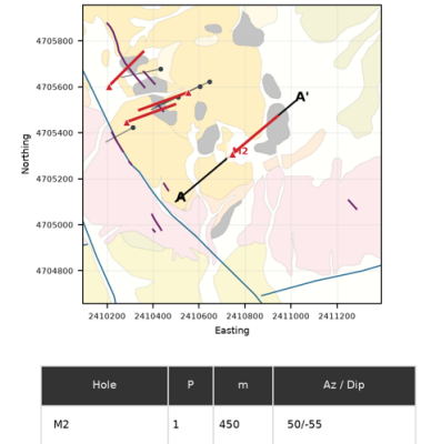
NE-directed test across Fault 2 and the 2026 geophysical response
