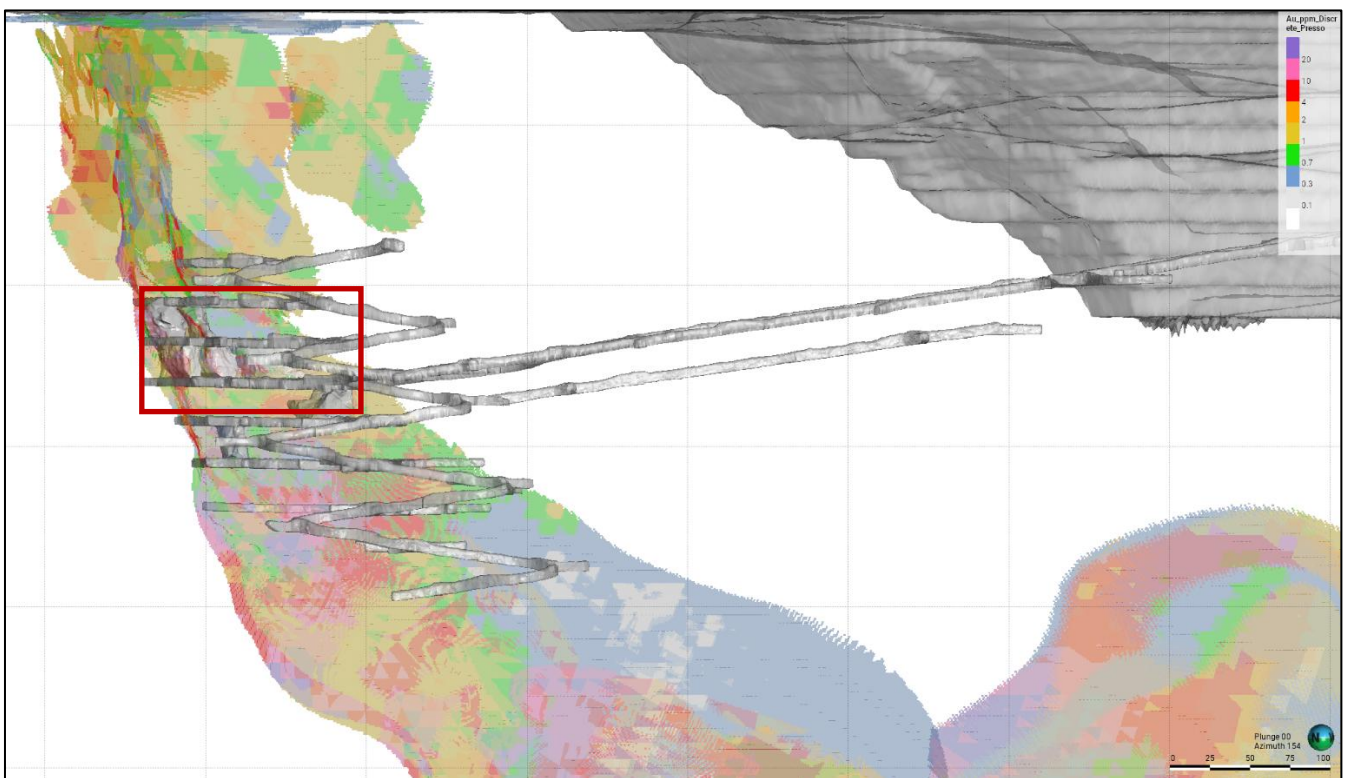
Figure 9: Never Never underground development, stoping (red box area) and pit long section with current resource estimate
