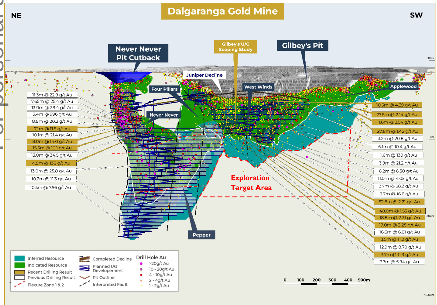
Figure 10: Dalgaranga underground mine showing recent development advance and exploration results
