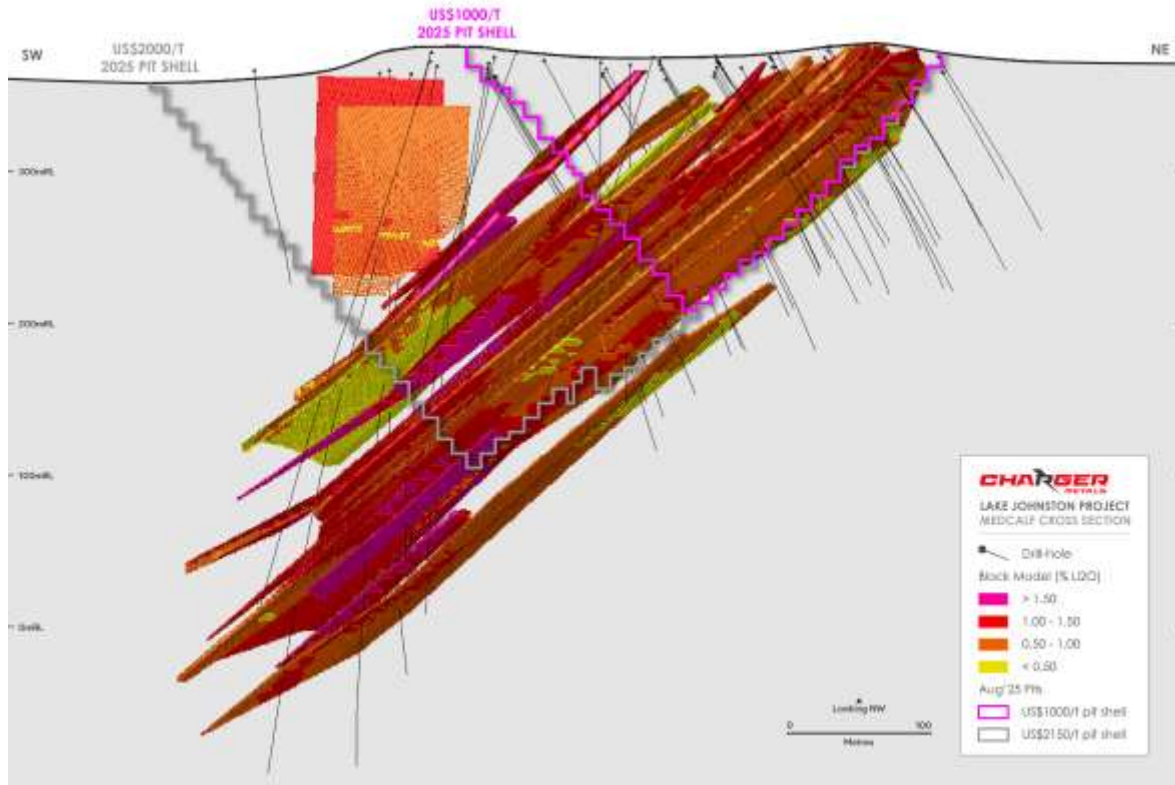
Figure 3. Oblique sectional view of the Medcalf Lithium Mineral Resource showing the pit optimisations based on spodumene concentrate (6% \text{Li}_2\text{O} ) (SC6) prices of US$1,000/t and US$2,000/t.
