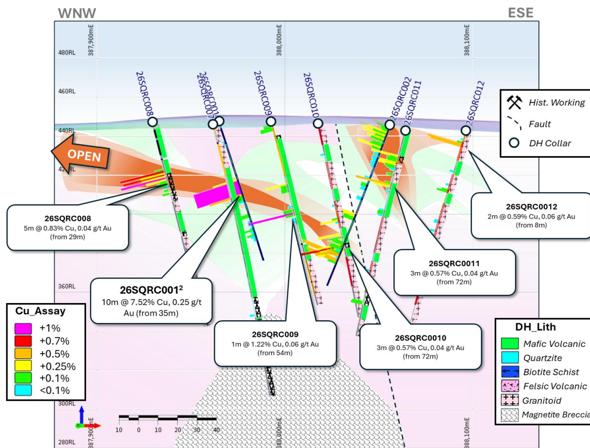
Figure 8: Long-section through the Snow Queen Prospect highlighting key intercepts and geological complexity
