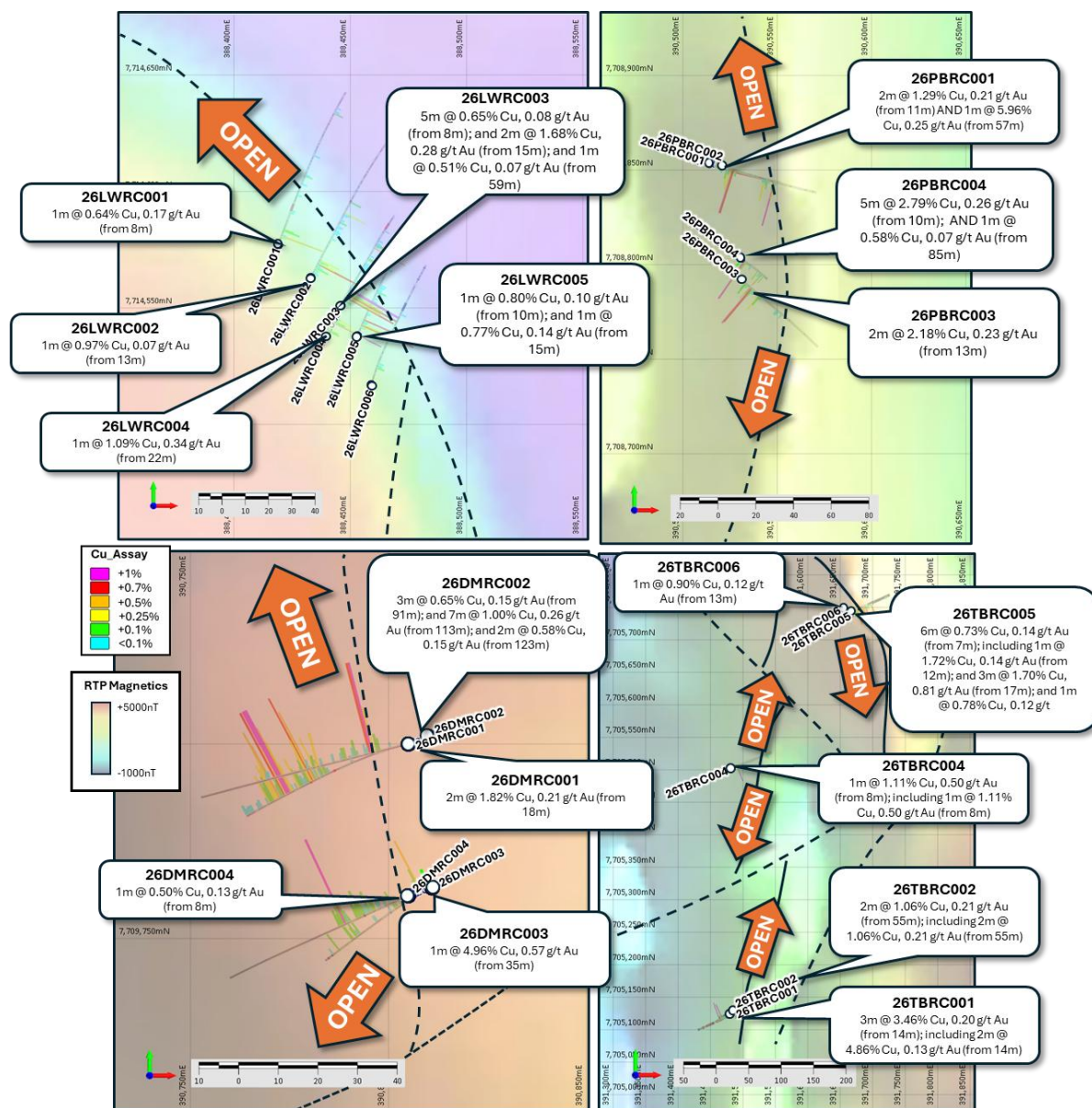
Figure 5: Plan view (with interpreted faults, contacts and extensions identified) showing drill collars and strings over the Last Weekend (top left), Playboy (top right), Dawn Marie (bottom left) and Trumby Line (bottom right) Prospects.
