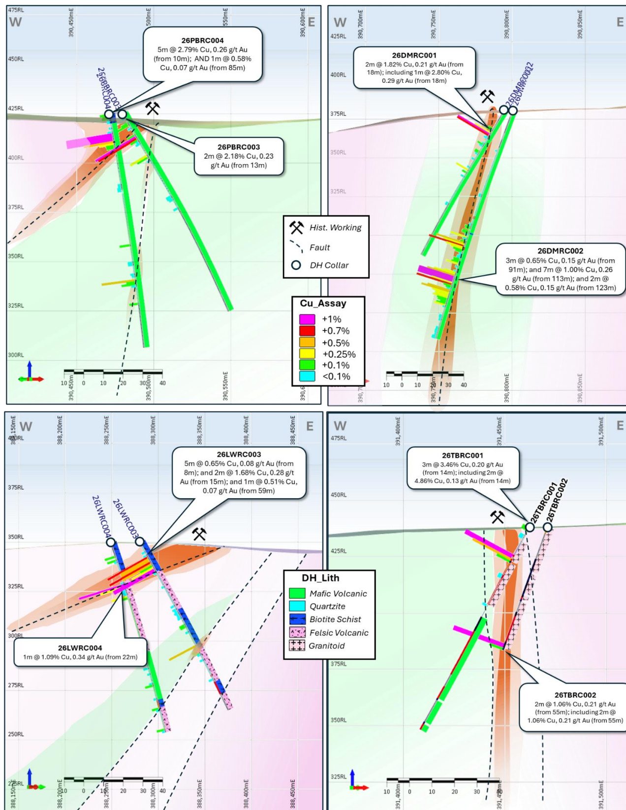
Figure 6: West-East Cross-sections (including geological interpretation) showing drillhole intercepts at the Playboy (top left), Dawn Marie (top right), Lost Weekend (bottom left) and Trumby (bottom right) Prospects.
