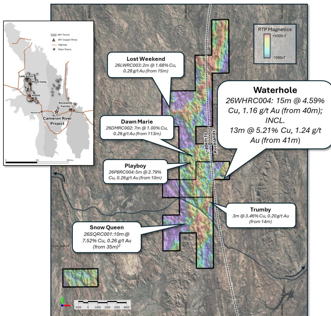
Figure 1: Plan view summary diagram showing peak drillhole intersections from reconnaissance drilling at the Cameron River Project. For a full list of 'Significant Intercepts' please refer to Appendix 2, and Full Assay results in Appendix 5.
