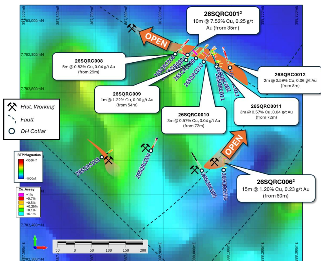
Figure 7: Plan view of the Snow Queen Area, highlighting magnetic complexity (background) and recent drill results.
