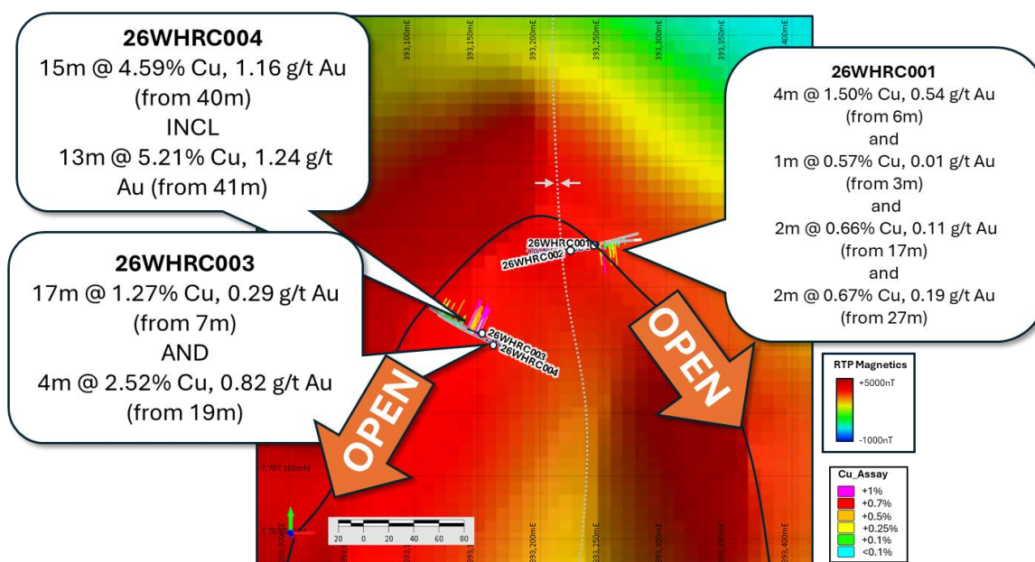
Figure 3: Plan view diagram highlighting fold-closure (via RTP magnetics) over the Waterhole Prospect.
