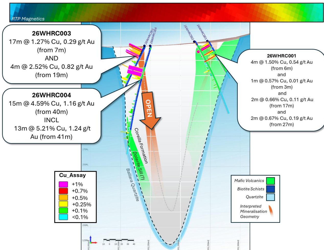
Figure 4: Cross-section through drilling at the Waterhole Prospect, showing interpreted extensions and relationship of interpreted geological relationships and plan view RTP magnetics.
