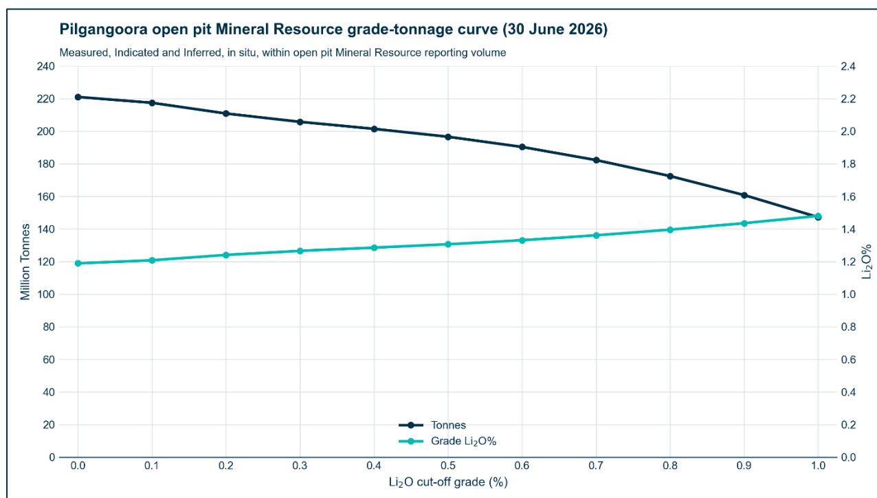
Figure 5 Pilgangoora open pit Mineral Resource grade-tonnage curve as at 30 June 2026
