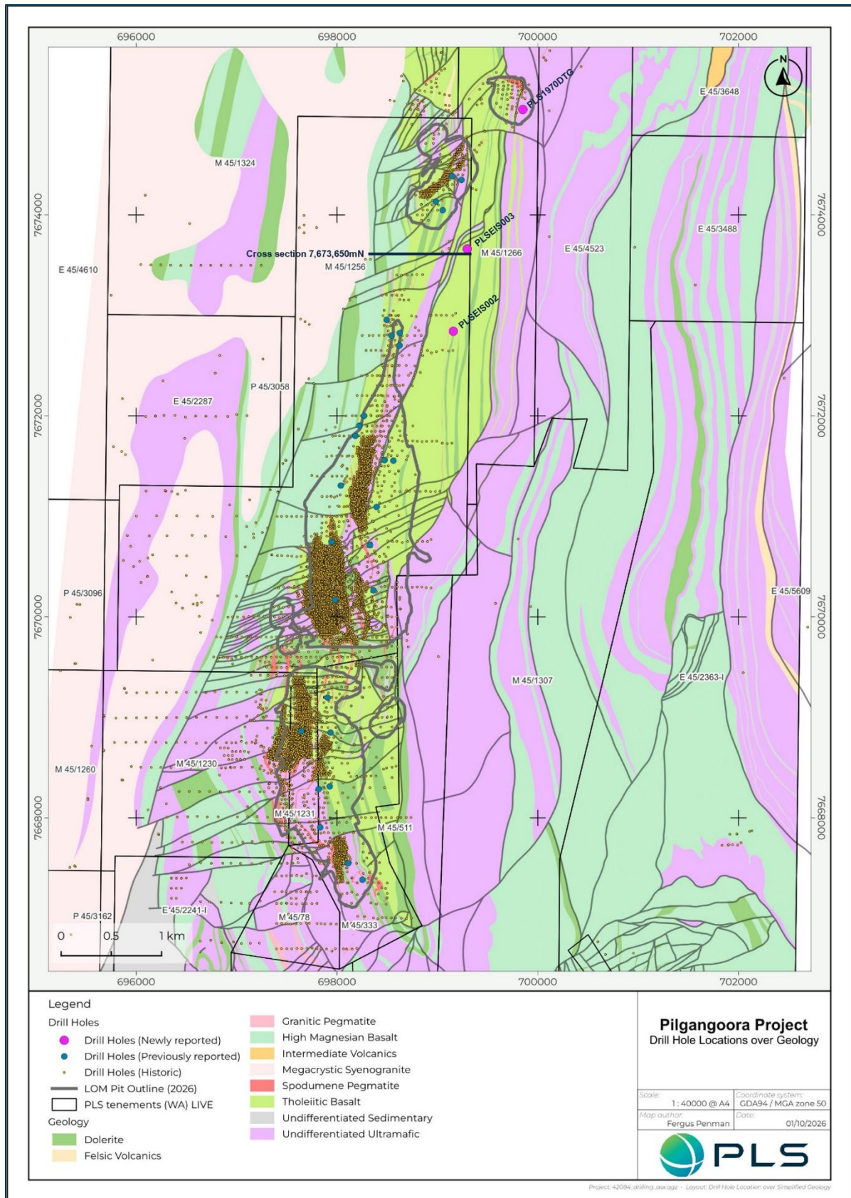
Figure 7 – Pilgangoora geology and drillhole collar plan showing new holes PLSEIS002, PLSEIS003 and PLS1970DTG, holes with additional and revised intercepts reported in this announcement and earlier drilling.
