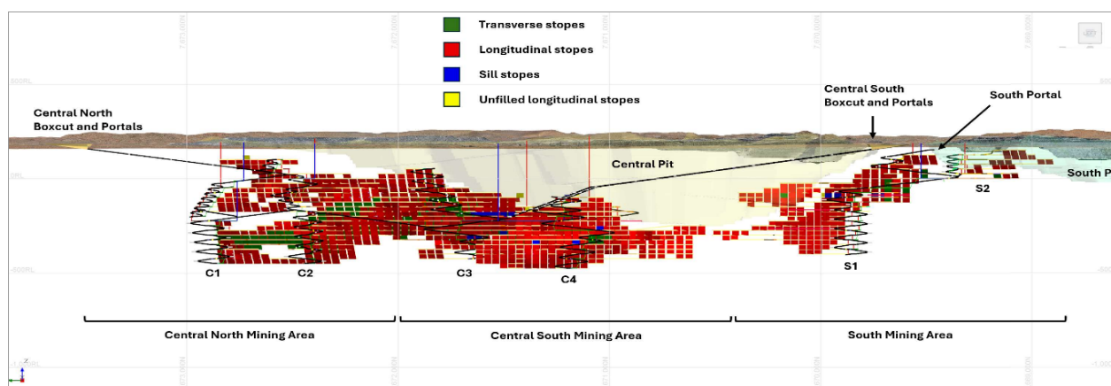
Figure 2 - Underground Ore Reserve Design (Long Section)
