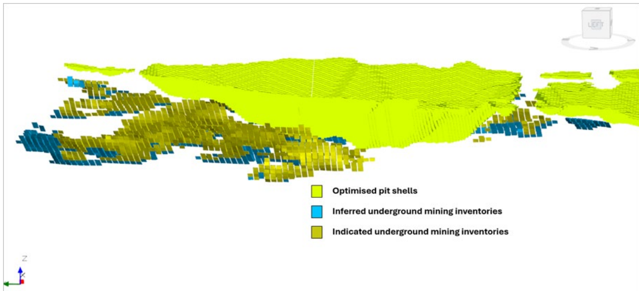
Figure 1 - Pilgangoora Optimised Pit Shells and Resulting Potential Underground Inventories
