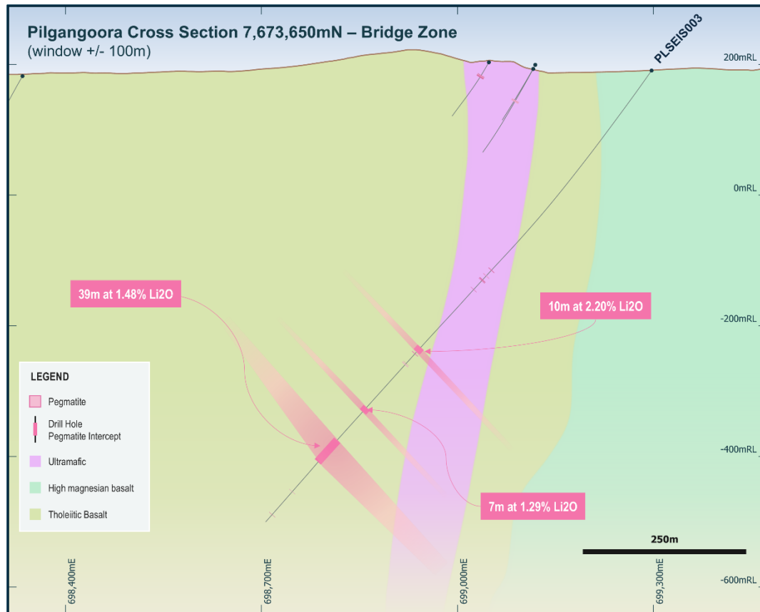
Figure 8 – Cross section 7,673,650mN – Bridge Zone (looking North)
