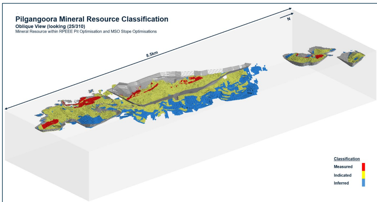
Figure 6 - Oblique view (looking 25/310) showing Mineral Resource by Classification
