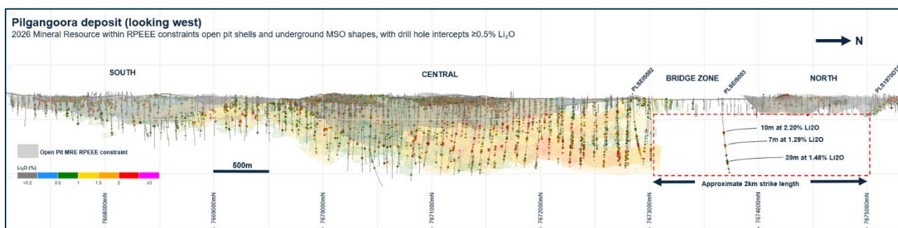
Figure 9 – Pilgangoora deposit, 3D view looking west, showing the Mineral Resource within the open pit and underground RPEEE constraints, drill hole intercepts of 0.5% \text{Li}_2\text{O} or more, and PLSEIS003 in the Bridge Zone
