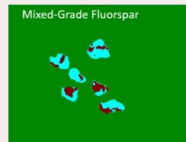
Laser ore-sorting technology by TOMRA applied to Quinn Project metallurgical samples, showing clear differentiation of ore types and waste. Samples approximately 10-15mm
