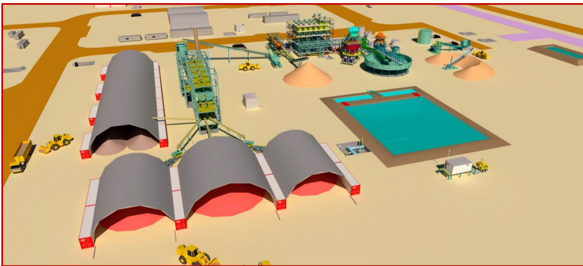
Figure 3: Port Gregory minerals sands modular plant and site layout (IHC Mining)
