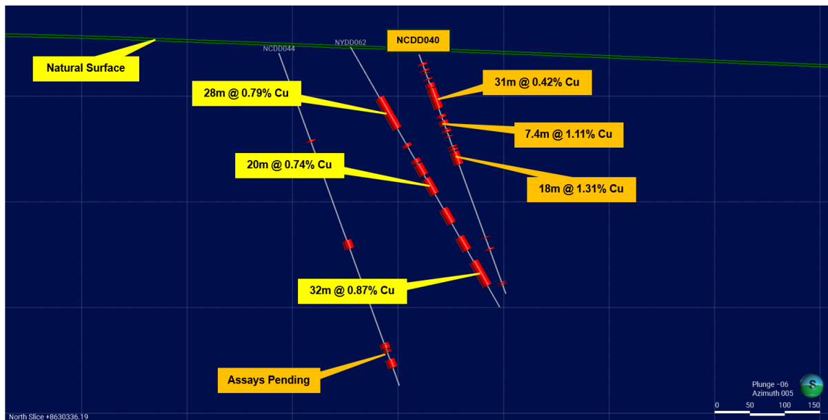
Figure 1. Nyungu Central drilling section at 8630350mN showing recent NCDD040 drilling result (looking north)
