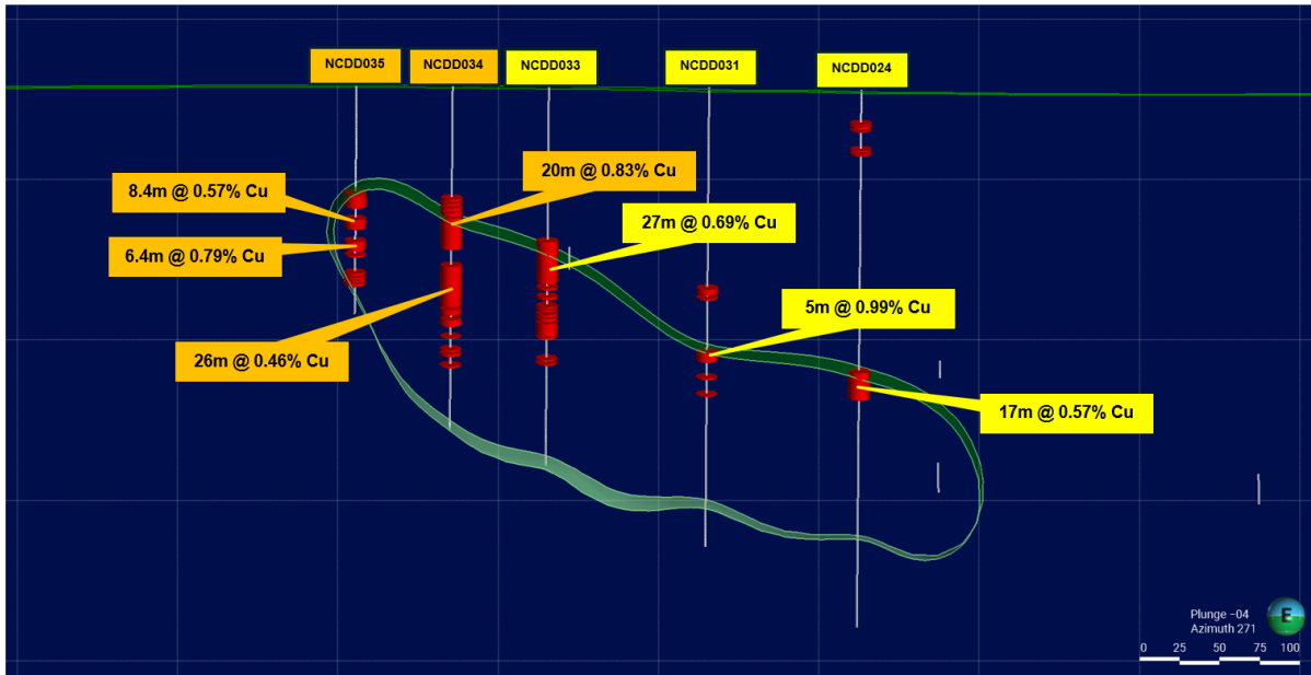
Figure 5. Long section projection at 339450mE showing Nyungu Central southeast mineralisation – as green ellipse (looking west)
