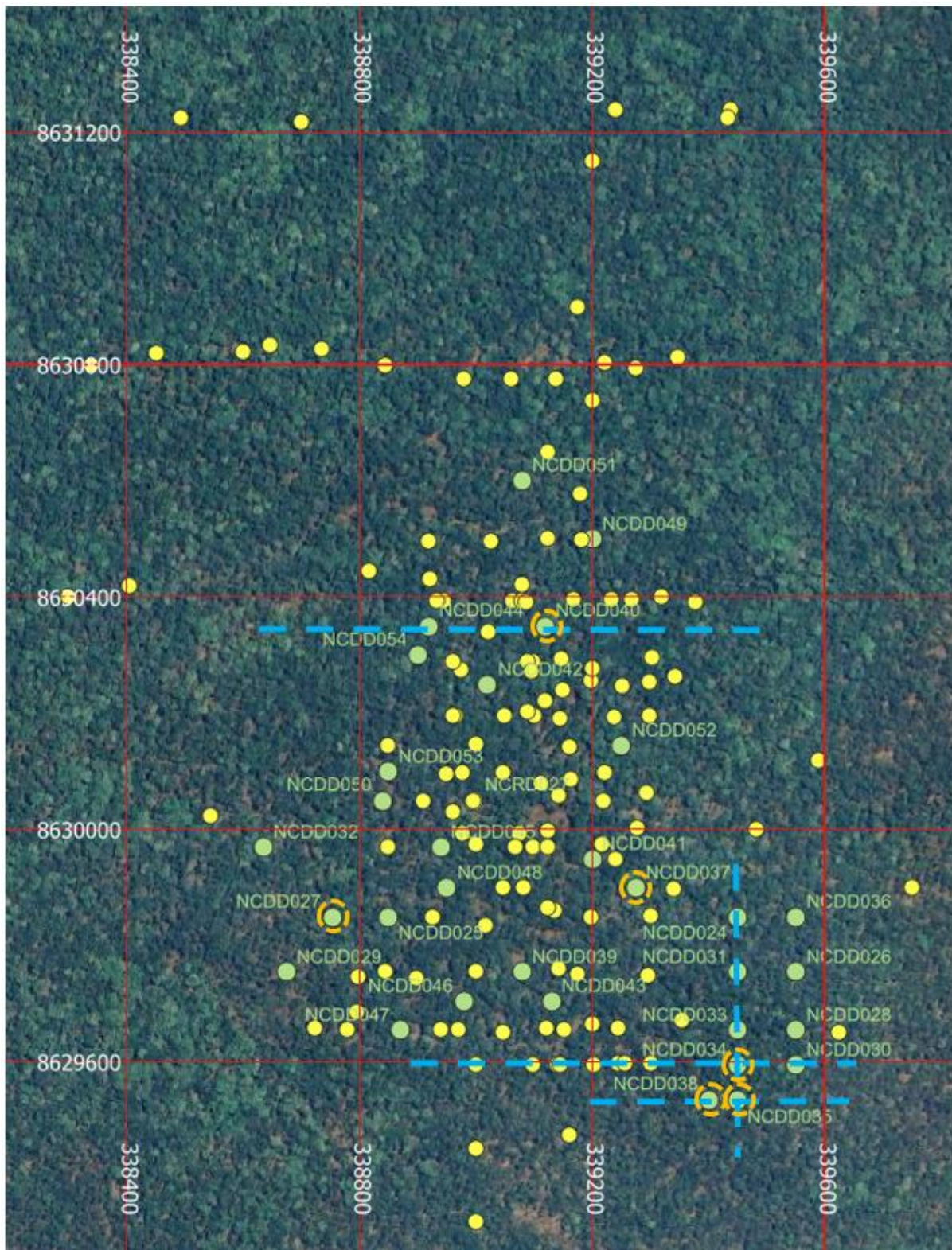
Figure 2. Nyungu Central drill hole collar plan showing Phase 3 drill holes (green); pre-2026 holes (yellow); reported holes (dashed orange) and sectional projections shown in Figures 1, 3, 4 and 5 (as dashed blue lines)
