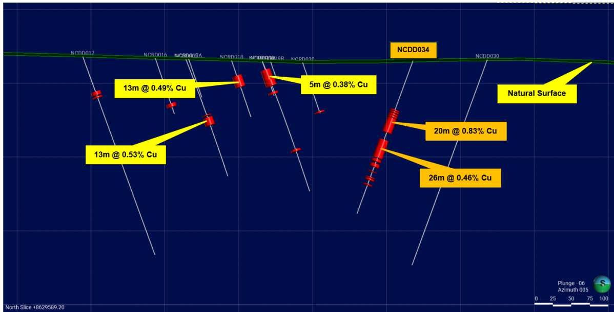
Figure 3. Nyungu Central drilling section at 8629600mN showing recent NCDD034 drilling result (looking north)
