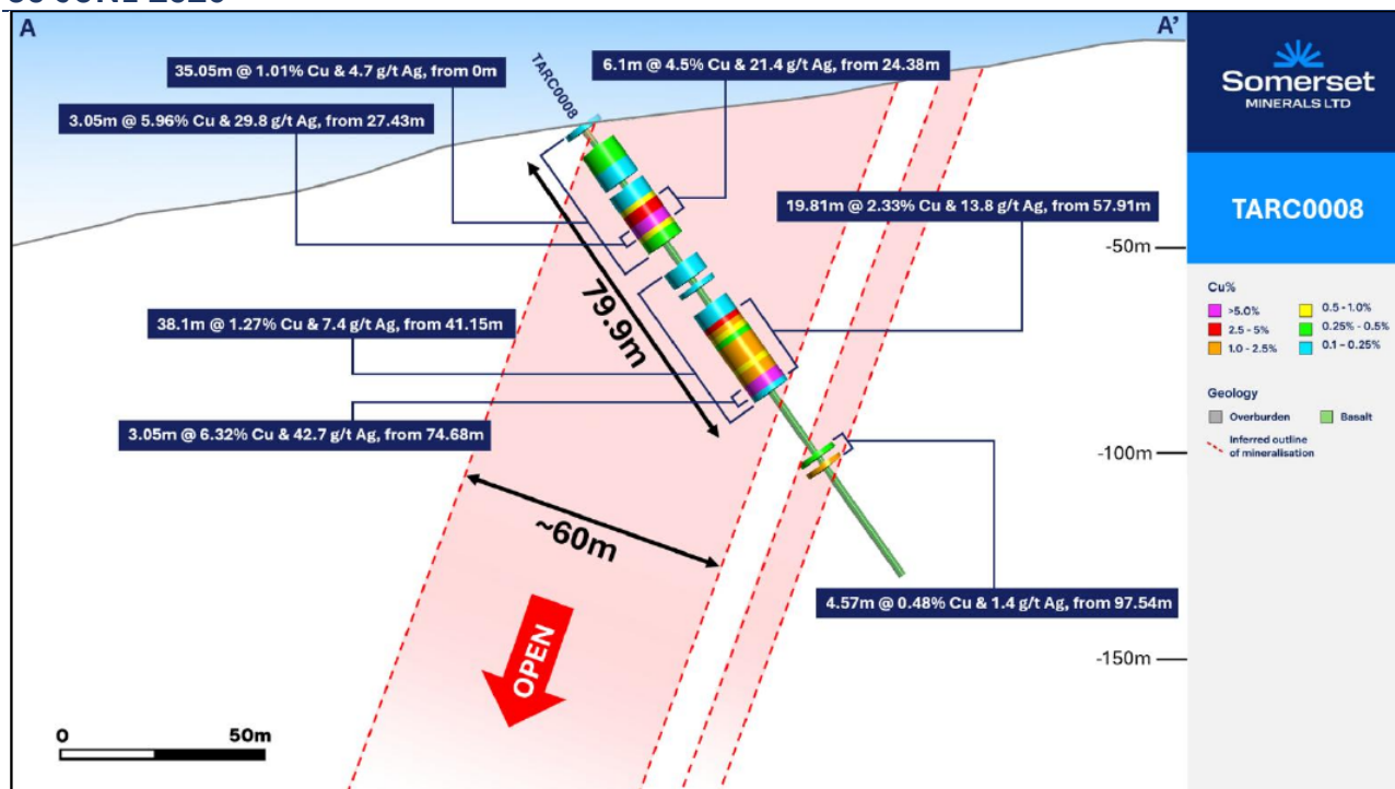
Figure 7: Cross section through TARC0008.
