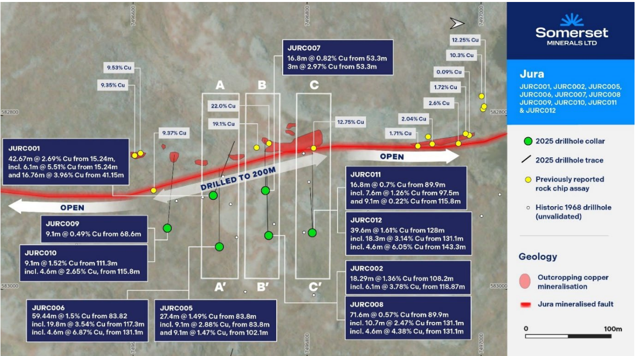
Figure 2: Plan map showing drill hole collar locations and significant intercepts.
