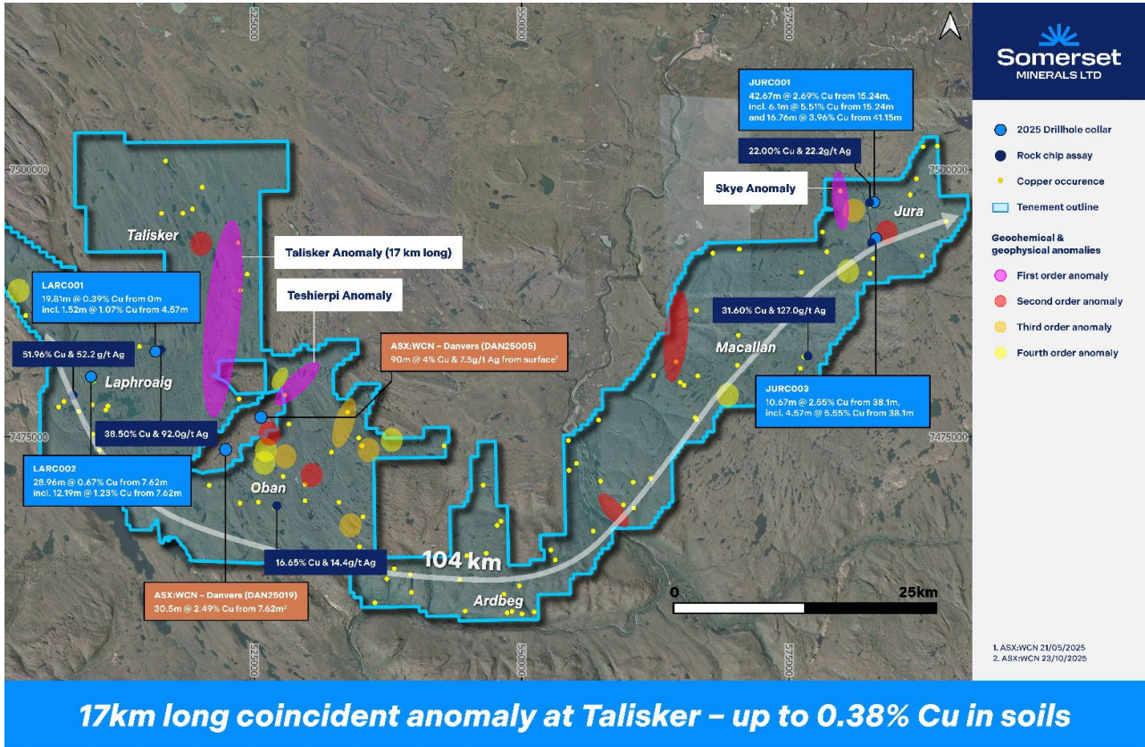
Figure 1: Somerset Minerals Coppermine Project showing coincident airborne magnetic and till geochemical anomalies (ranked), highlighting the ~17 km Talisker Corridor (up to 0.38% Cu in till) and proximity to White Cliff Minerals' Danvers copper project. See ASX:SMM 04/02/2026.
