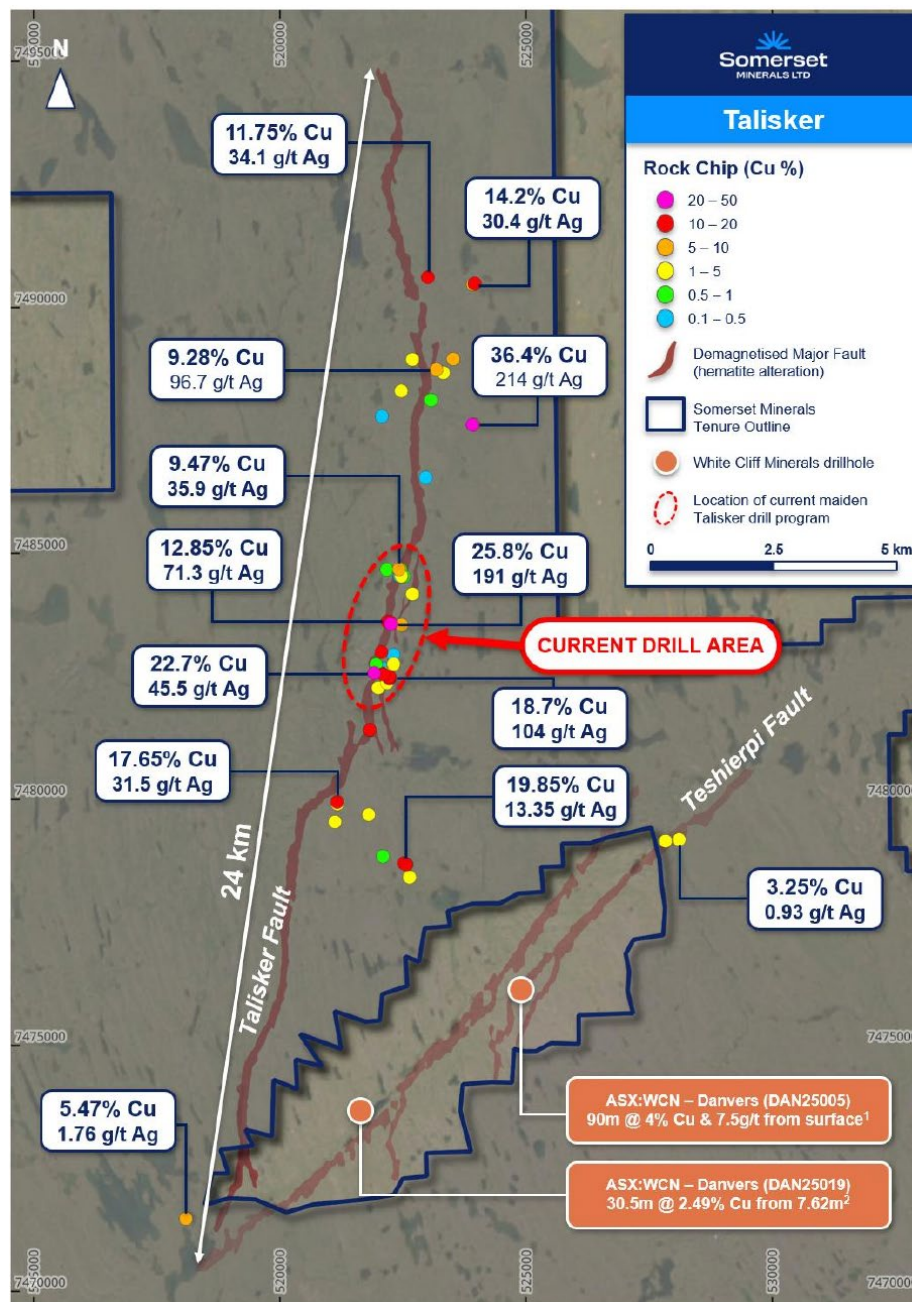
Figure 5: Location of surface rock chip results above 0.1% Cu across the Talisker district.
