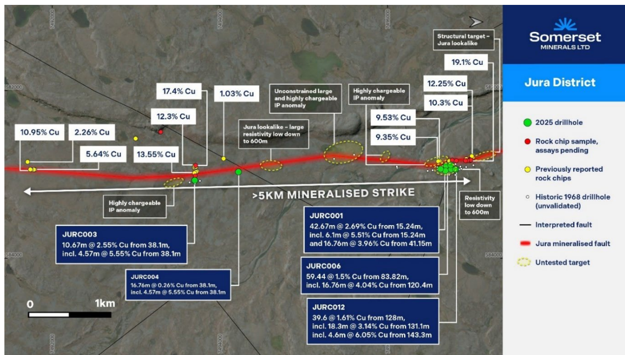
Figure 3: Plan map showing wider Jura prospect area, drill hole collar locations, significant intercepts and rock chip samples.
