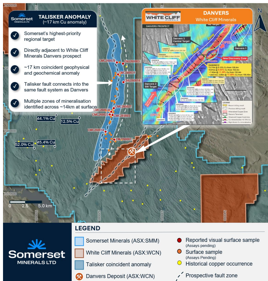
Figure 4: Talisker combines proximity to Danvers, demagnetised geophysics, Cu geochemistry and multiple mapped surface copper occurrences over ~14km. This image contains references to drill results derived by other parties either nearby or proximate to the Coppermine Project and includes references to topographical or geological similarities. It is important to note that such discoveries or geological similarities do not in any way guarantee that the Company will have any success or similar successes in generating similar results, if at all. (See ASX:SMM 24/06/2026; ASX:WCN 10/06/2026).
