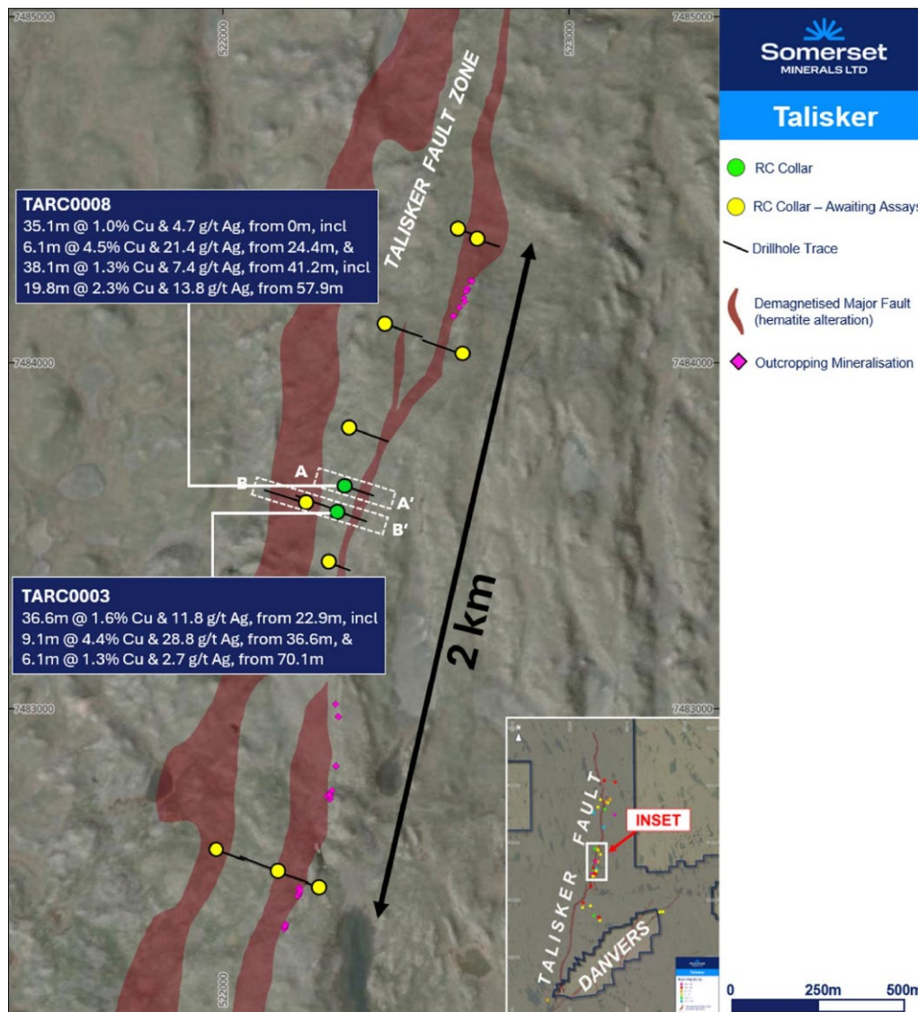
Figure 6: Plan map of the Talisker corridor showing drillhole collar locations, significant intercepts, outcropping copper mineralisation, and the demagnetised signature of the Talisker fault zone.
