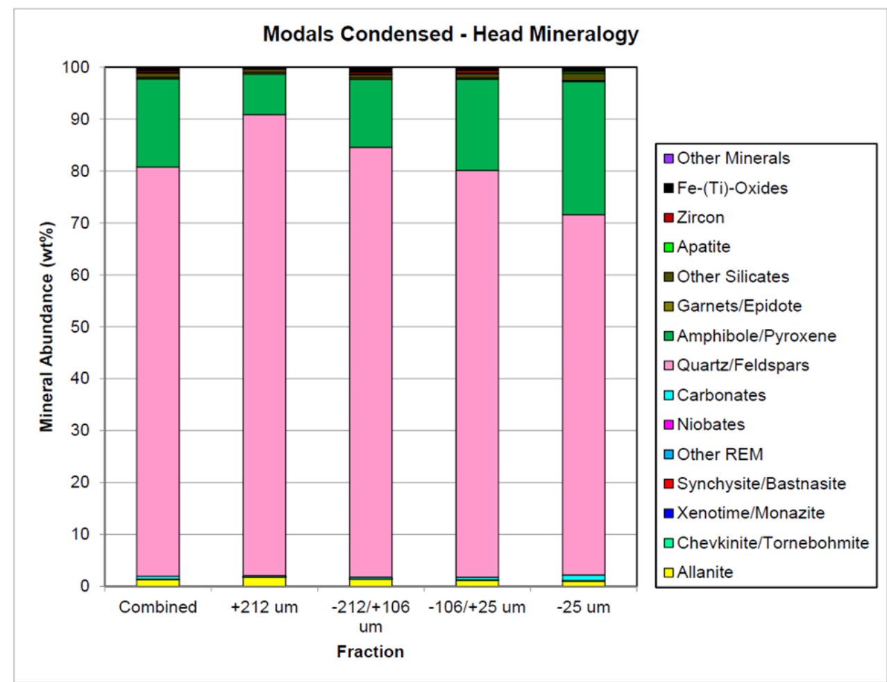
Figure 5-10. Modal Mineralogy by Size and Calculated Head
