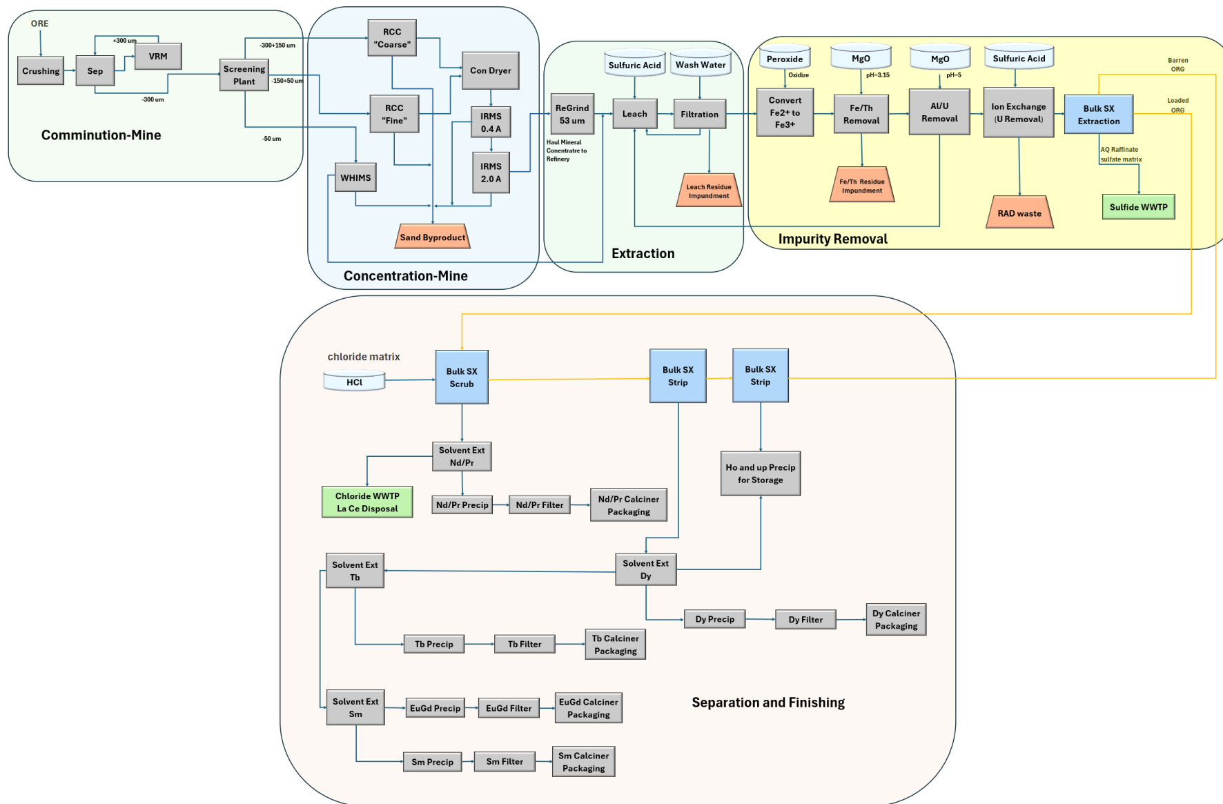
Figure 13-1. Preliminary Process Flowsheet — Halleck Creek Rare Earth Project
