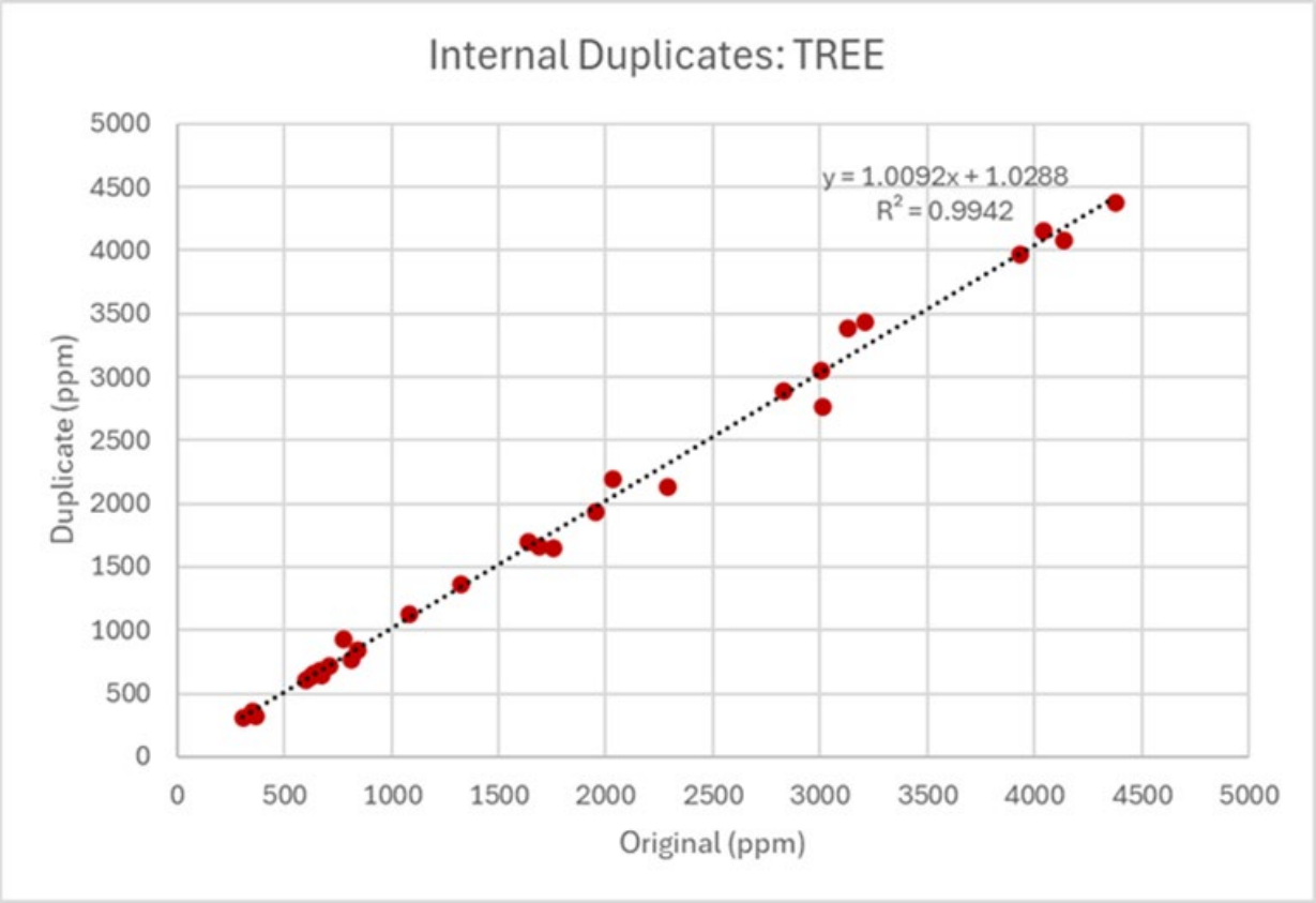
Figure 7-5. Company Internal Duplicates — TREE Scatter Plot and Regression Curve ( R^2 > 0.99 )
