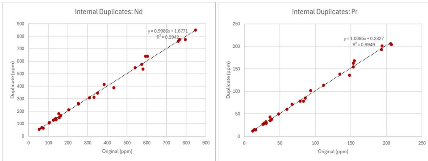
Figure 7-7. Chart of Internal Duplicates for Nd and Pr
