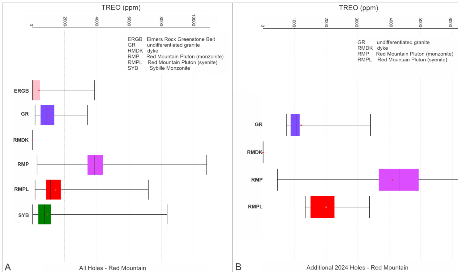
Figure 10-2. Boxplot of TREO Grade for Geological Domains
