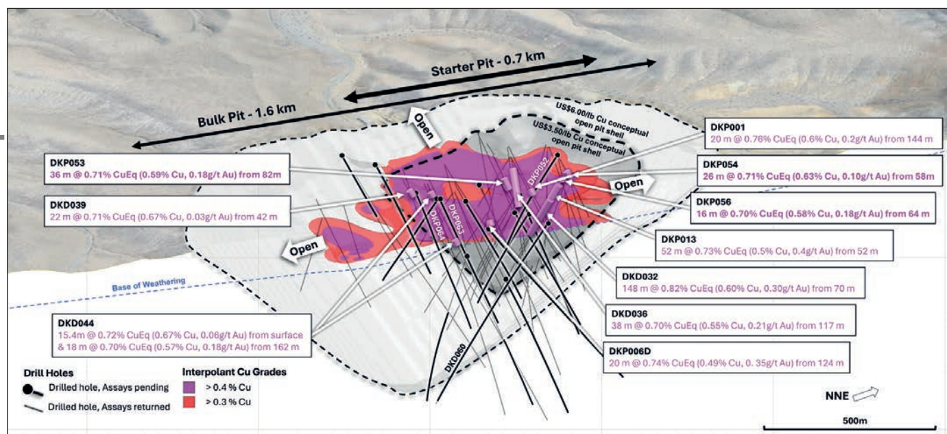
Figure 2. Oblique slice towards NW (Azi 325°, Plunge+26°). 0.3% and 0.4% Cu interpolants displayed for oxide and transitional material, sliced along NNE orientation with the front removed. US$3.50/lb Cu conceptual open pit shell displayed in dark grey; US$6.00/lb Cu conceptual open pit shell displayed in light grey 1 . Base of weathering shown as dashed blue line. Results reported including CuEq 2 and in some instances represent subsequent material results, post reporting period.
