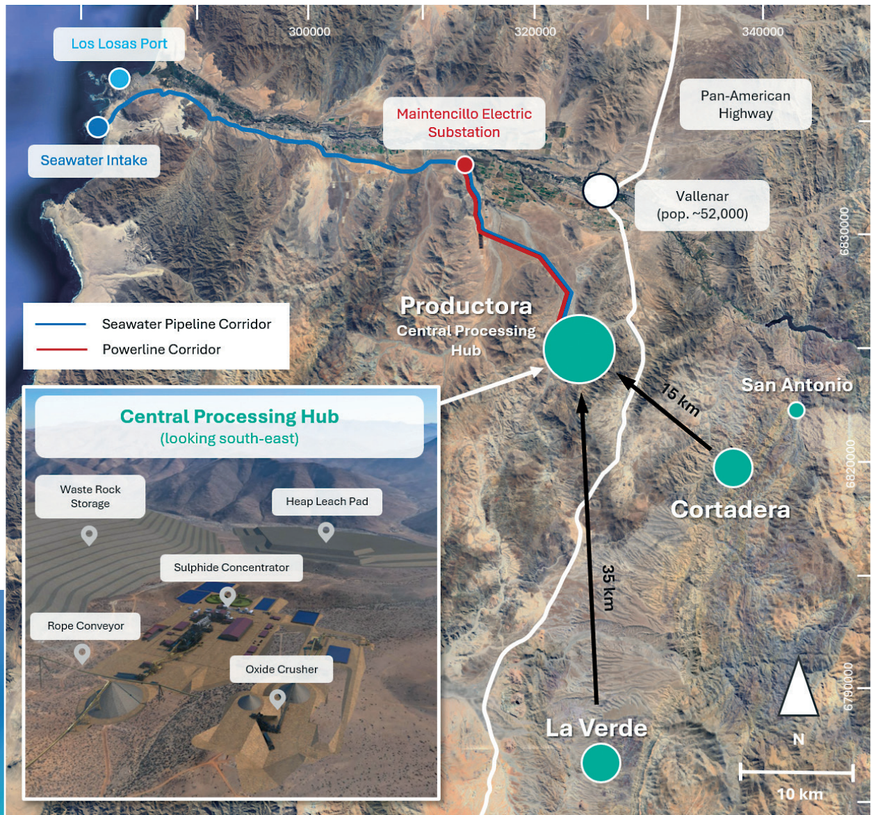
Figure 4. Plan view of the Costa Fuego Project Layout, including the La Verde discovery and integrated infrastructure at Productora.
