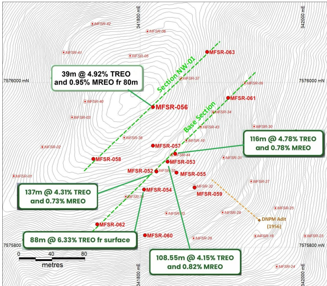
Figure 2. Location map showing current Power Minerals Morro do Ferro drillholes and intercepts from previous drillholes (see ASX announcements dated 8 April 2026). Drilling is progressing across and along strike from the central location. The LiDAR survey by PNN topographic contours lines at 1m interval are shown
