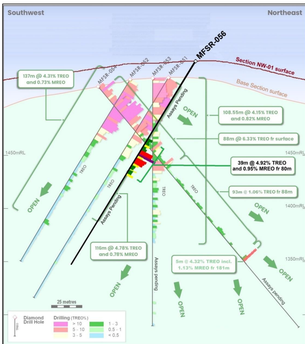
Figure 1. Cross-section looking northwest showing the section with MFSR-056 further up the hill, together with drillholes from the Base section further southeast. MFSR-056 is at a higher elevation than previous drillholes, and the high-grade REO (red-purple) extends lower. The whole-rock TREO percentage is colour-coded on the drill traces. Not all results are available for the lower and upper parts of MFSR-056 and the lower part of MFSR-054. Results for MFSR-051, MFSR-052, MFSR-053,
