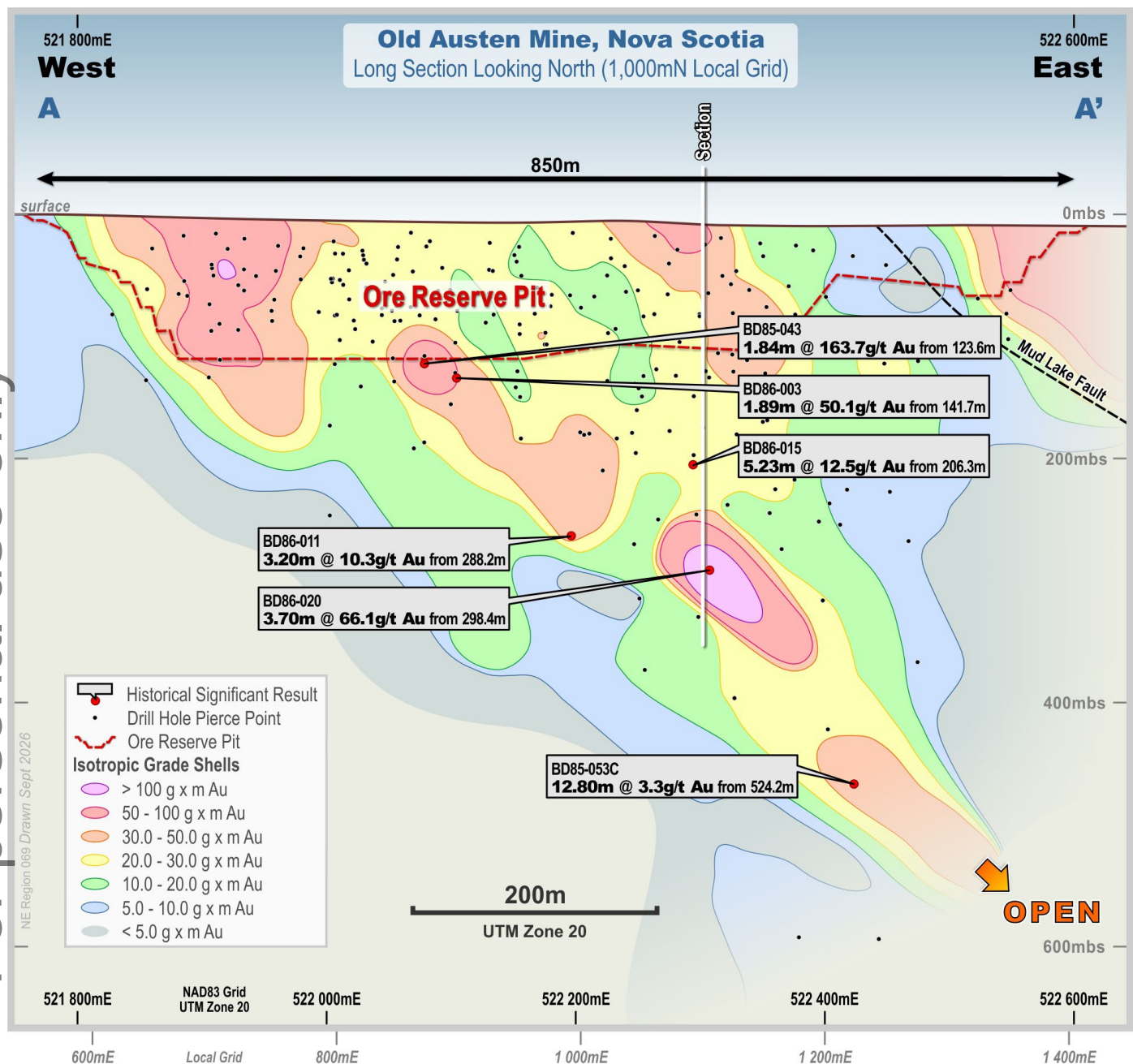
Figure 4. Old Austen Mine Down-Plunge Prospect Long Section, Nova Scotia, Canada
