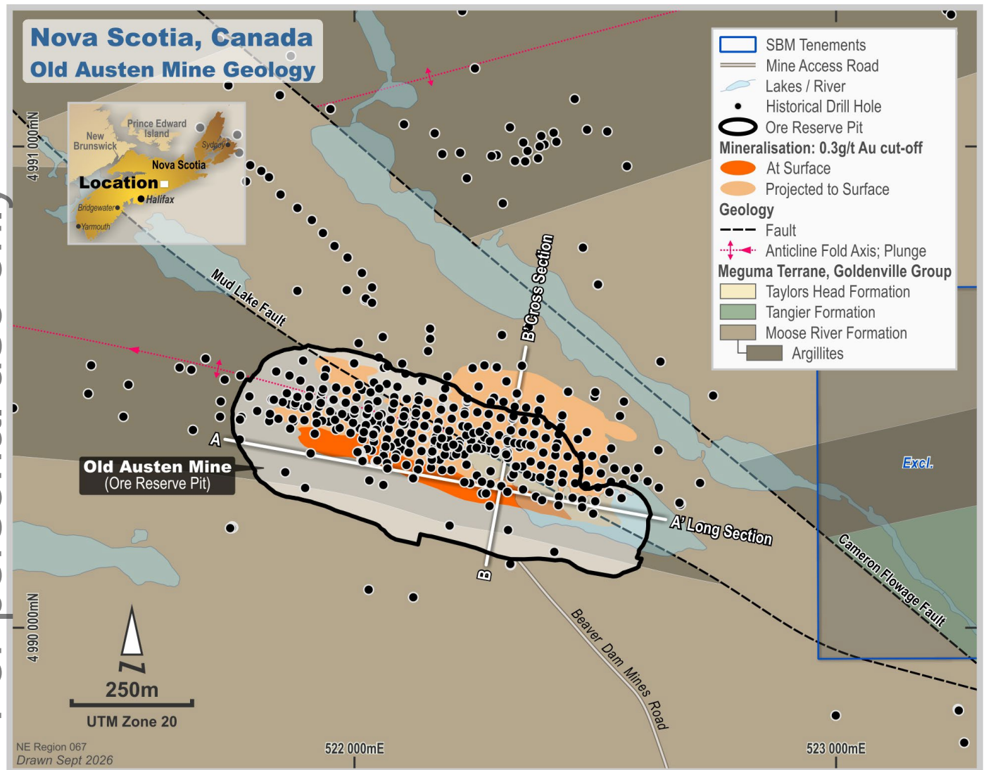
Figure 3. Old Austen Mine Geology, Nova Scotia, Canada
