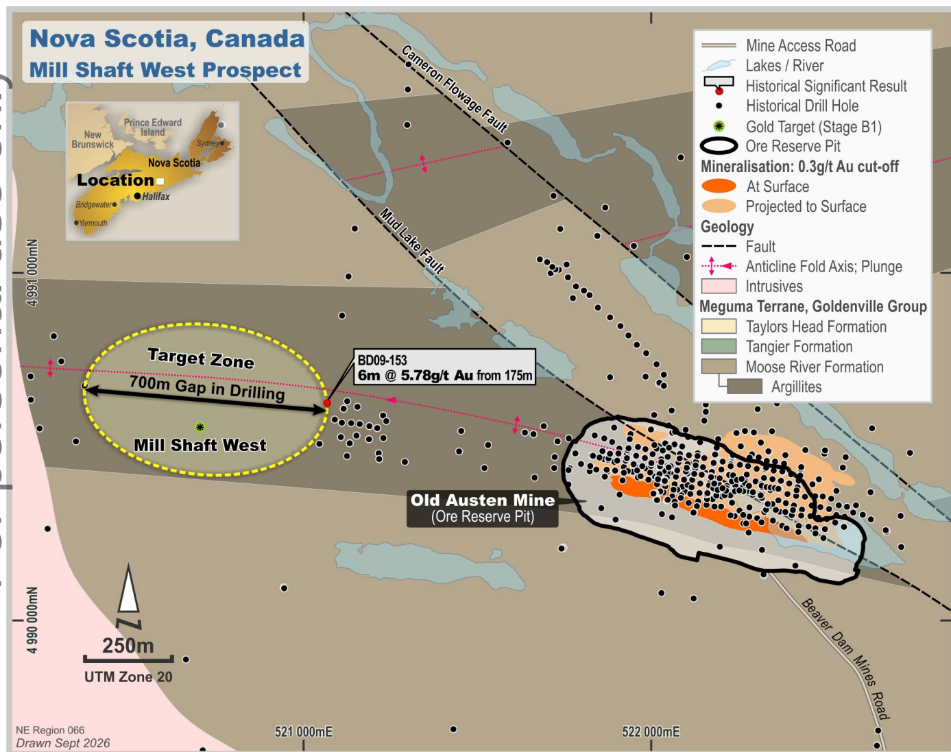
Figure 6. Mill Shaft West Prospect, Nova Scotia, Canada
