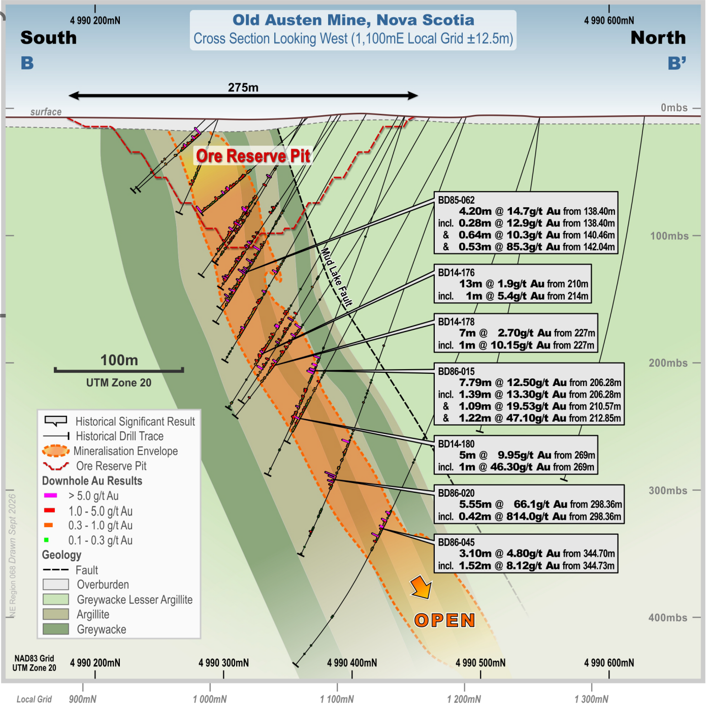
Figure 1. Old Austen Mine Down-Plunge Prospect Cross Section (equivalent to 1,100 m E Mine Grid), Nova Scotia, Canada
