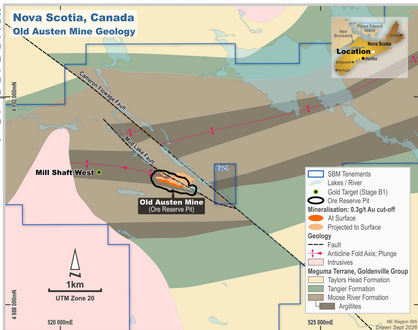
Figure 2. Old Austen Mine Down-Plunge and Mill Shaft West Geology, Nova Scotia, Canada
