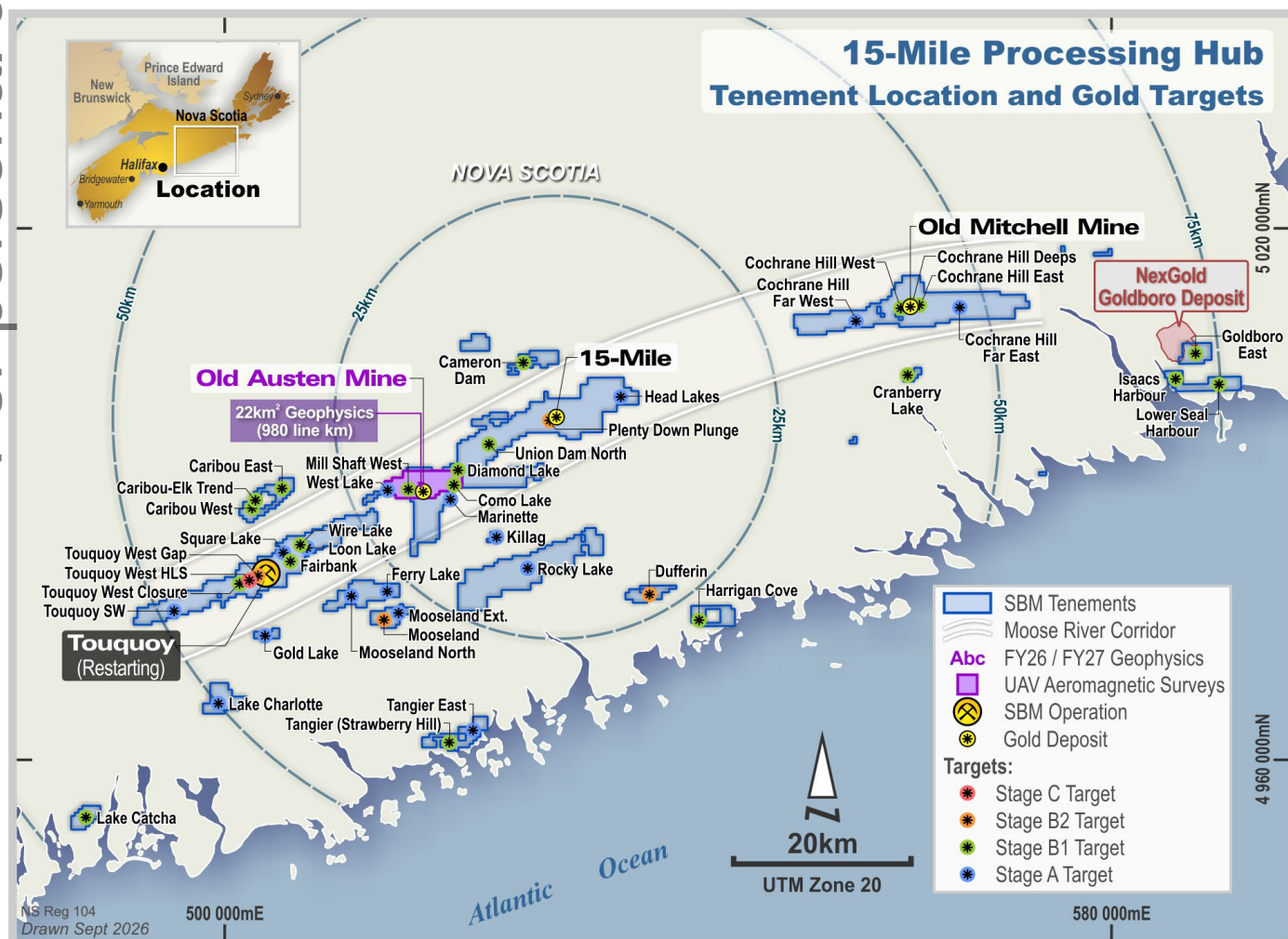
Figure 5. 15-Mile Processing Hub Exploration Targets and Old Austen Mine Down-Plunge Prospect and Mill Shaft West Prospect Locations, Nova Scotia, Canada
