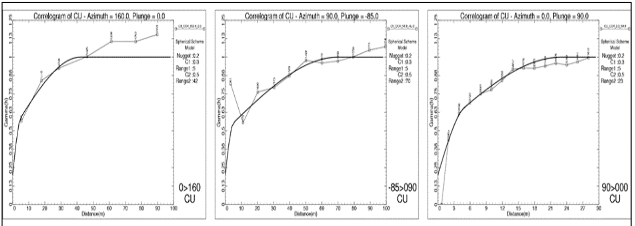
Figure 8-11. Correlogram models.
