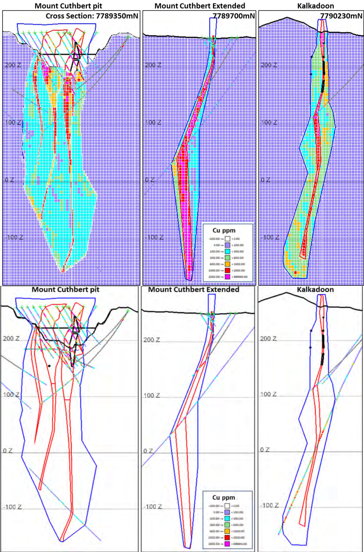
Figure 8-12. Selected cross sections of copper in model (top) vs drillhole data (bottom).
