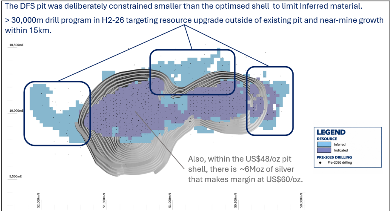
Figure 2 Target areas for pit and mine life expansion
