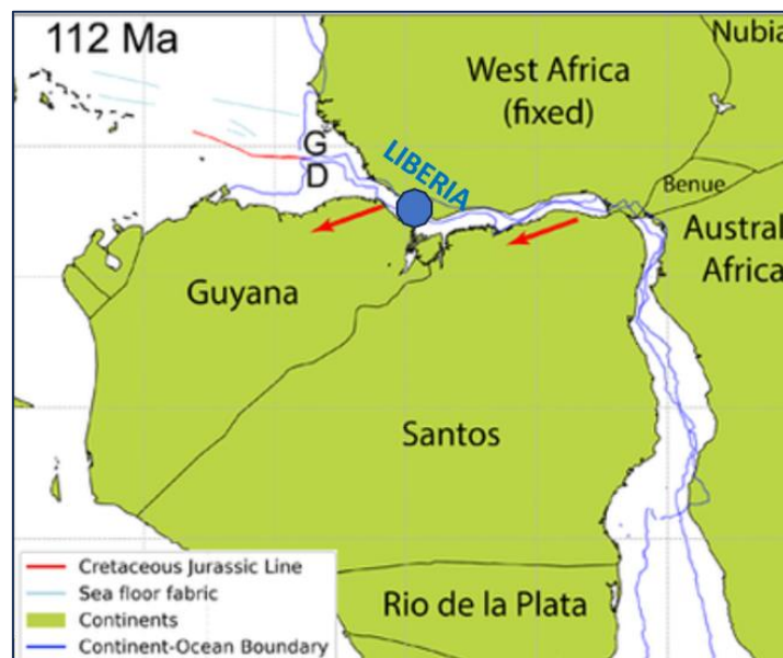
Figure 4: Pre-rift conjugate margin South America/West Africa showing Liberia and Guyana Source: Lesourd—Laux et al (2025). New Kinematic Model of the Early Opening of the Equatorial Atlantic Realm
