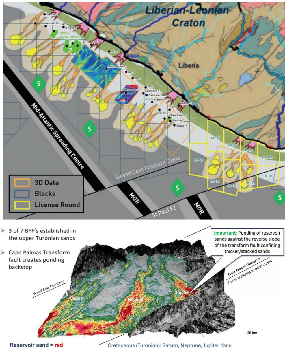
Figure 3: Top – schematic diagram showing late Cretaceous channel and turbidite fan systems. Source: TGS (data property of TGS); Winter et al. 2020. Bottom – BlueEnergies mapping of the Saturn, Neptune and Jupiter Fans. Source: BlueEnergies.
