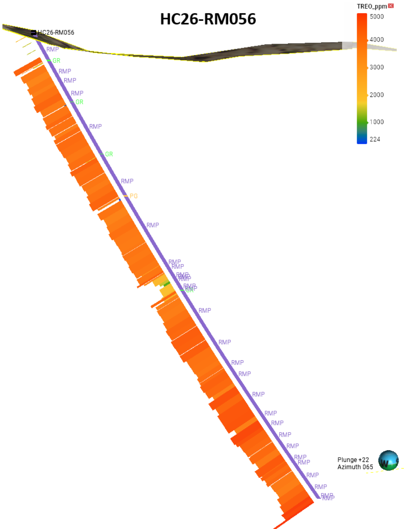
Figure 4 HC26-RM056 Cross Section Showing Down-Hole TREO Distribution
