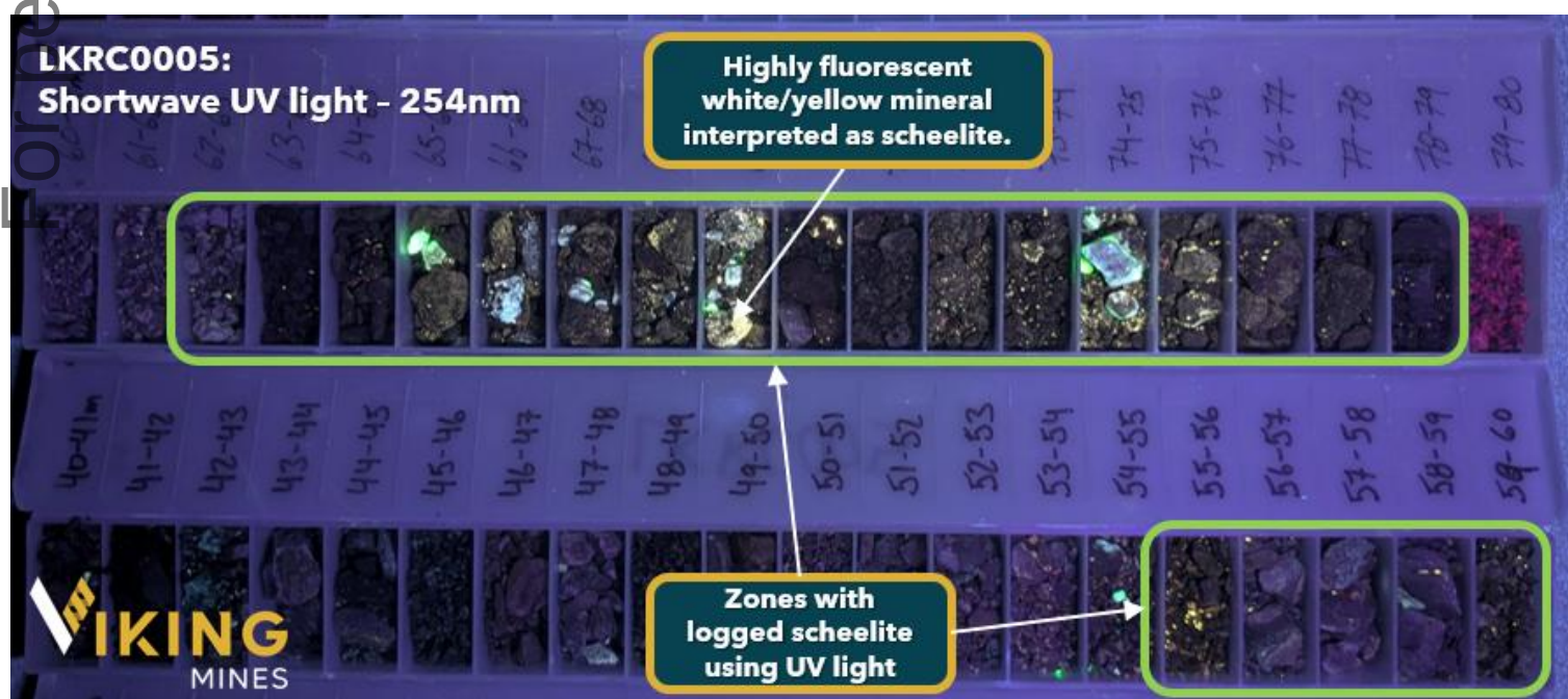
Figure 1; Photograph under shortwave UV light (254nm) of chip tray from hole LKRC0005. Downhole intervals are 1m. Note 22m interval highlighted with interpreted visual estimate range of abundance from 0.1% to 1.5% scheelite. Assay results expected in 6-8 weeks.
