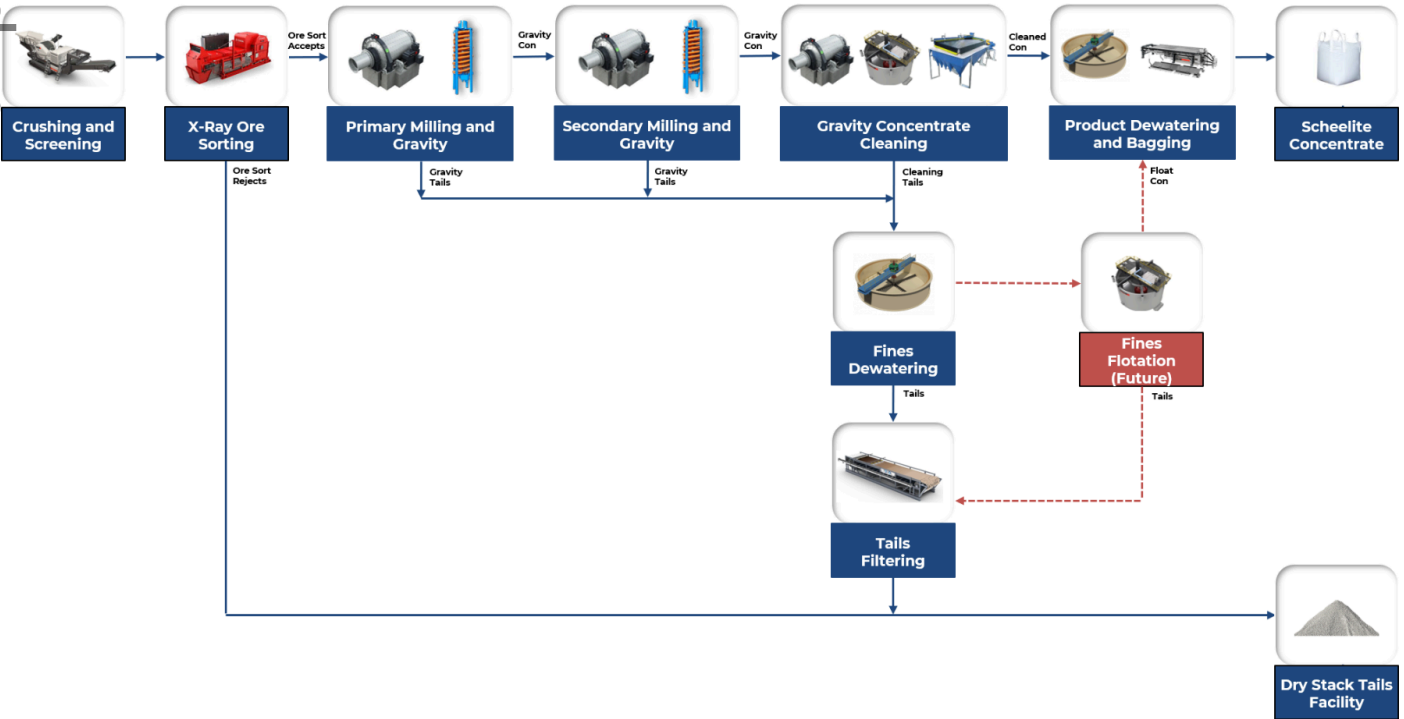
FIGURE 6 — SUMMARY BLOCK FLOW, WATERSHED DFS PROCESSING FLOWSHEET
