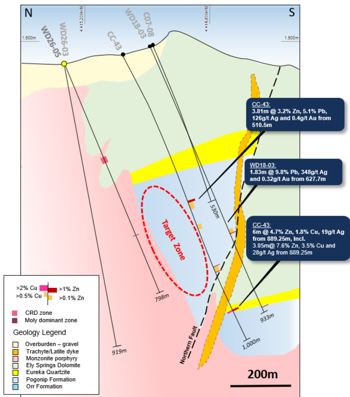
Figure 10: Schematic geological section at 289,920E (+/-150m) showing main geological units and drilling. A simplification of the mineralised intervals in WD26-05 is shown.
