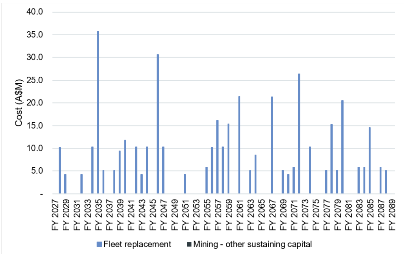
Figure 7.13 Plan C sustaining capital cost (over time)
