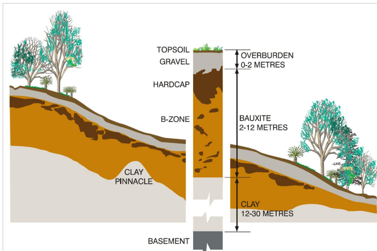
Figure 3.1 Typical laterite weathering profile
