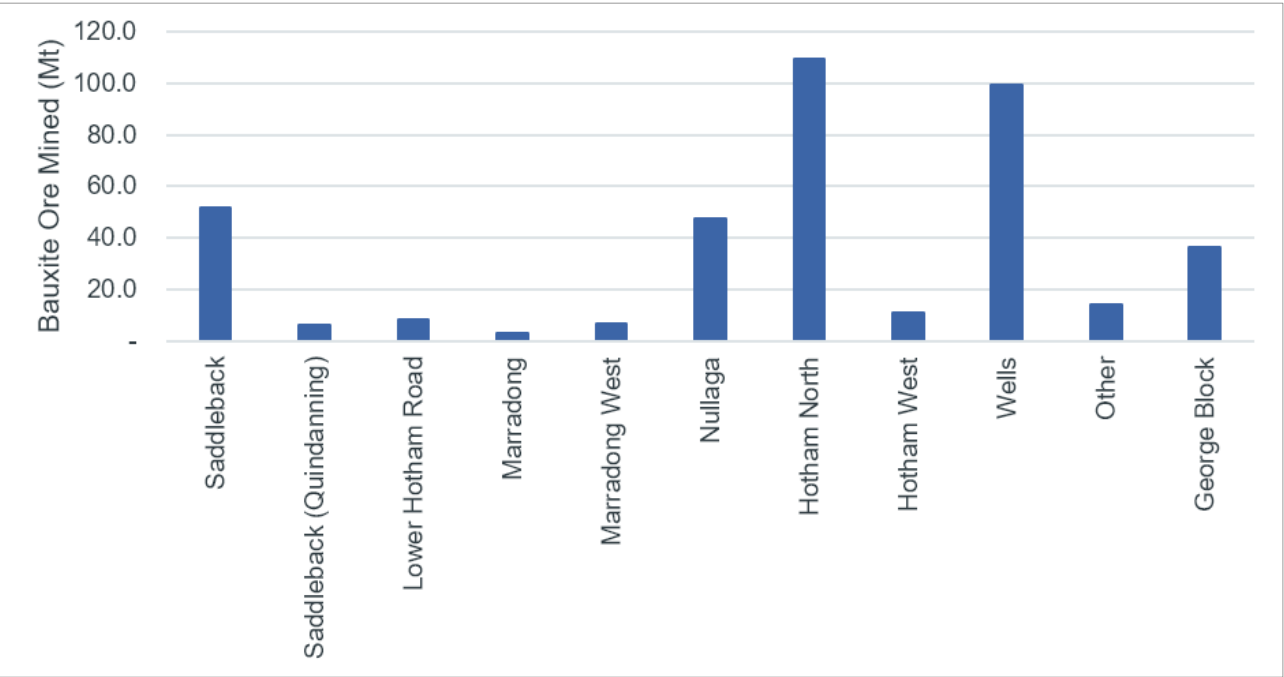
Figure 7.7 Plan B tonnage by mining area
