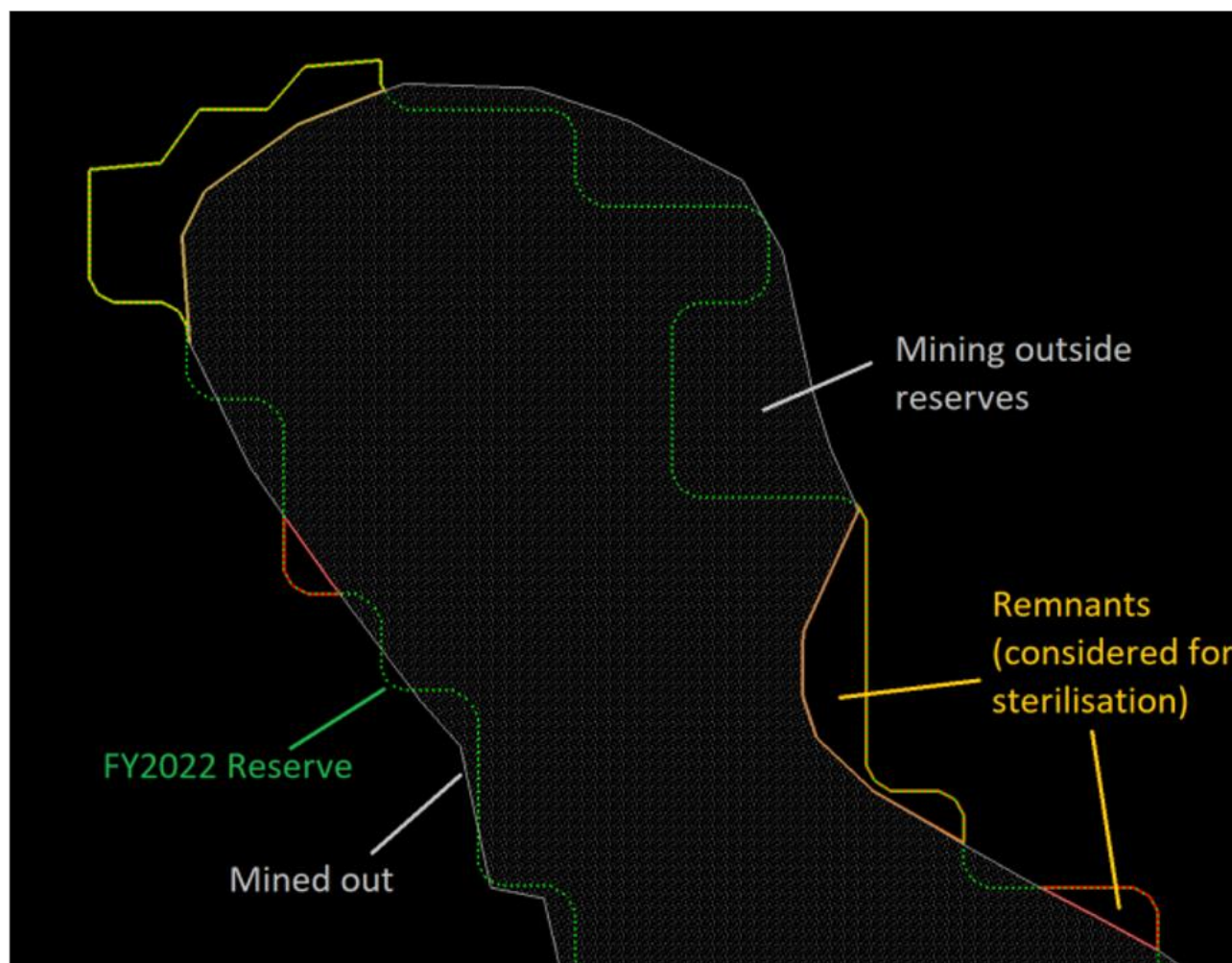
Figure 4.2 Plan vs actual mining areas
