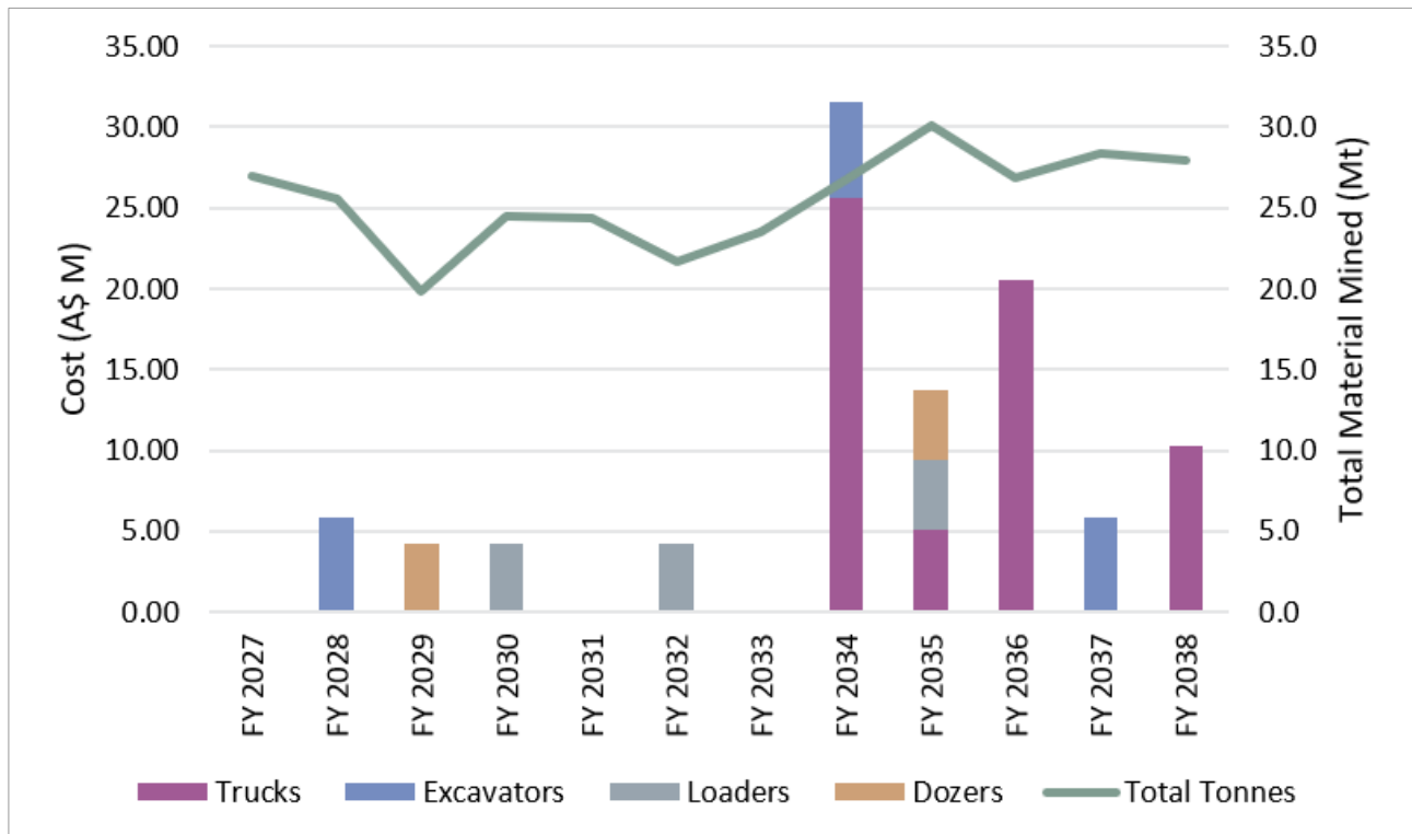
Figure 7.4 Plan A sustaining capital costs (over time)
