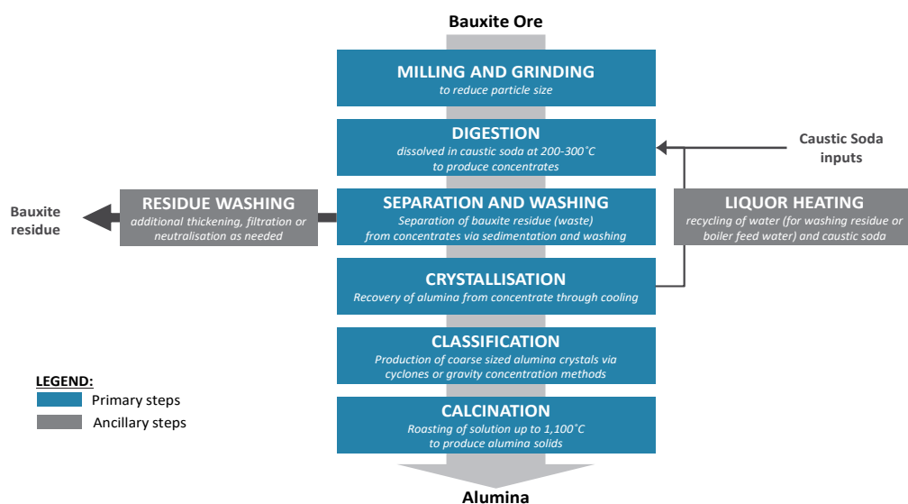
ILLUSTRATIVE ALUMINA REFINERY FLOWSHEET
