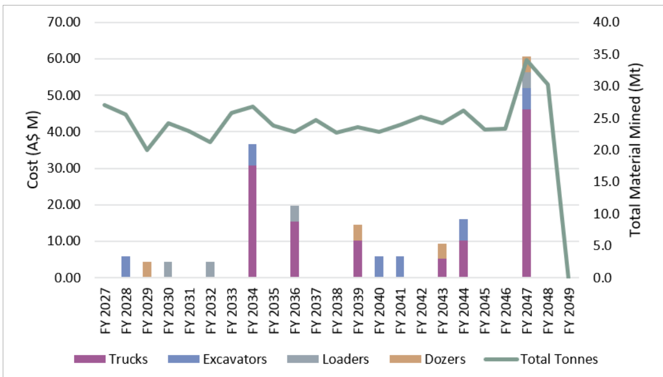
Figure 7.9 Plan B sustaining capital (over time)
