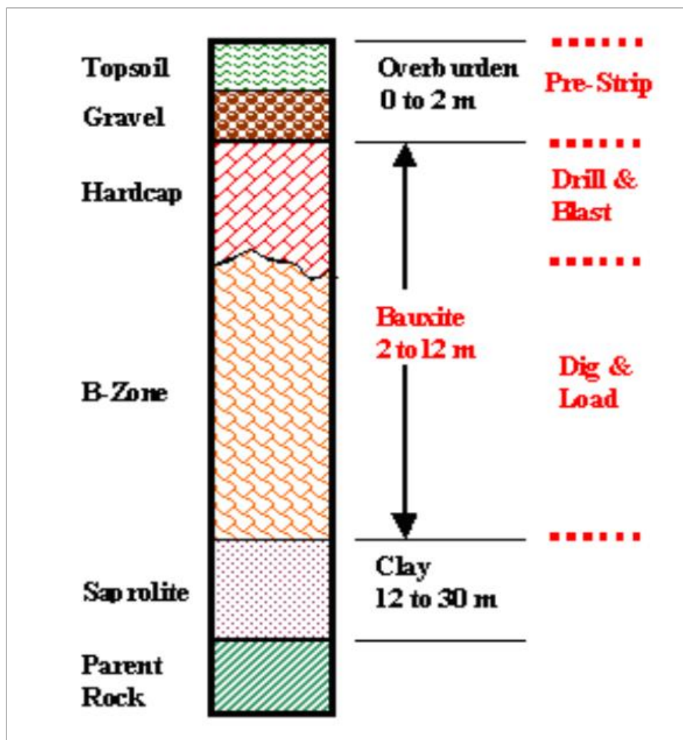
Figure 4.1 Indicative column through the mining zone
