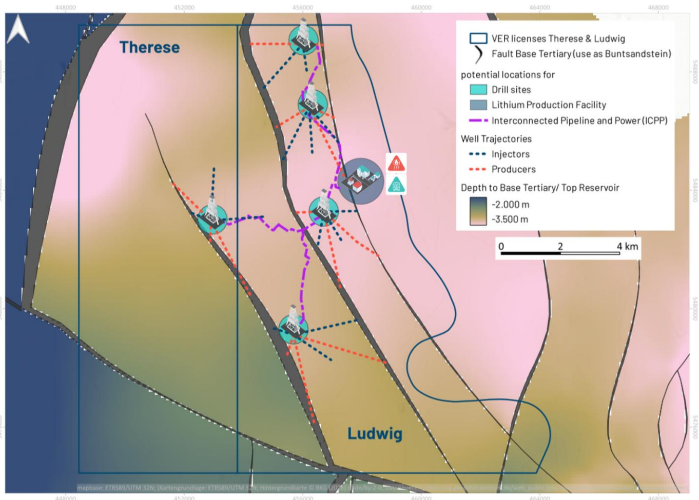
Figure 5 - Conceptual Field Development Plan for Project Ludwig
