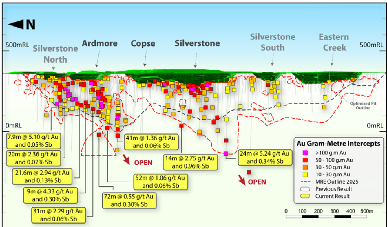
Long section through the Ricciardo deposit showing the locations of reported intervals.
