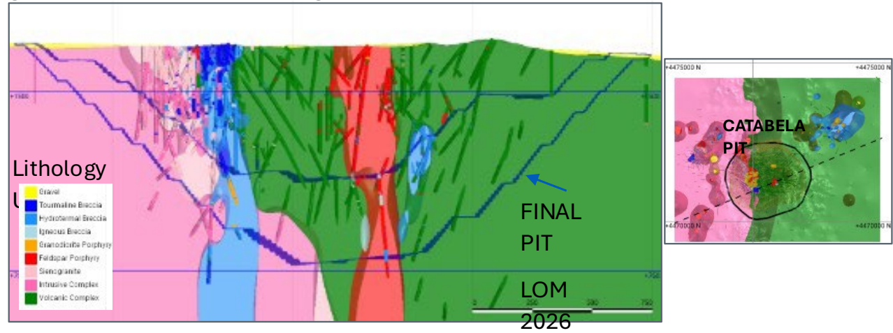
Figure 5. SW-NE Section of the Lithological Model
