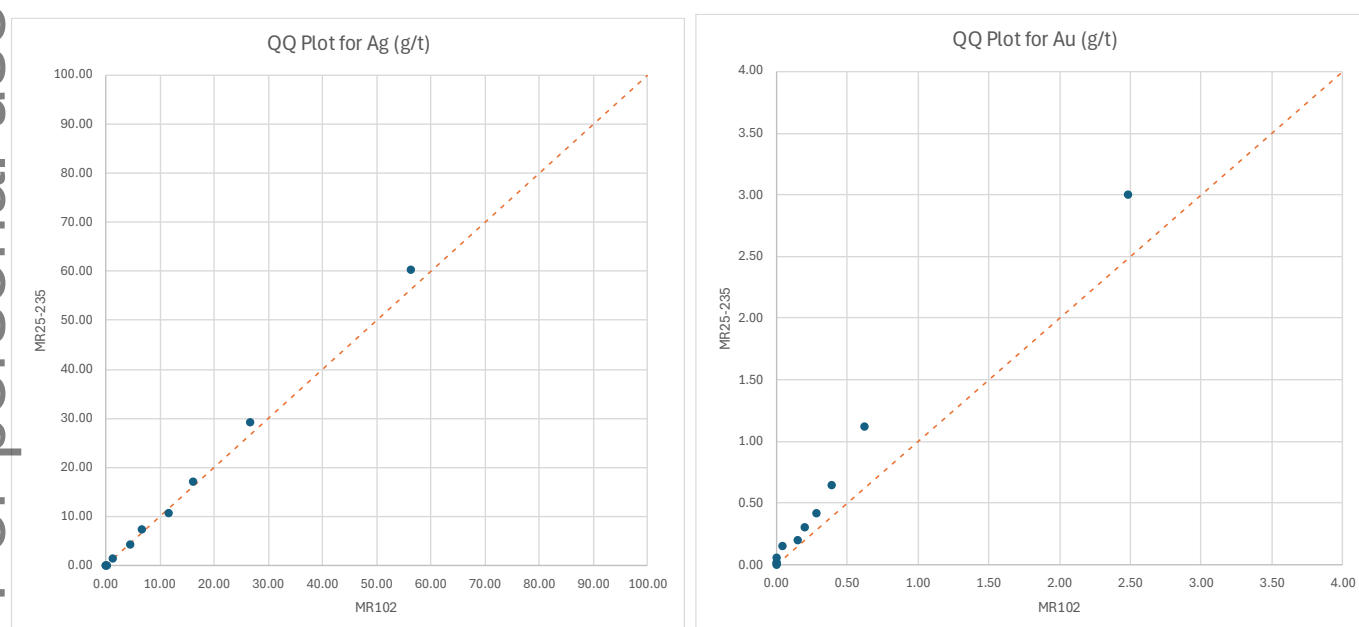
Figure 3: QQ Plots for gold and silver for twin hole MR25-235 (y) against historic drill hole MR102 (x).
