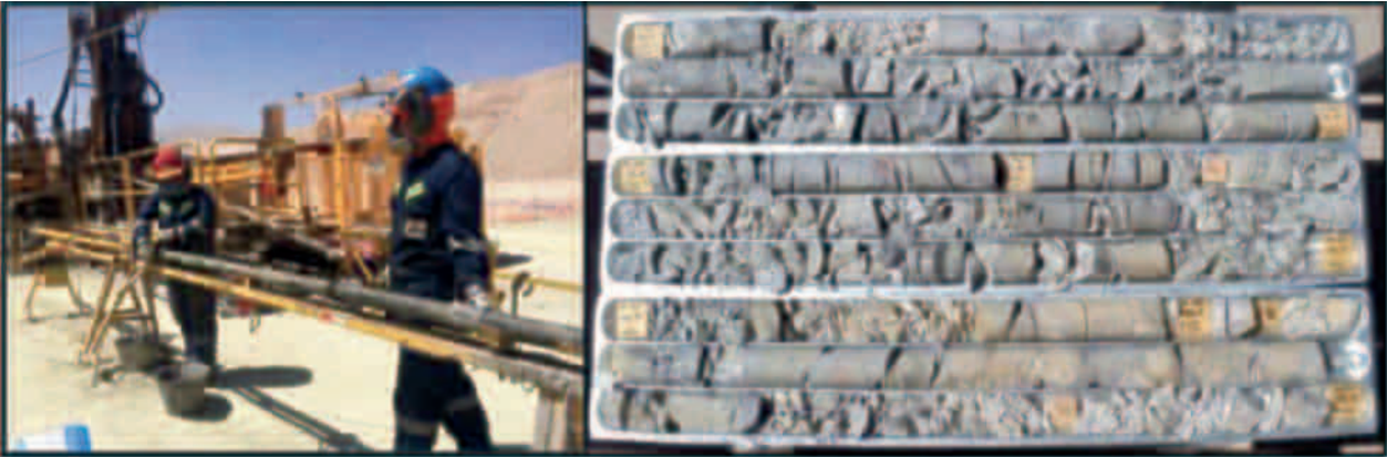
Figure 8-2: DDH Sampling; A) Sample Collection; B) Sample Distribution in Metallic Trays
