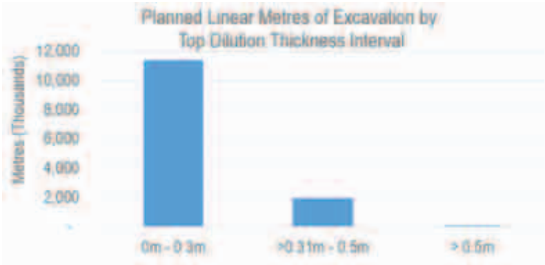
Figure 13-7: Histogram of planned linear metres to be excavated by top dilution thickness interval
