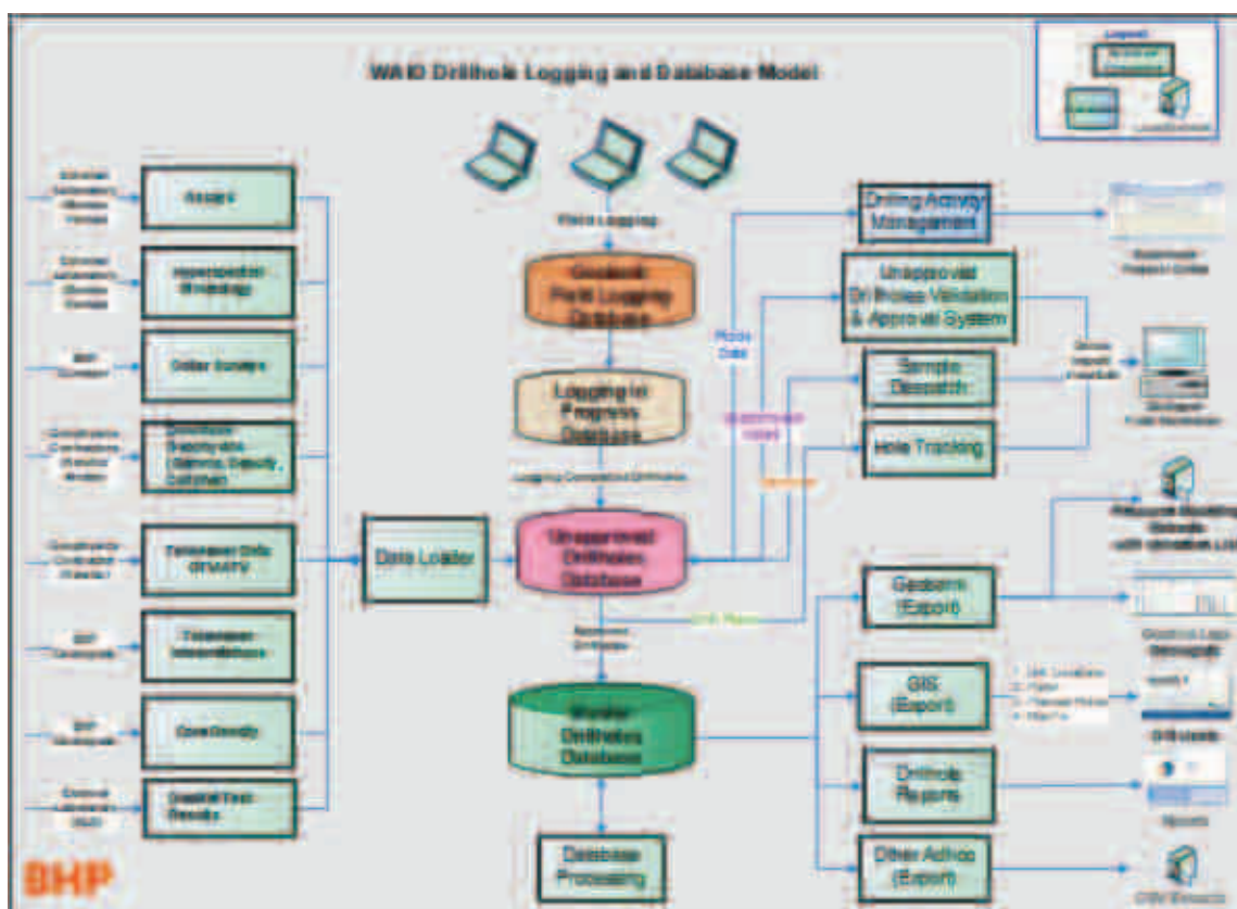
Figure 9-1: A Schematic Flowsheet of WAI0 Drill Hole Logging and Database Model
