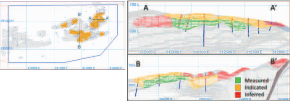
Note: Collar location, mineralisation wireframe (in grey); Indicated Mineral Resource (in orange) through a typical iron deposit
