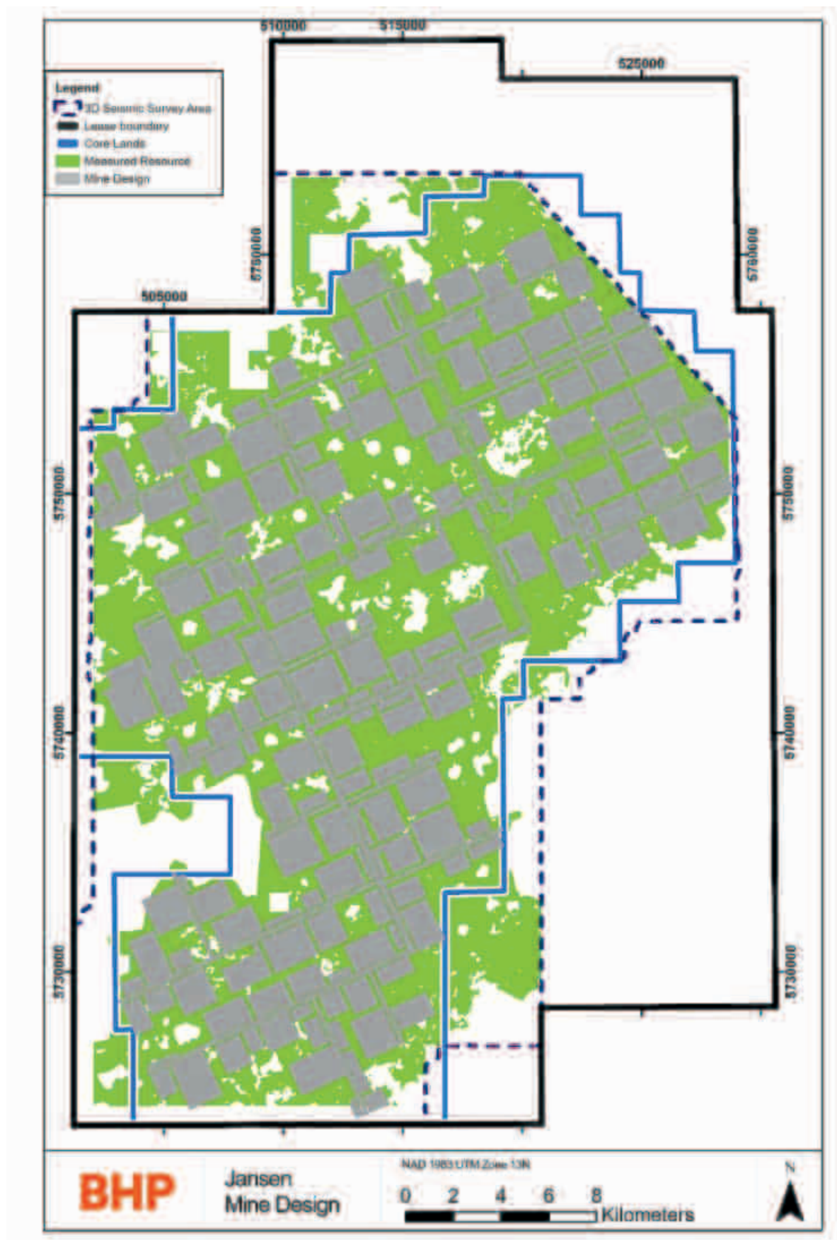
Figure 13-8: Jansen mine design.
