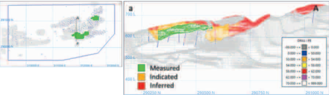
Note: Collar location, mineralisation wireframe (in grey); Measured Mineral Resource (in green) through a typical iron deposit.
