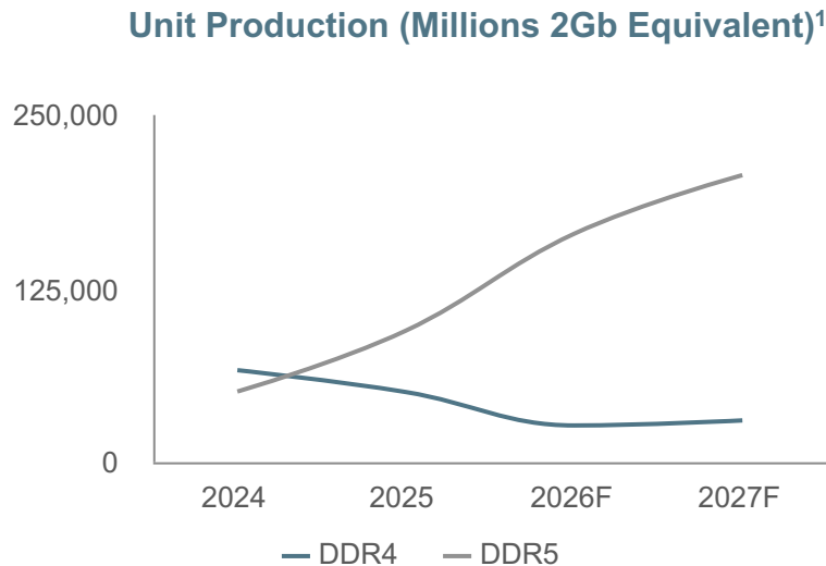
DDR4 VS DDR5 PRODUCTION
