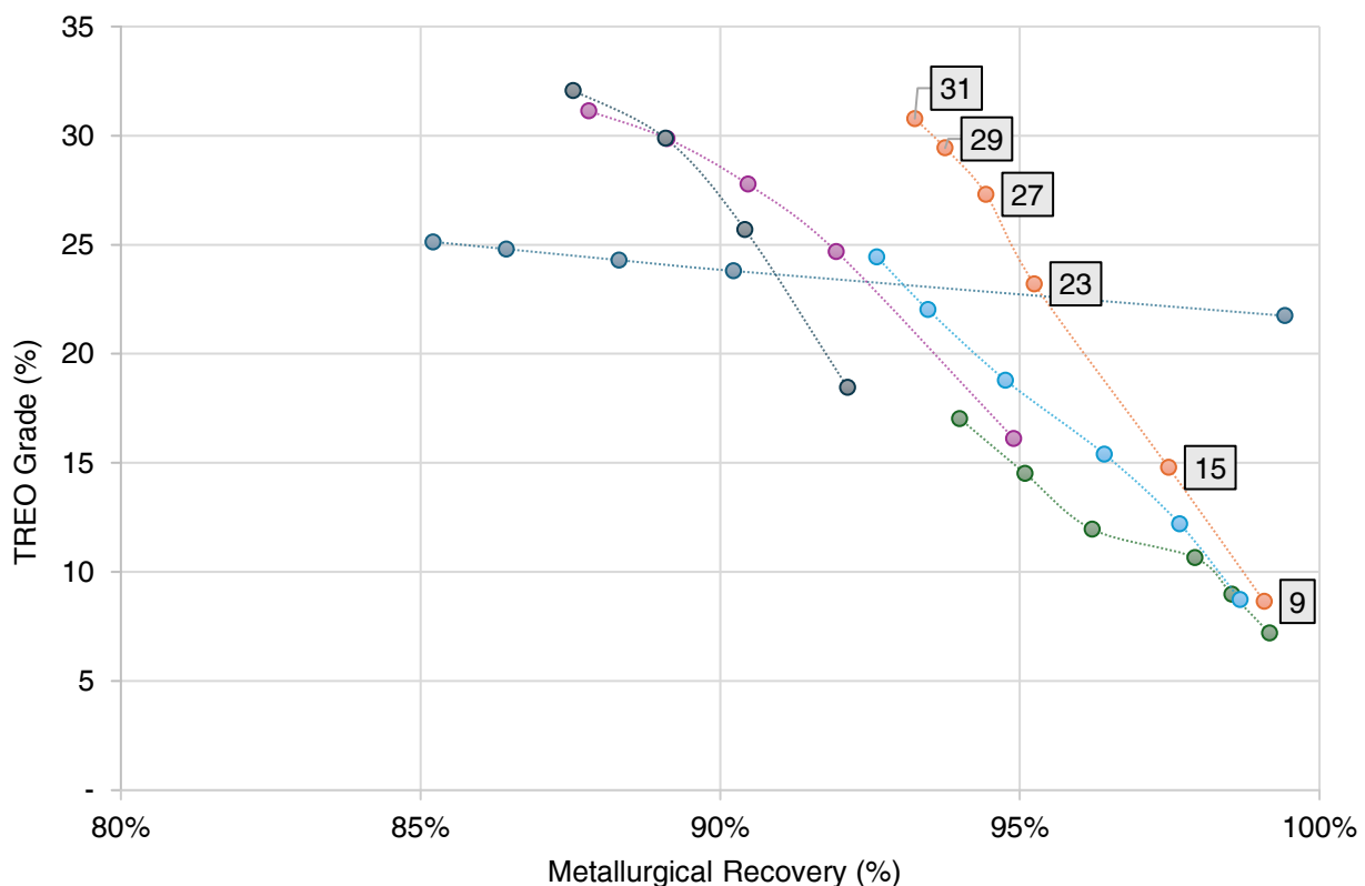
Figure 65: Sulista Weathered Flotation Grade-Recovery Curve
