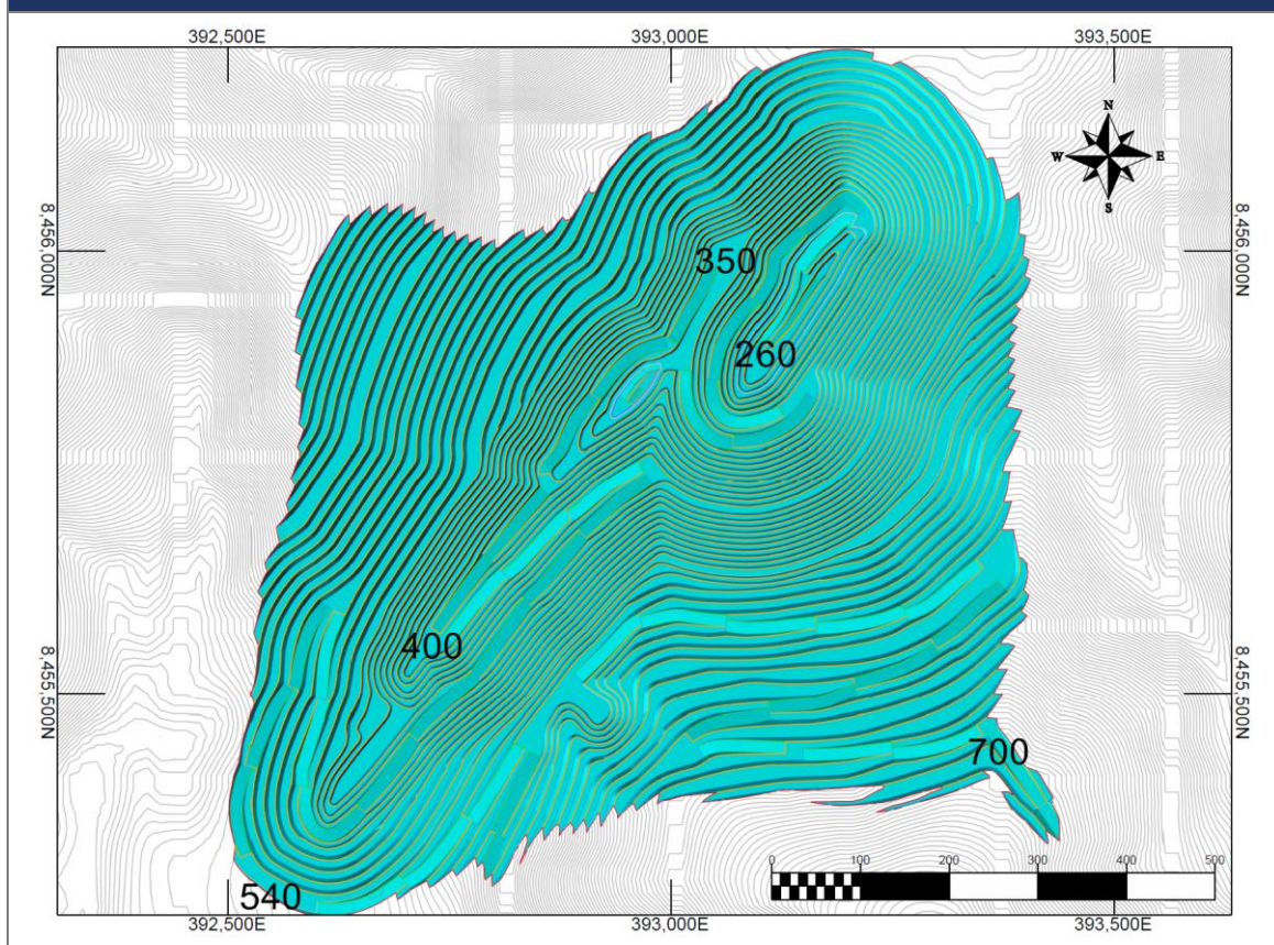
Figure 84: Sulista Final Pit Design
