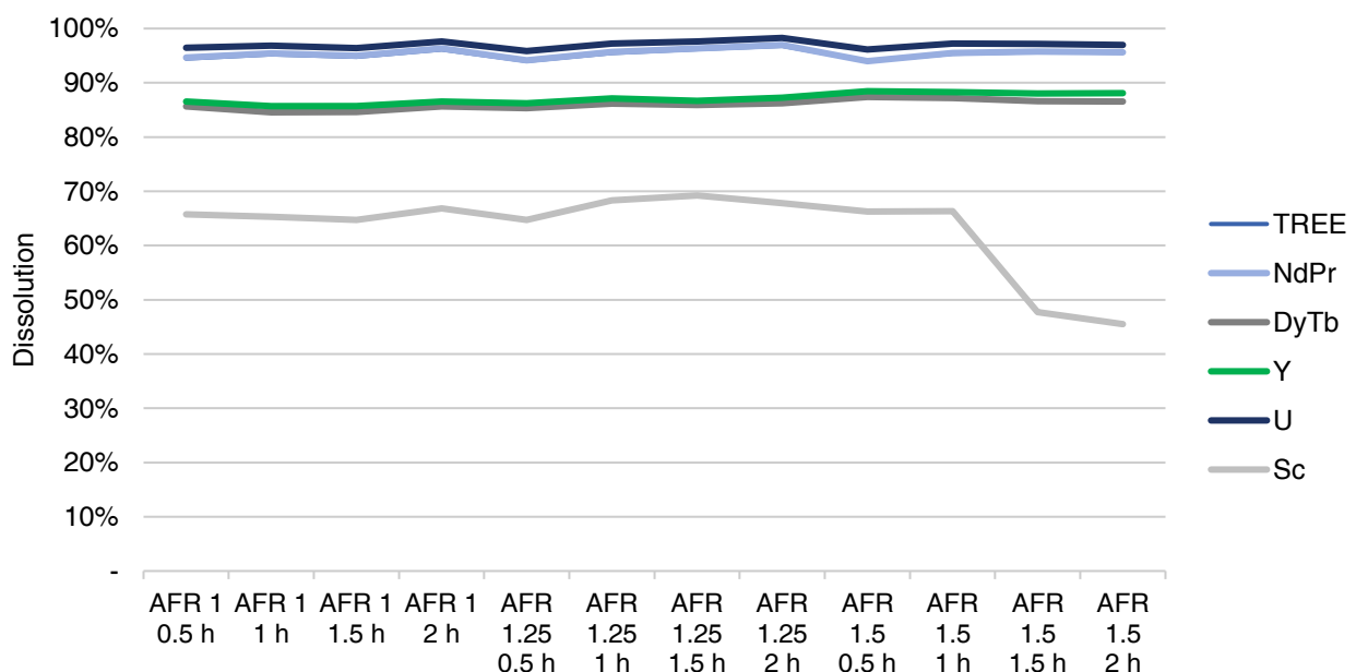
Figure 67: Effect of AFR and Digestion Time on Dissolution – Monte Alto CAB
