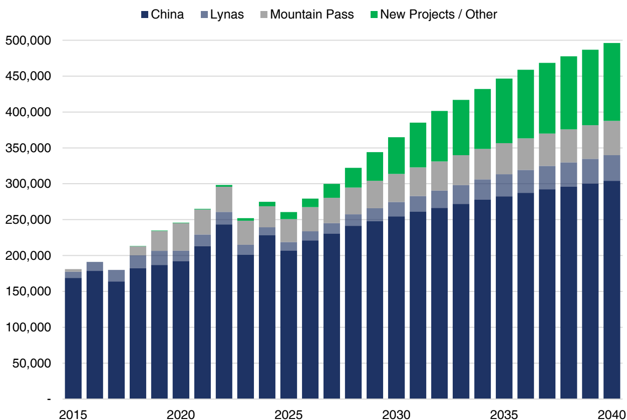
Figure 117: Global Rare Earths Supply by Source (tonnes of REO)
