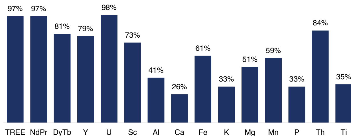
Figure 70: Scale-Up Extraction (AFR 1 – 1h) – Monte Alto CAB
