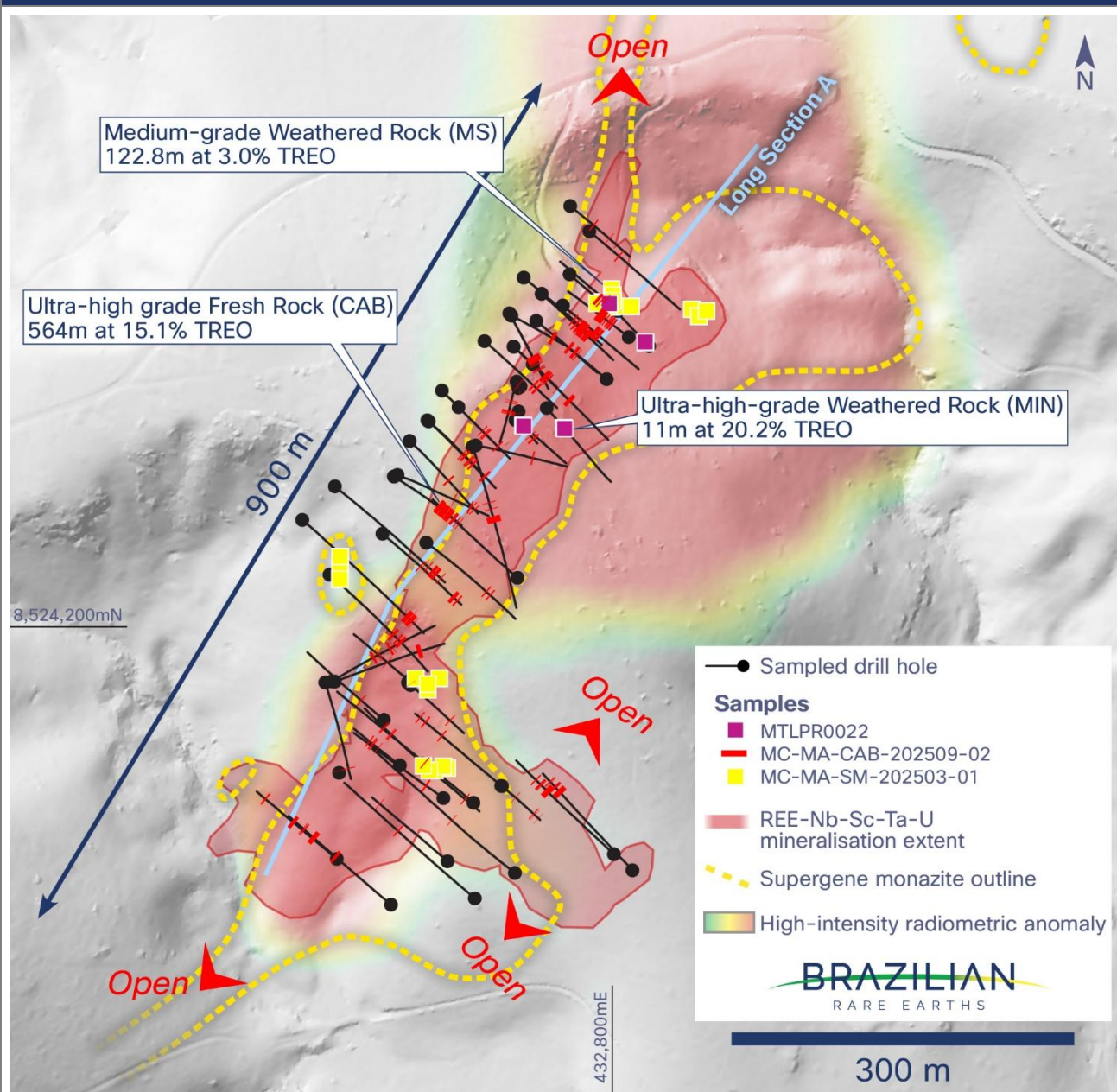
Figure 58: Monte Alto Plan View Showing Distribution of Metallurgical Samples
