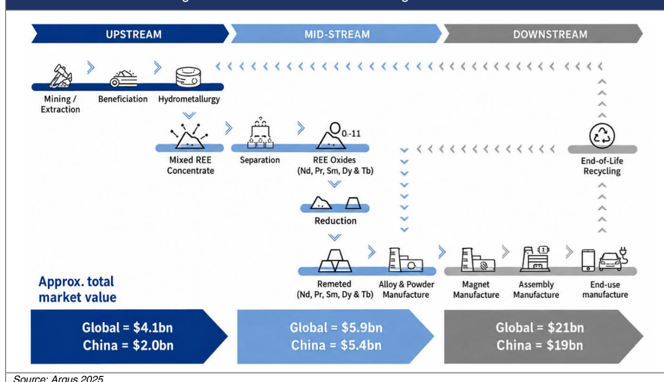
Figure 114: Rare Earth Permanent Magnet Value Chain
