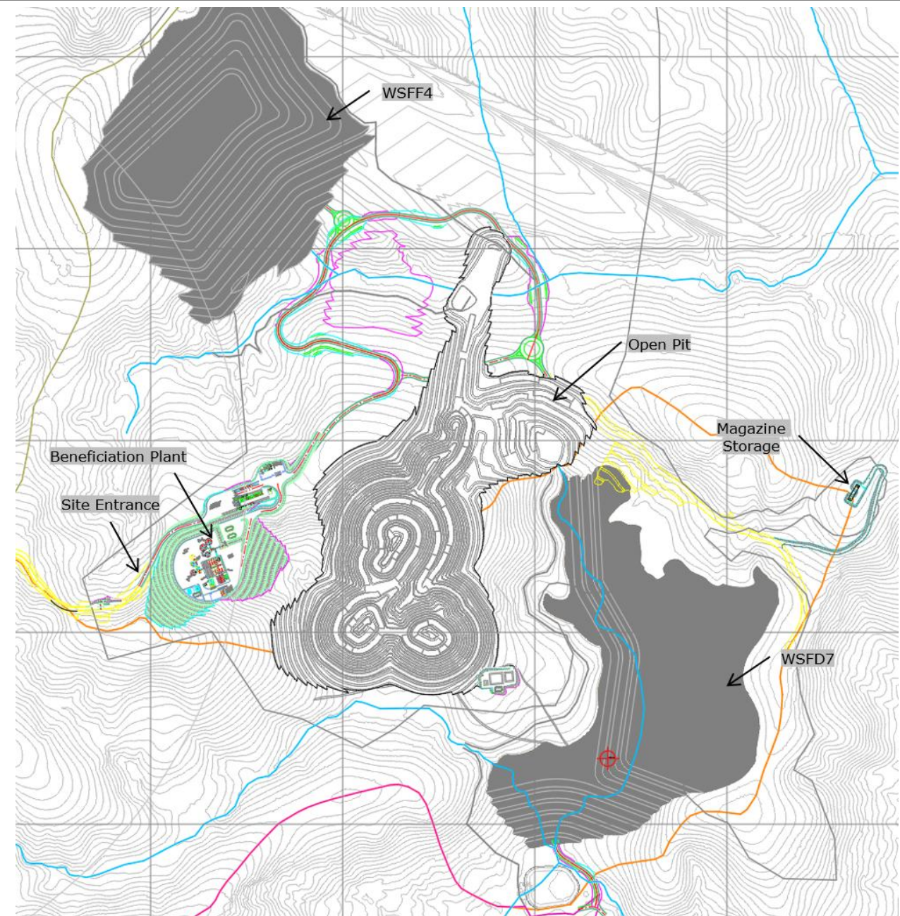
Figure 98: Monte Alto Site Overview
