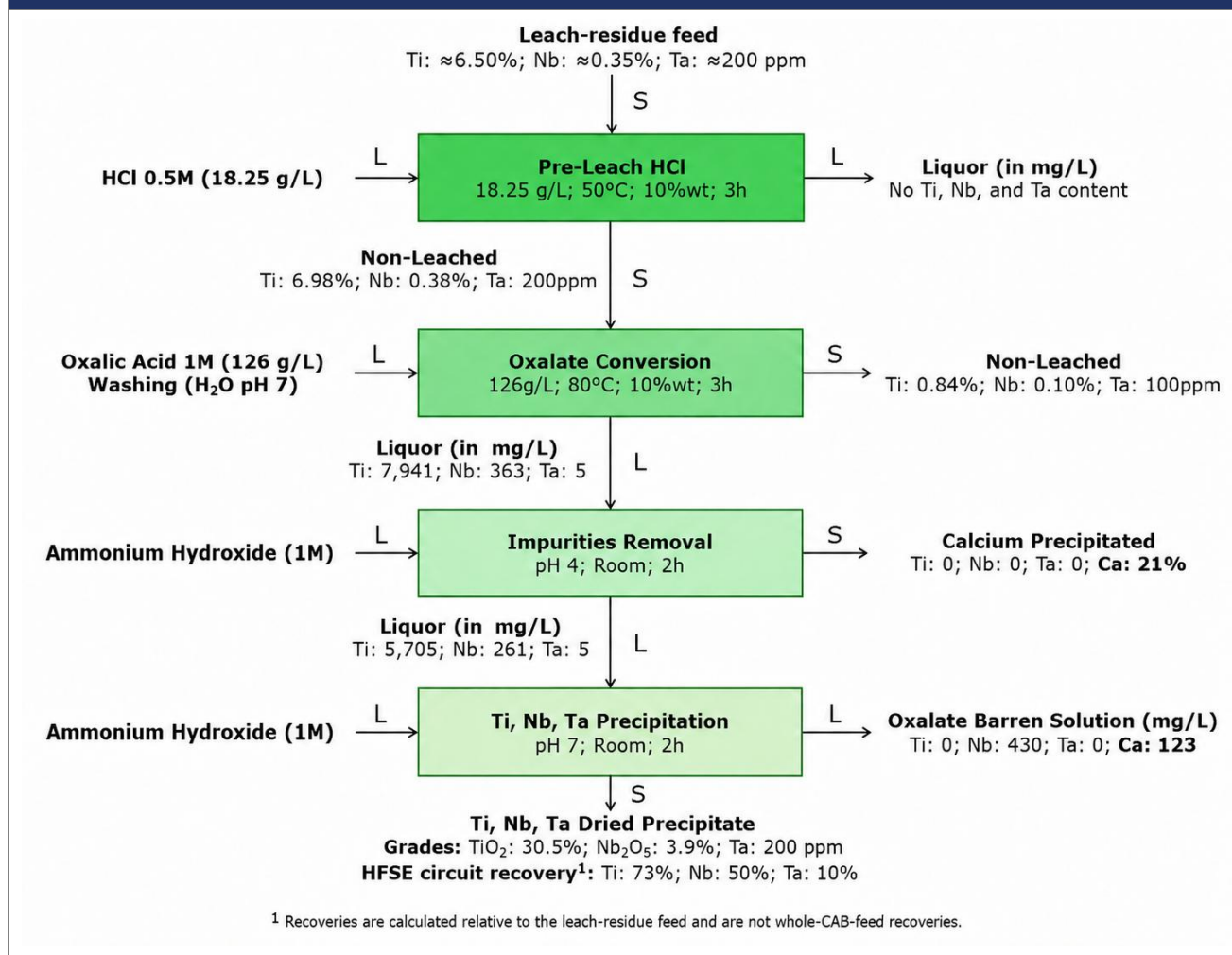
Figure 133: Indicative CAB Residue Recovery Circuit
