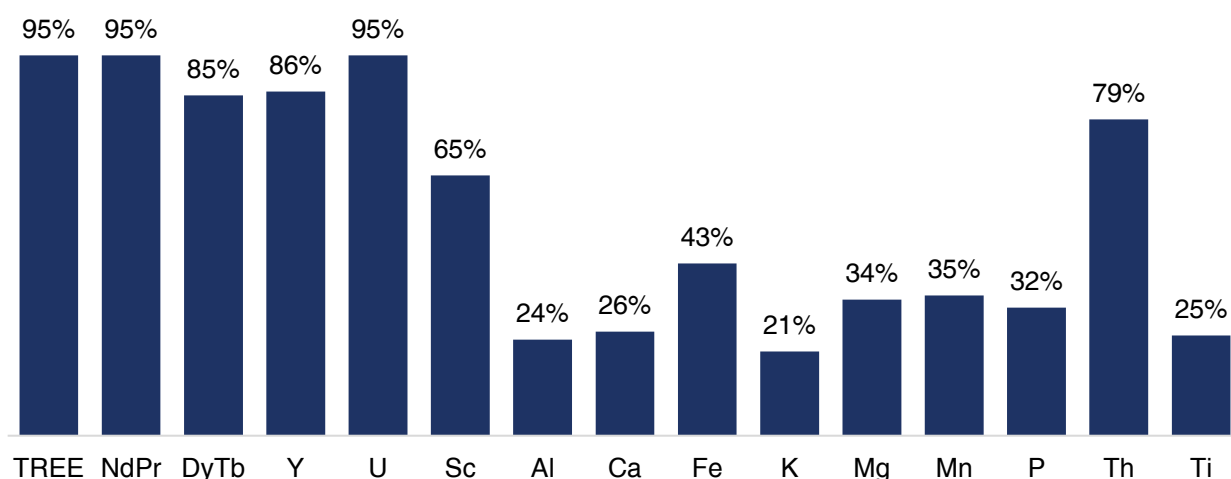
Figure 69: Bench Extraction (AFR 1 – 1h) – Monte Alto CAB
