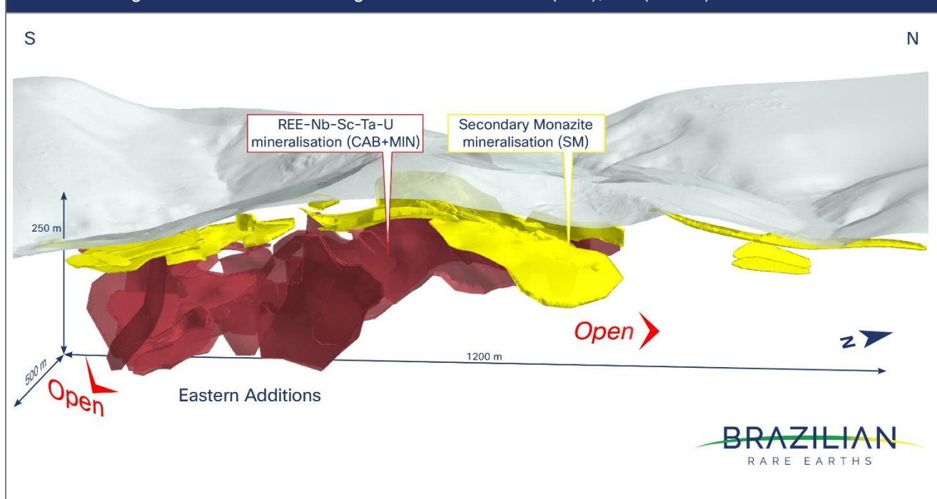
Figure 51: Monte Alto Geological Model. CAB+MIN (Red), SM (Yellow). View W/NW.
