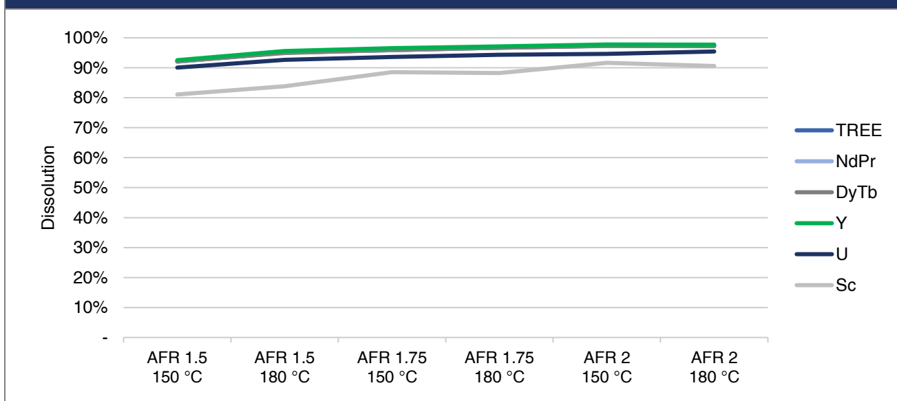
Figure 72: Effect of AFR and Temp. on Dissolution – Monte Alto MIN
