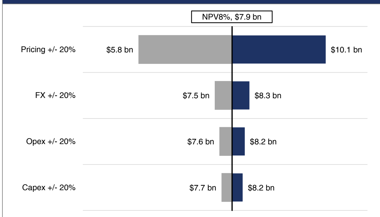
Figure 130: After-Tax NPV 8 (US$ bn), Argus EU/US Forecast
