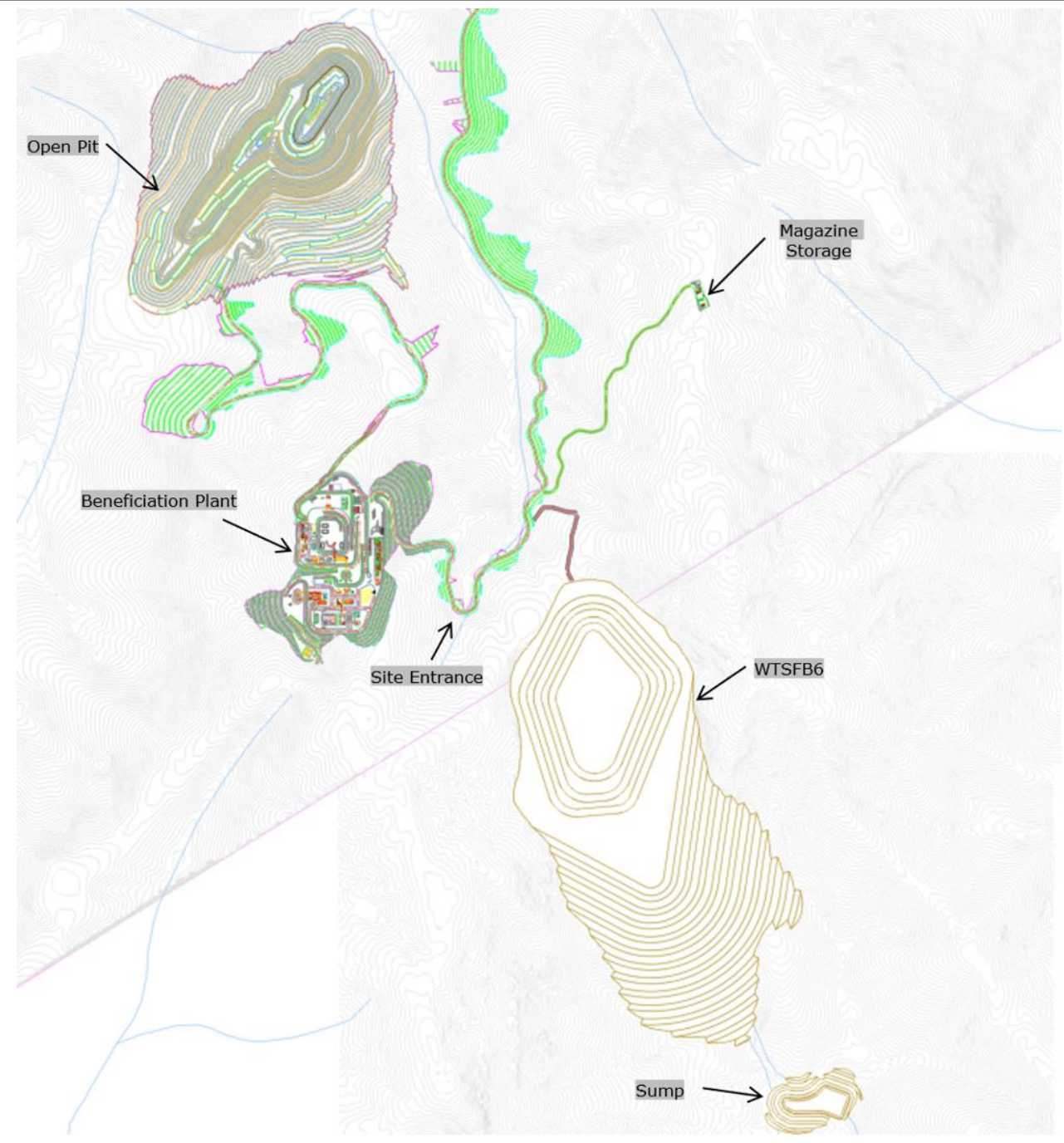
Figure 101: Sulista Site Overview
