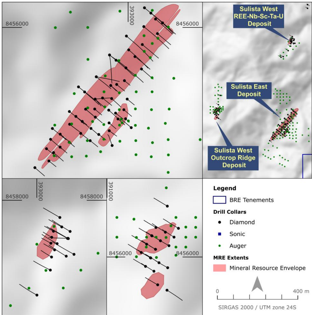
Figure 37: Sulista Drill Collar Location Map
