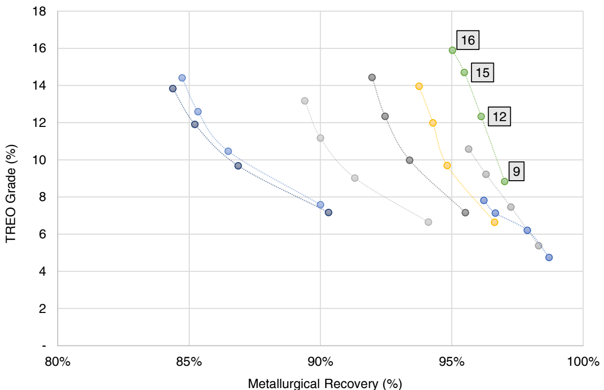
Figure 66: Sulista Fresh Rock Flotation Grade-Recovery Curve
