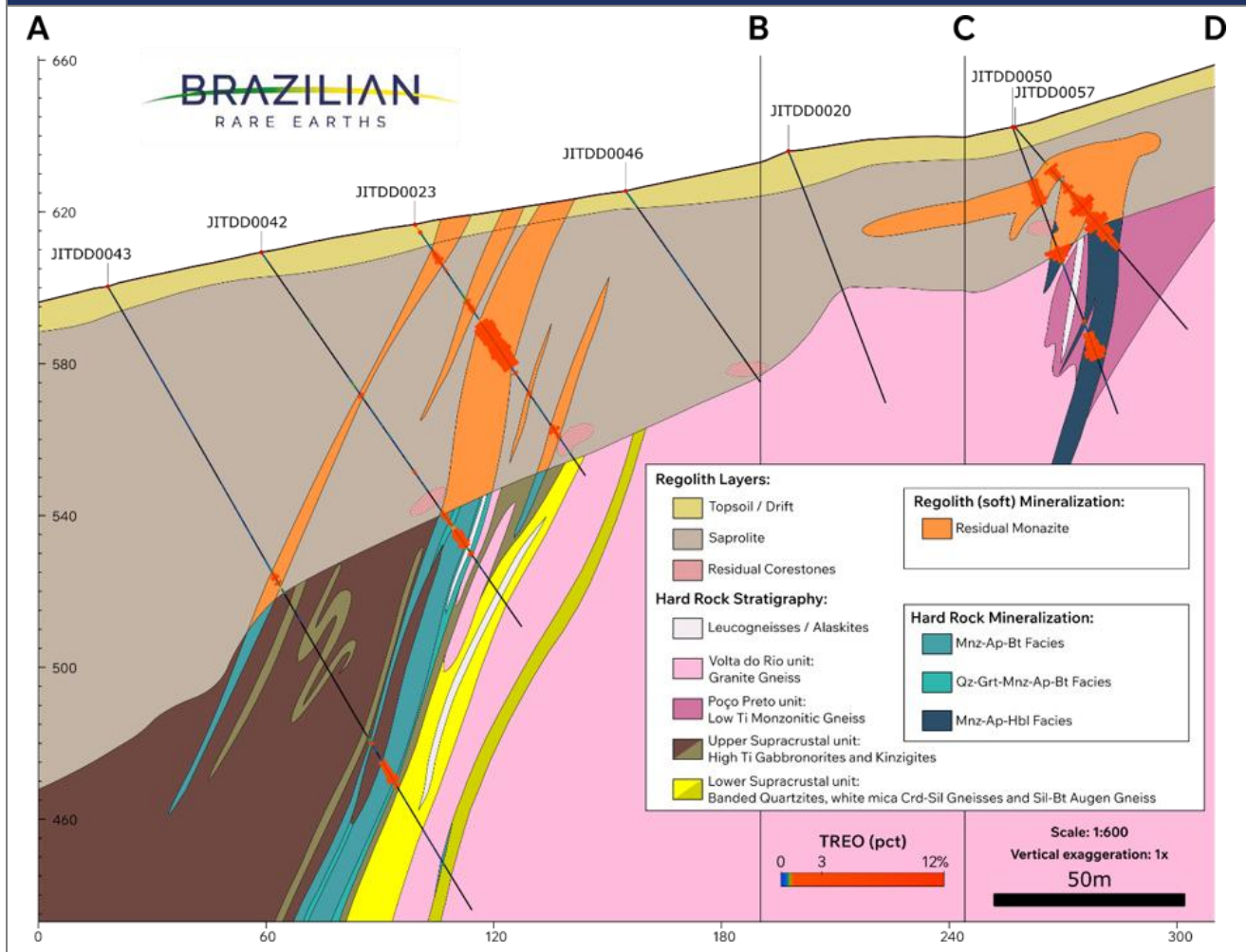
Figure 25: Cross Section of Sulista East Deposit
