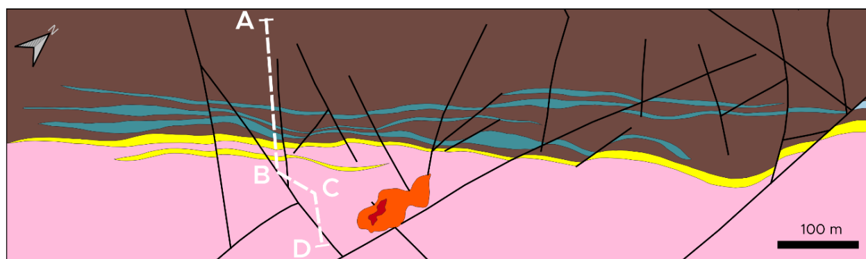
Figure 24: Simplified Geological Map of Sulista East
