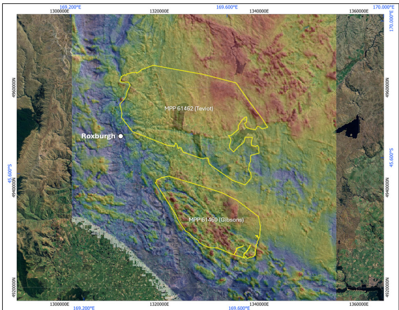
Figure 6. Otago prospecting permits over regional magnetic (TMI-RTP).
