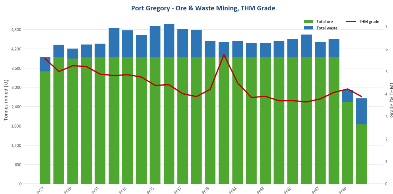
Figure 7: Total ore and waste mined, and THM grade, by year
