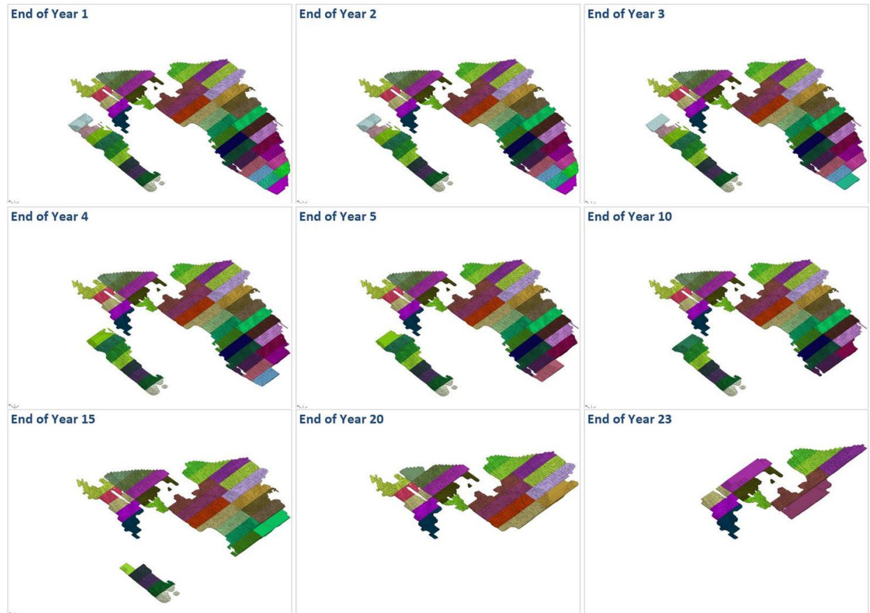
Figure 9: Pit progression, end of year 1 to year 23
