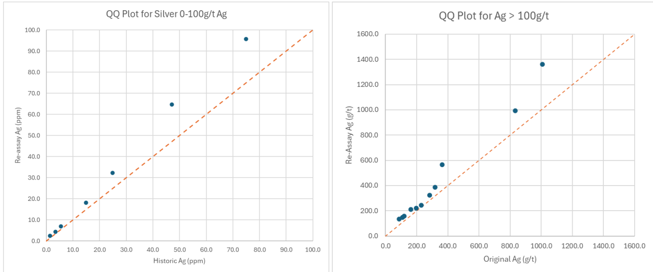
Figure 4: Percentile analysis for silver between Original data set and Re-assays from 0-100g/t Ag and >100g/t Ag
