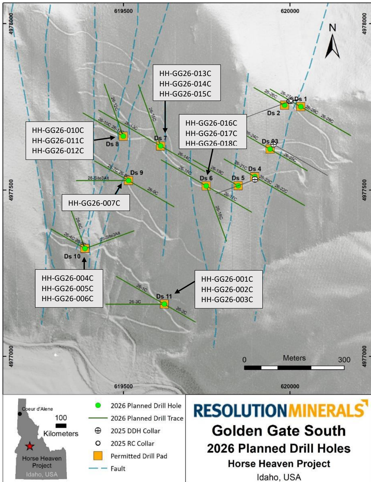
Figure 4: Golden Gate South 2026 Drill targets with drillhole numbers and drill sites (Inset).
