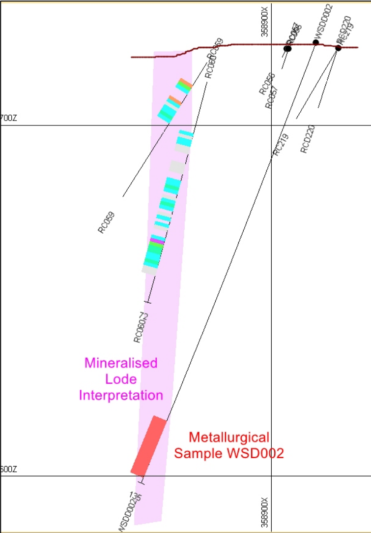
Section looking North. The section for WSD007 is similar. The colours on the drill traces indicate mineralised intervals. The metallurgical sample composited the entire mineralised interval.
