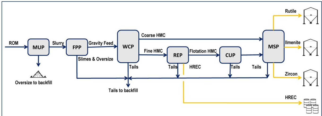
Figure 8-5: Proposed Flowsheet Based on Metallurgical Testwork
