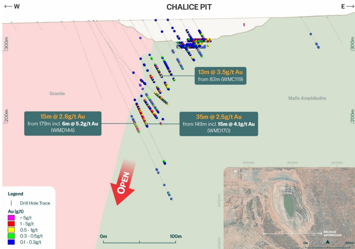
Figure 6: Kronos 6478650mN – Cross Section
