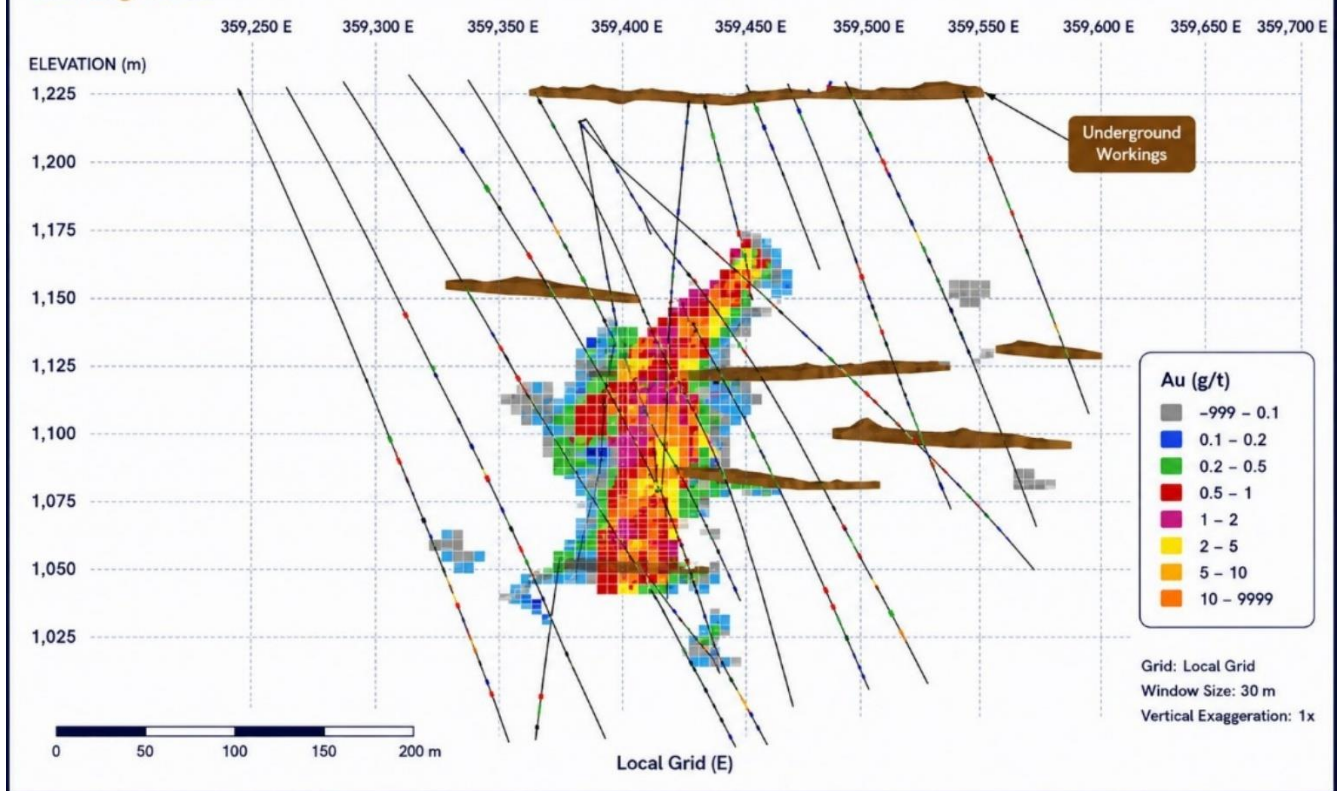
Figure 7: Long(top) and Cross(bottom) Section of the Block Estimates
