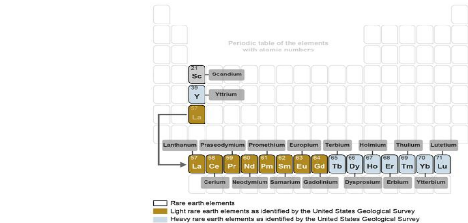
Figure 8.1: Rare earth elements in the periodic table of elements
