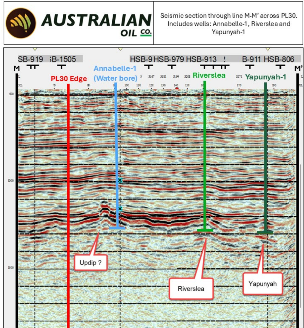
Figure 2 arbitrary seismic cross section line through the 1984 Riverslea-Yapunyah 3D seismic survey acquired by Hematite Petroleum Pty Ltd
