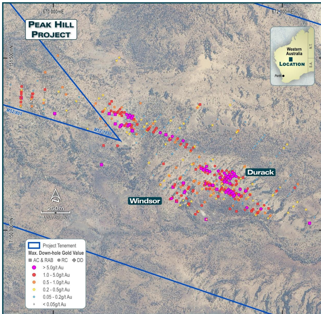
FIGURE 16: DURACK AND WINDSOR. WINDSOR IS THE LESS-DRILLED AREA IMMEDIATELY SOUTHEAST OF THE CENTRAL CLUSTER OF +5G/T RC HOLES.
