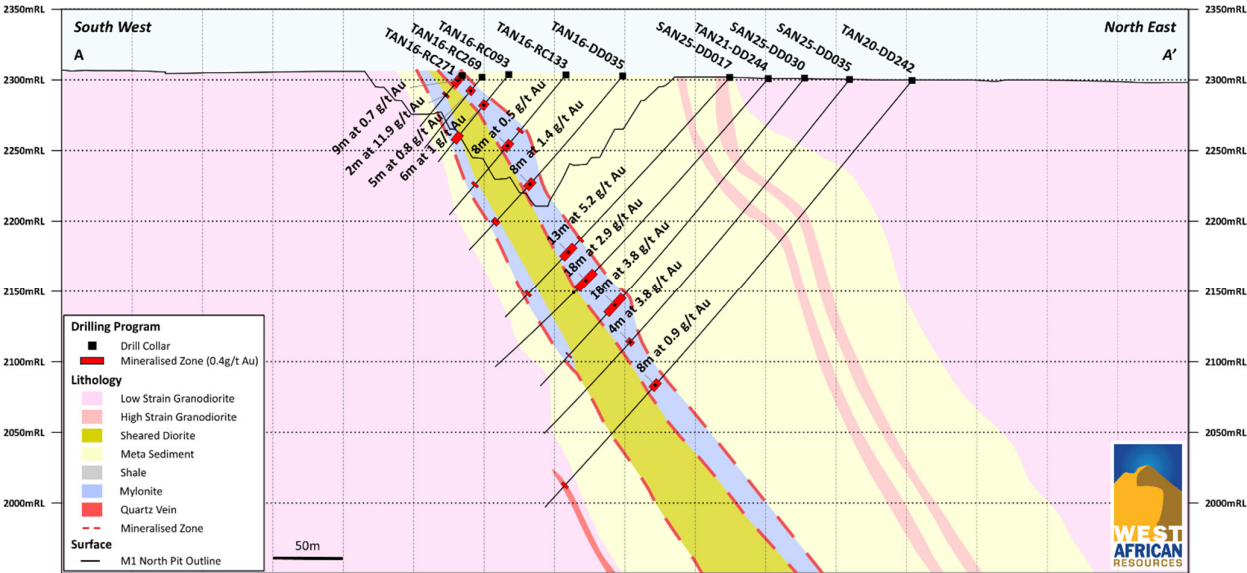
Cross Section of M1 North Drilling
