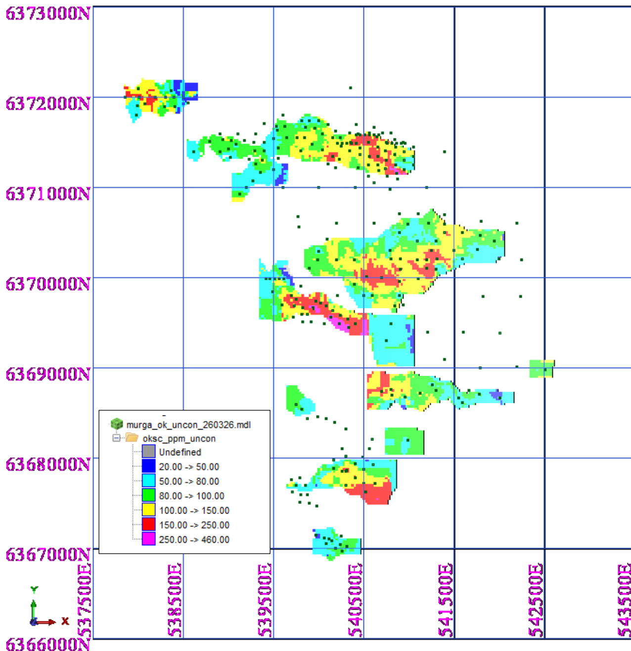
Murga Global Block Grade Distribution for Scandium
