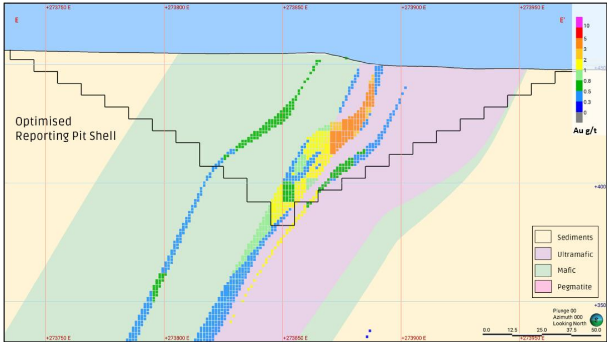
Figure 9 – Cross section E-E' Looking North at Macedon showing lithology, block model grades (g/t) and the Optimised Reporting Pit Shell.
