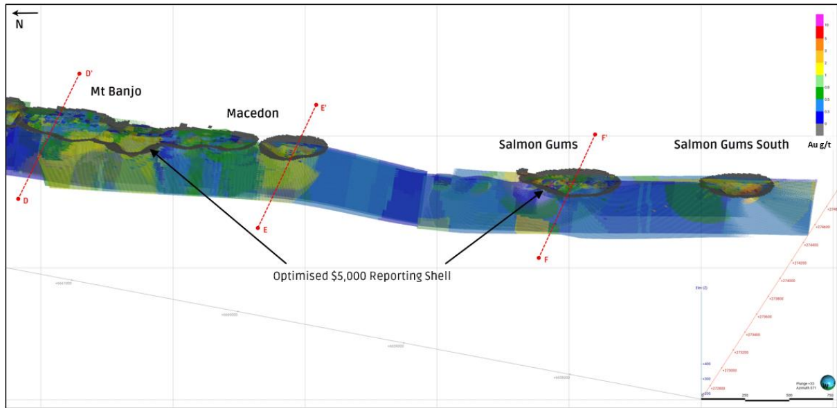
Figure 7 – Oblique View (looking East) of Mt Banjo, Macedon and Salmon Gums block model grades (g/t) with mined pit shapes and Optimised Reporting Pit shells.
