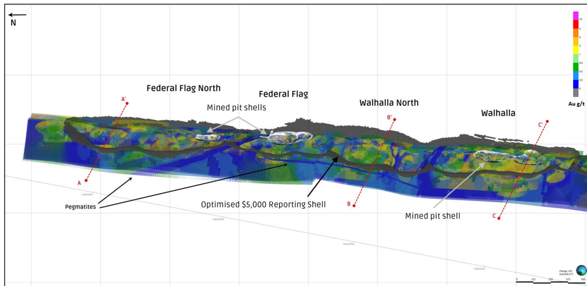
Figure 3 – Oblique View (looking East) of Walhalla and Federal Flag block model grades (g/t) with mined pit shapes and Optimised Reporting Pit shells.
