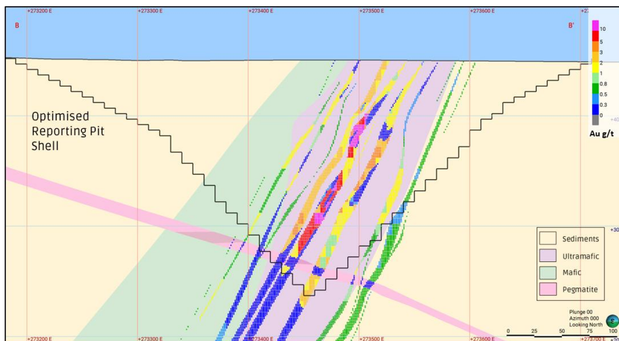
Figure 5 – Cross section B-B' looking North at Walhalla North showing lithology, block model grades (g/t) and the Optimised Reporting Pit Shell.
