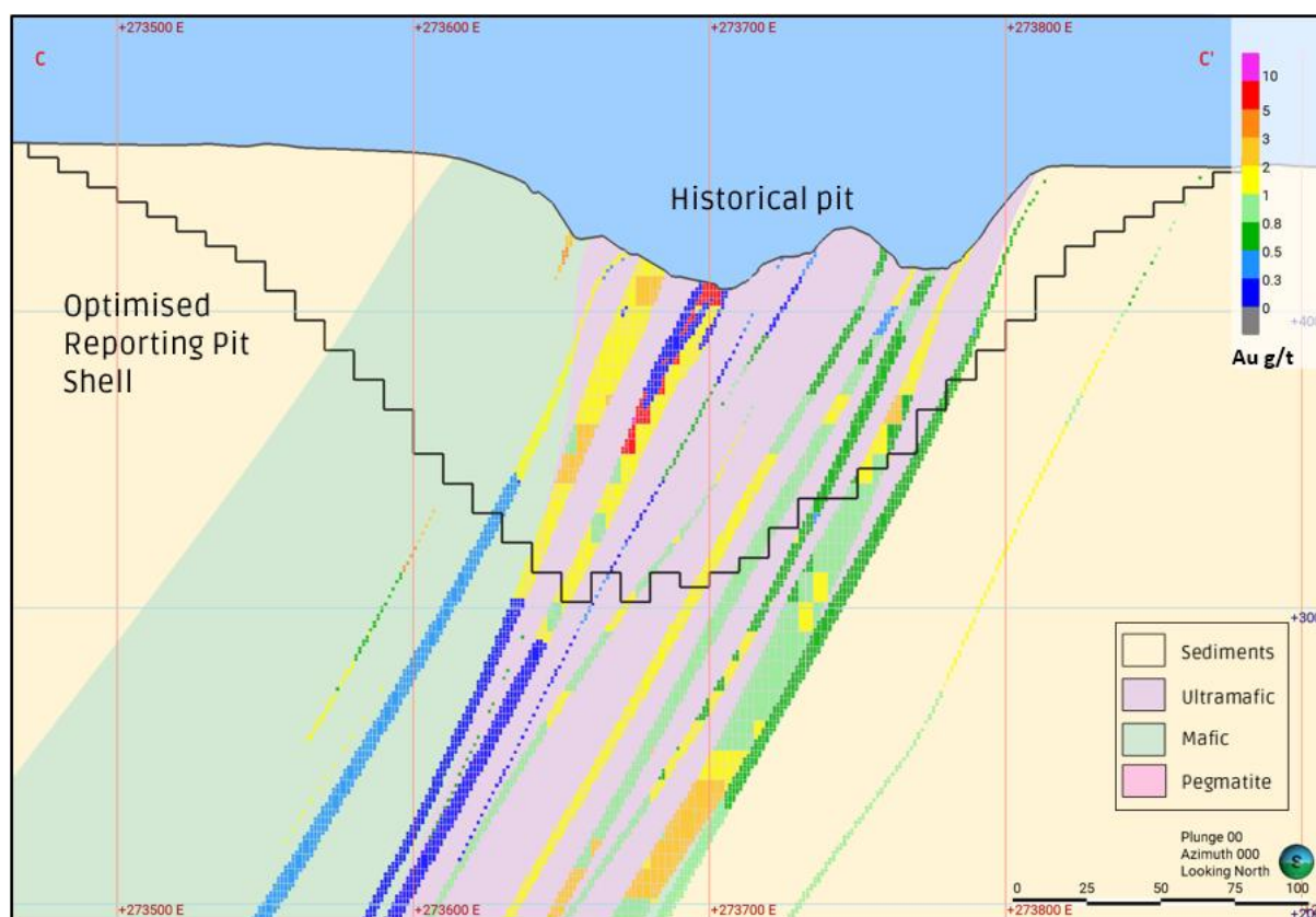
Figure 6 – Cross section C-C' looking North at Walhalla under the current pit, showing lithology, block model grades (g/t) and the Optimised Reporting Pit Shell.
