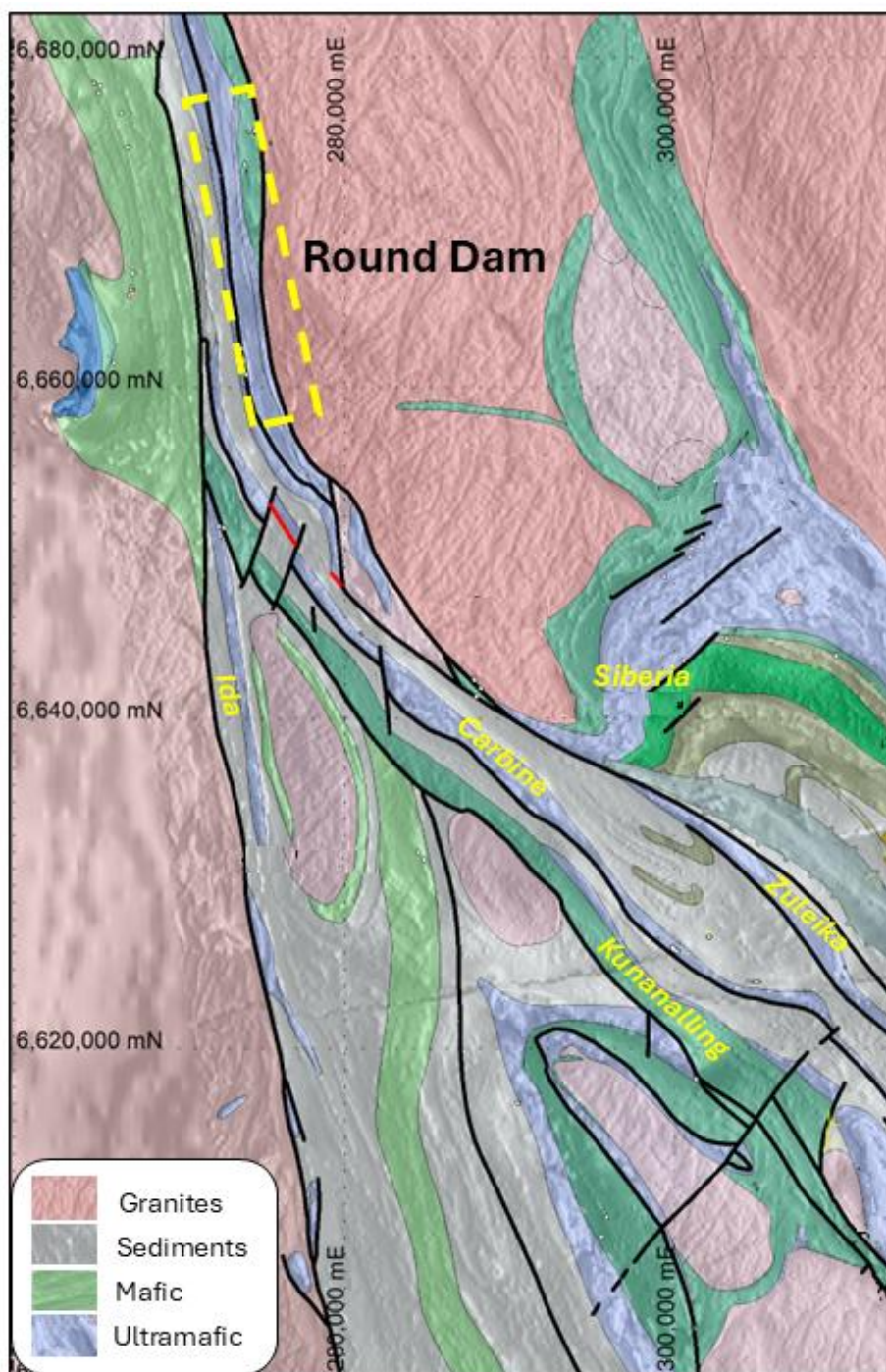
Figure 12 – Regional Geology showing proximity of major regional structures to Round Dam
