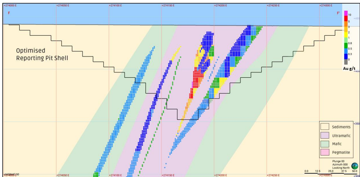
Figure 10 – Cross section F-F' Looking North at Salmon Gums showing lithology, block model grades (g/t) and the Optimised Reporting Pit Shell.
