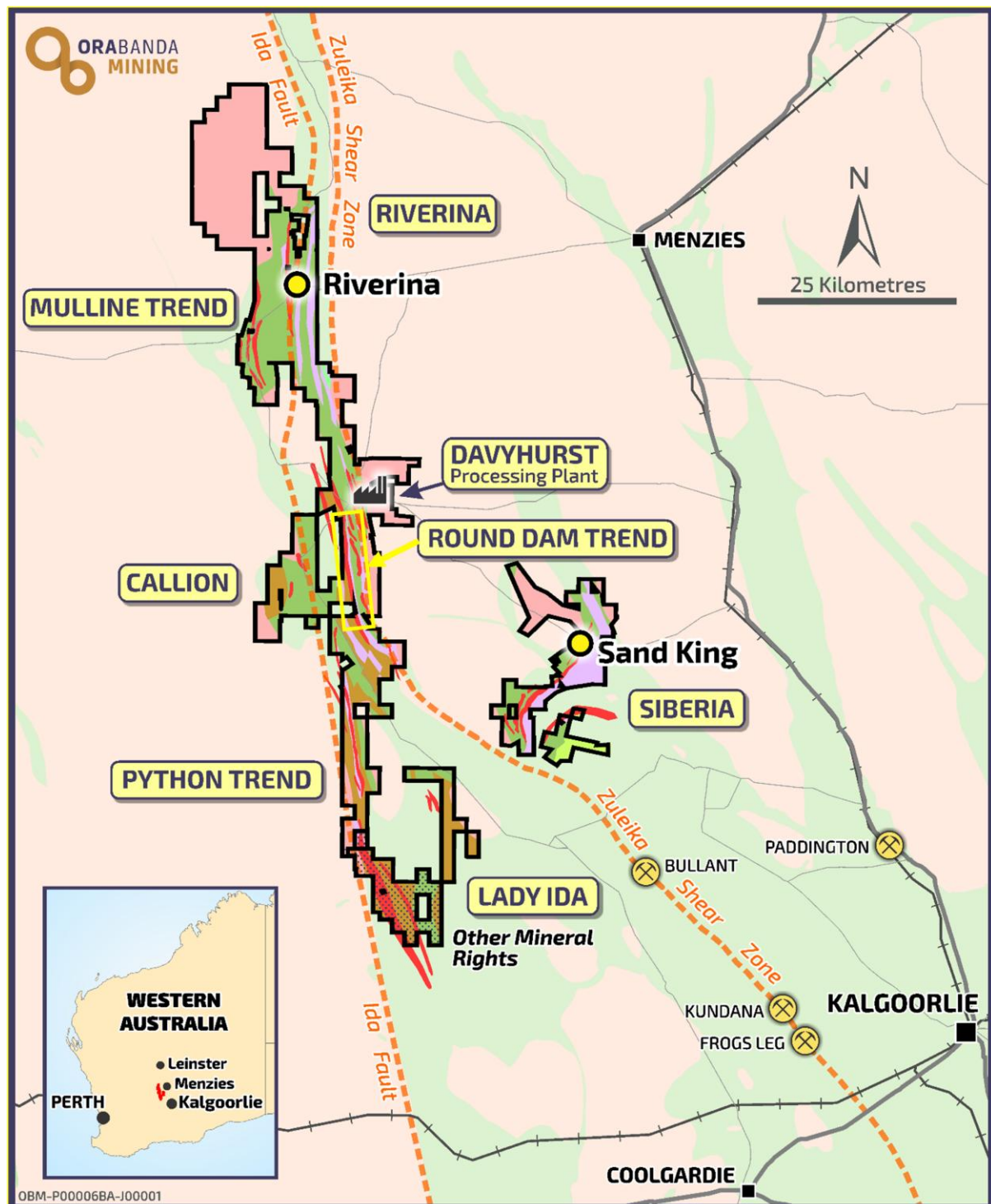
Figure 11 - Regional map, OBM tenements and deposits
