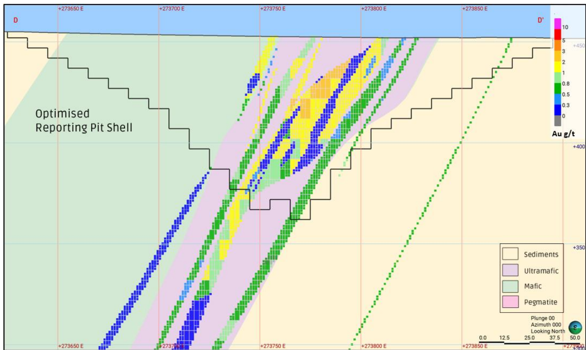
Figure 8 – Cross section D-D' Looking North at Mt Banjo showing lithology, block model grades (g/t) and the Optimised Reporting Pit Shell
