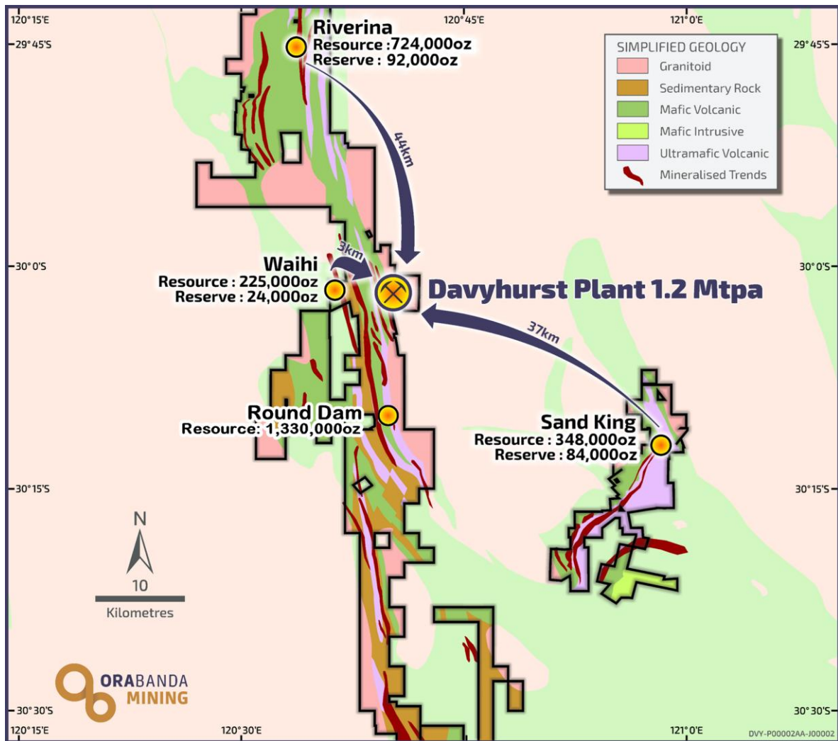
Figure 1 - Deposit locations
