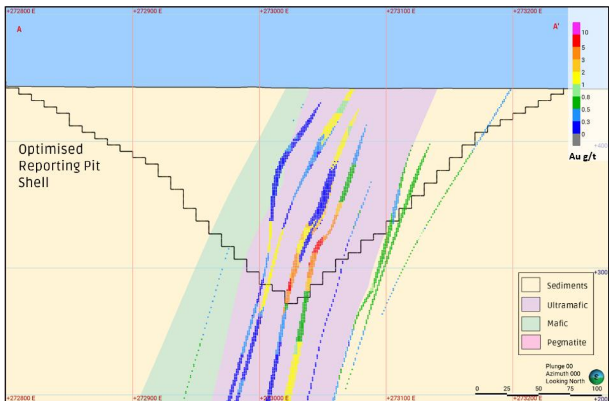
Figure 4 – Cross section A-A' looking North at Federal Flag North showing lithology, block model grades (g/t) and the Optimised Reporting Pit Shell.
