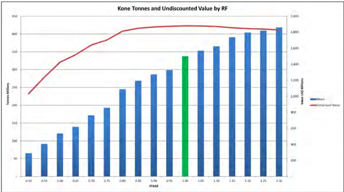
Figure 2.15: Koné pit optimisation results
