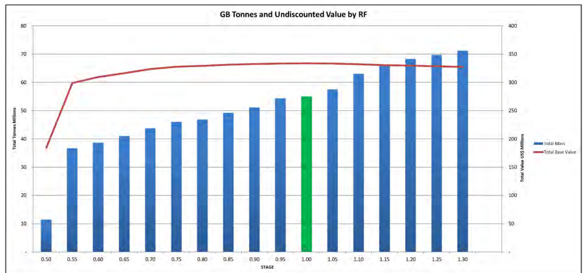
Figure 2.16: Gbongogo pit optimisation results
