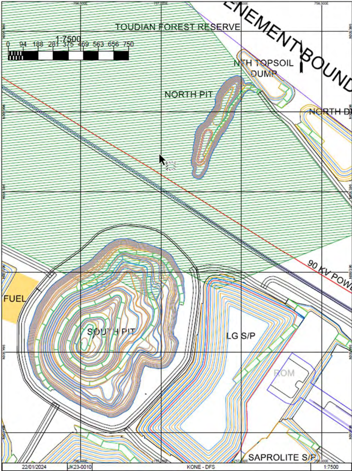
Figure 2.17: Koné South and North pit designs
