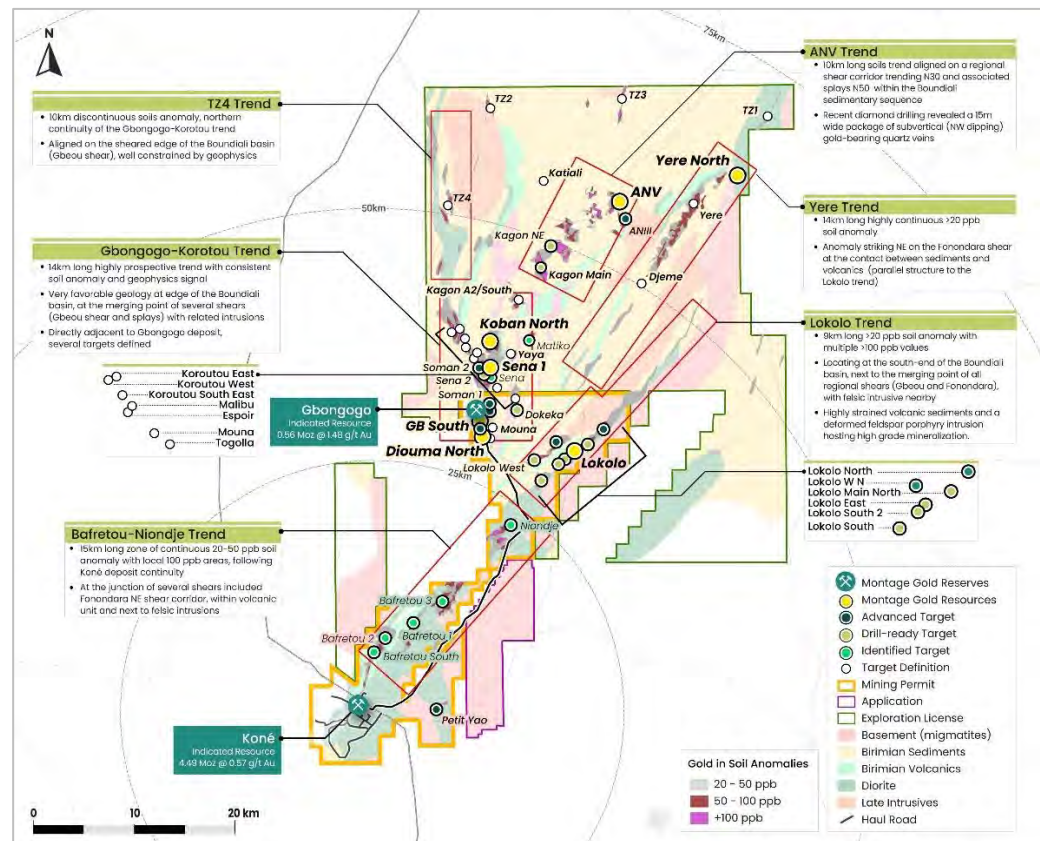
Figure 6. Koné Project geological trend and exploration target map.
