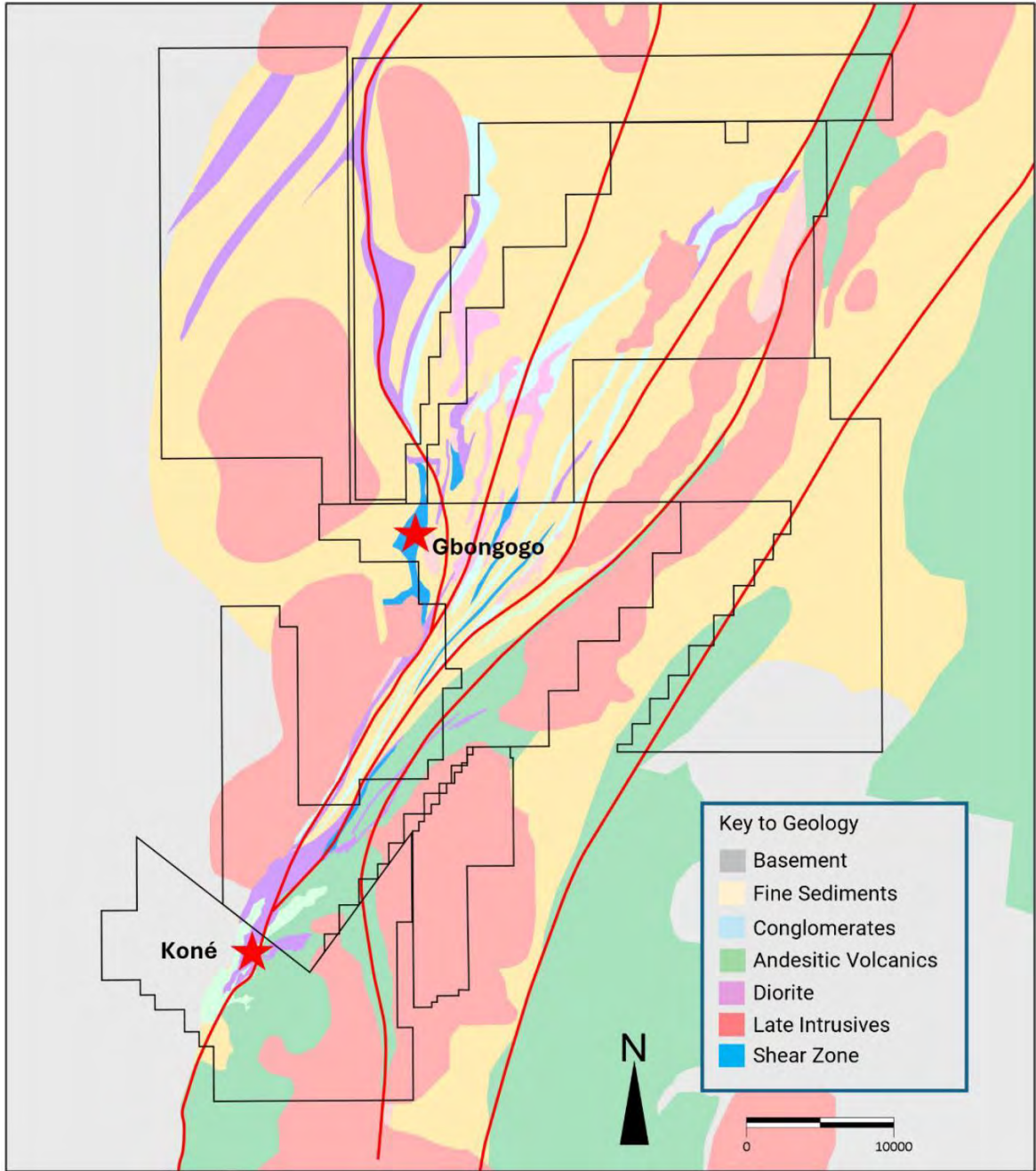
Figure 2.3: Koné Gold Project geology (includes Koné and Gbongogo)
