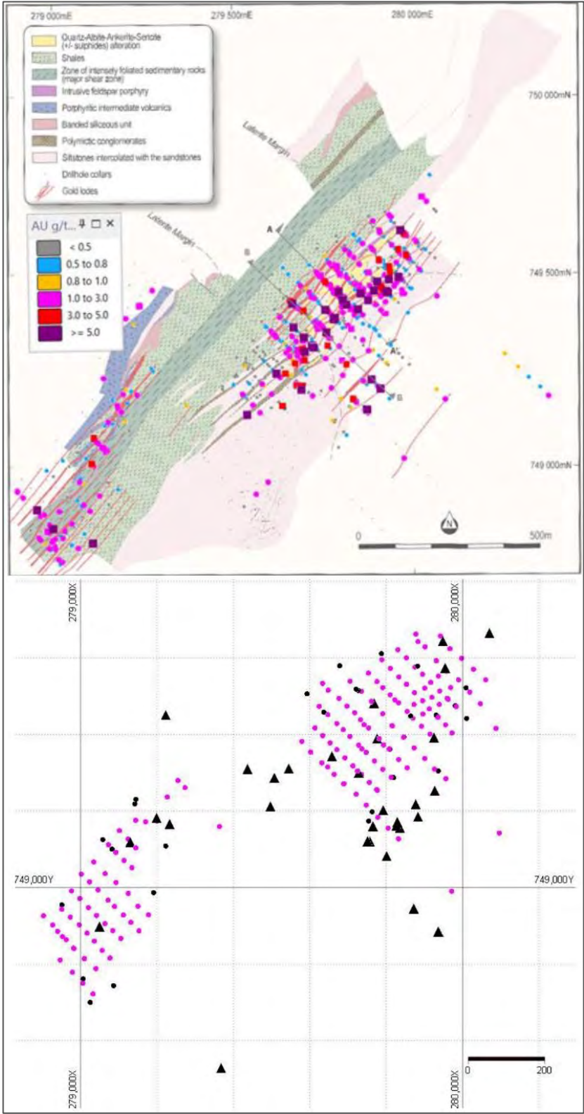
Figure 3.2: Blaffo Guetto drilling
