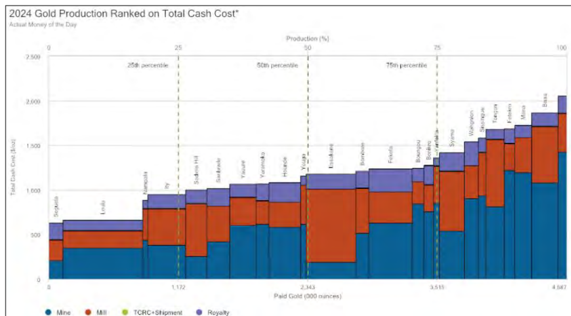
Figure 2.21: Central West African gold producers cash cost curve – 2024
