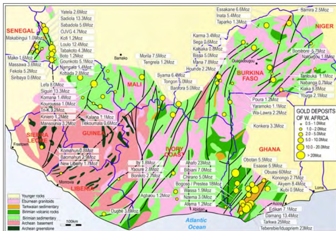
Figure 2.2: West African Craton – main tectonic elements
