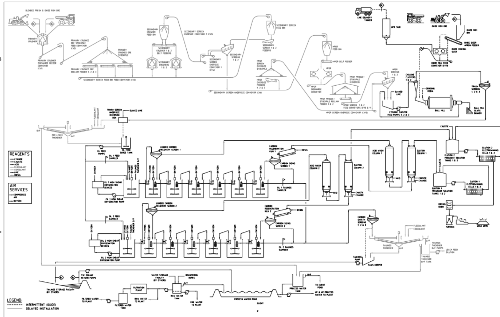
Figure 2.31: Summary process flow diagram
