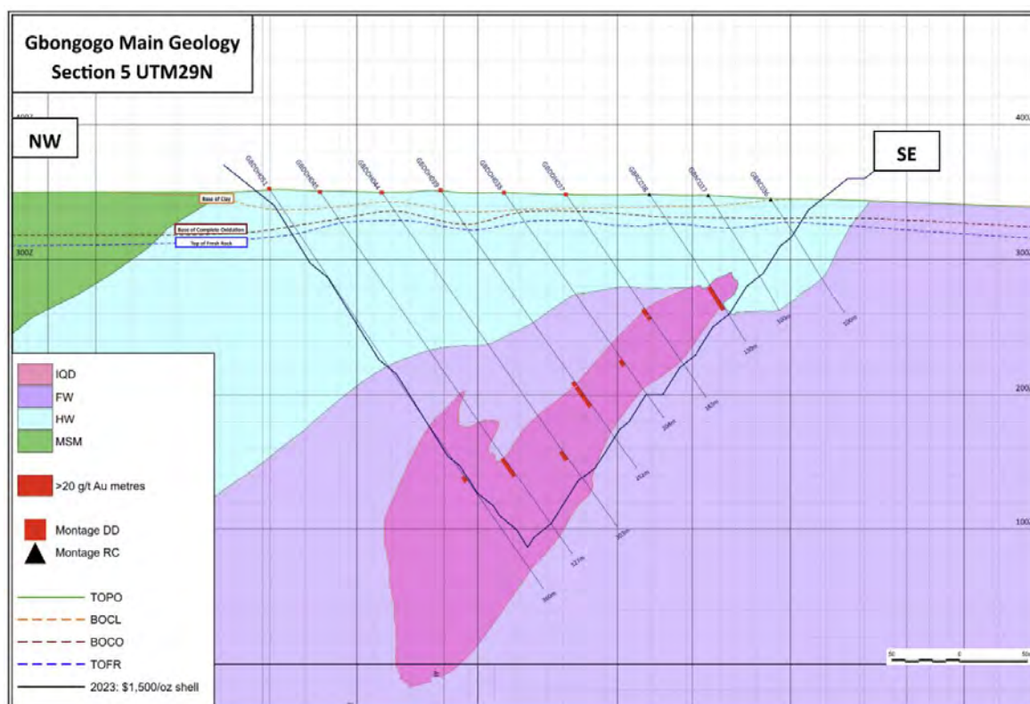
Figure 2.5: Cross section through Gbongogo (looking northeast)
