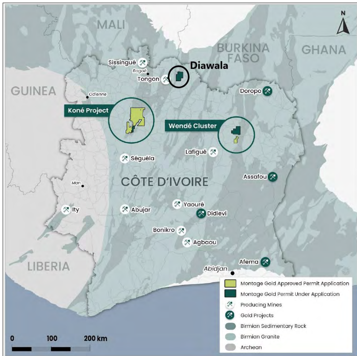
Figure 2.7: Montage regional exploration projects, Cote d'Ivoire
