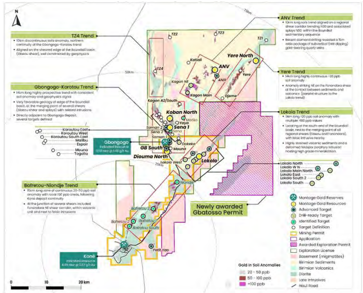
Figure 2.6: Montage – permitted areas and key gold deposits and targets
