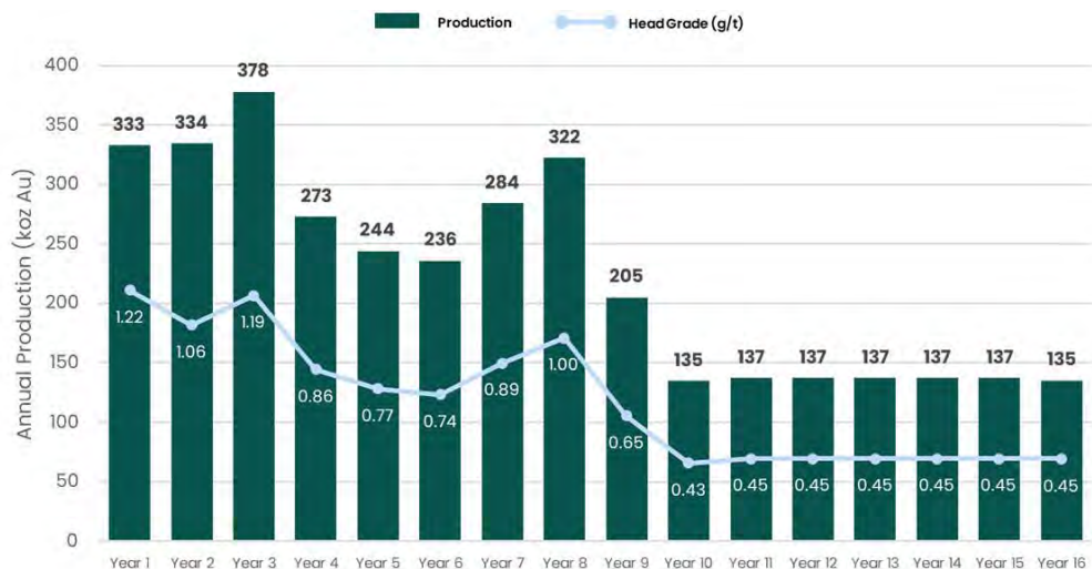
Figure 7. Production profile of the Koné Project
