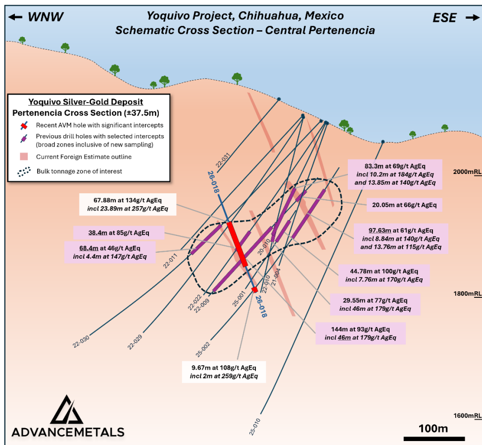
Figure 3. Schematic cross section (±37.5m, looking north-northeast) through the central portion of Pertenencia showing previous drilling 4 and highlighting selected broad intervals (purple) defined following the recent resampling program 1 . An approximate outline of the existing Foreign Estimate 3,4 , along with significant down hole intersections for new oblique drill hole YQ-26018 (red bars) are also shown.
