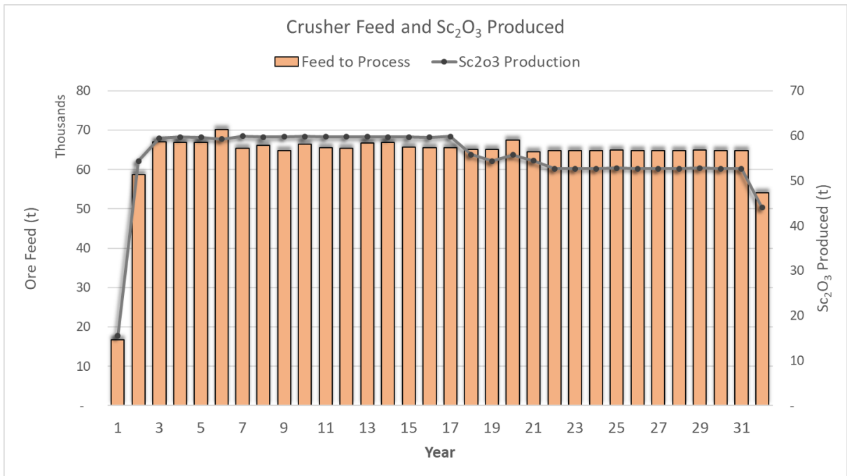
Figure 4: Life of Mine (LOM) Ore Feed and Sc 2 O 3 Production
