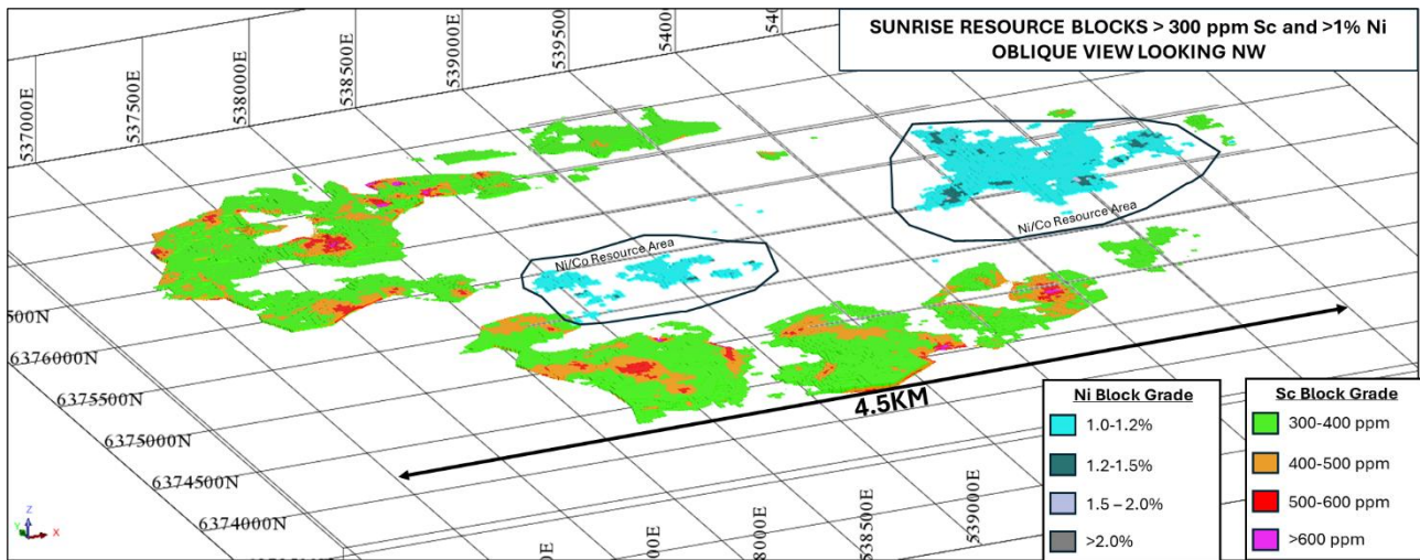
Figure 6: – Cross section of Syerston MRE including proximity to the Sunrise Ni/Co deposit
