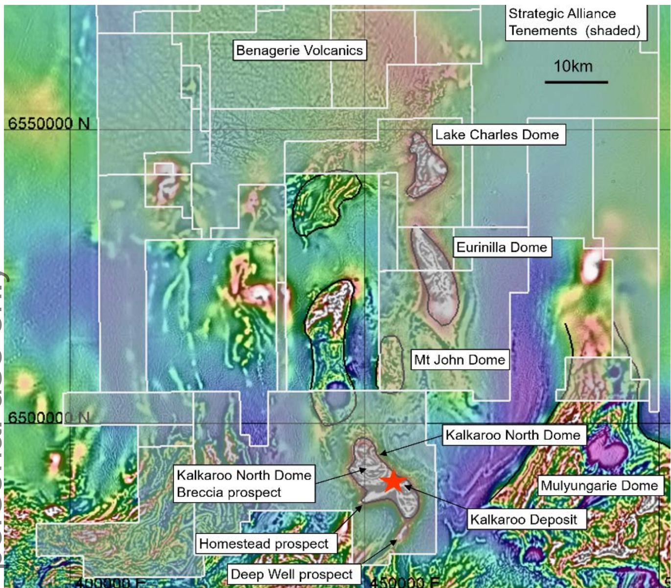
Figure 1 Aeromagnetic image showing locations of the prospects mentioned in the text in relation to the Kalkaroo deposit, in the Curnamona Province of northeastern South Australia.
