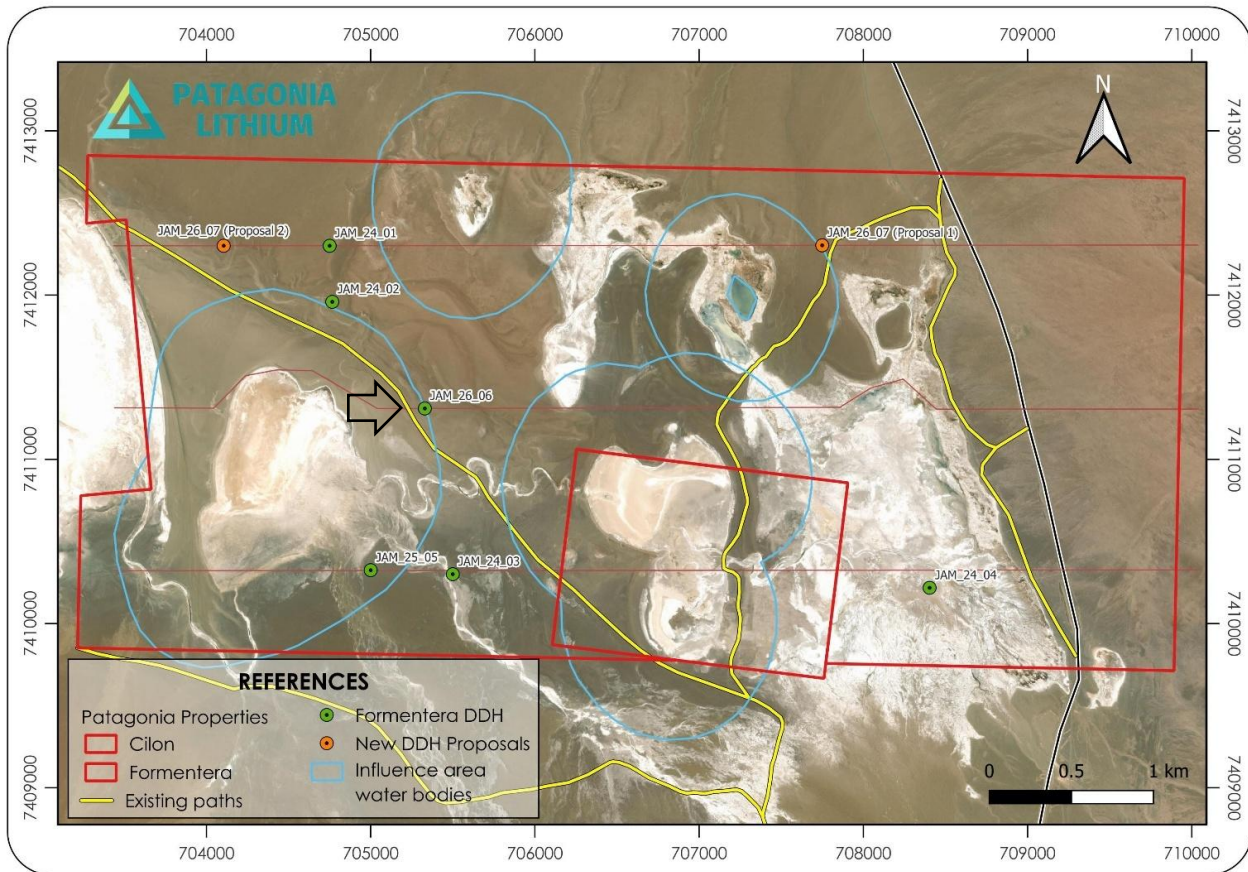
Figure 4. Location map showing well JAM 26-06 location with black arrow. Note it is only 500m from JAM 24-02. Blue lines are 500m boundaries from lagoons or brine filled depressions.
