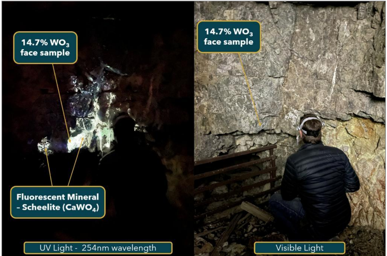
Figure 1; Photo showing LKGB0005 high grade face sample returning 14.7% WO_3 collected from the Linka-Conquest Pit and fluorescent scheelite under UV light.
