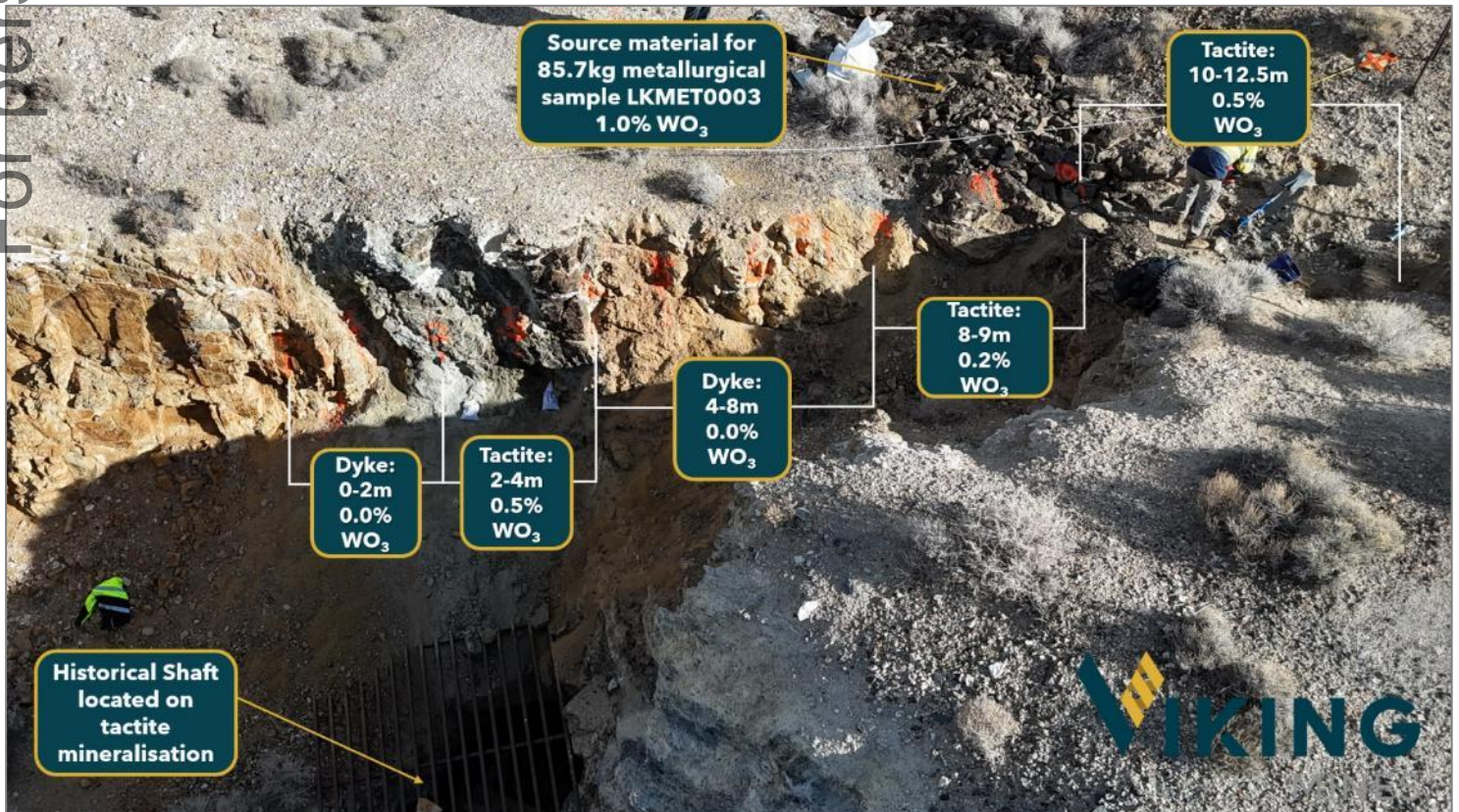
Figure 2; Photo showing LKCH0003 channel sample at Linka-Conquest pit with two mineralised intervals, 2m at 0.5% WO_3 and 2.5m at 0.5% WO_3 separated by unmineralised quartz monzonite dyke.
